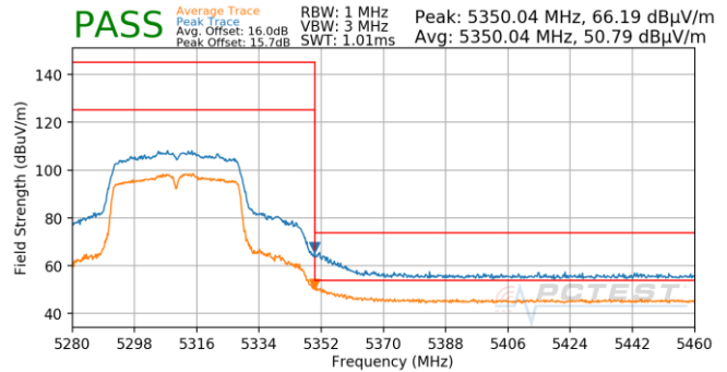
Plot 7-851. Antenna 4b (Pk & Avg, Ch.62, 802.11n, MCS3)
