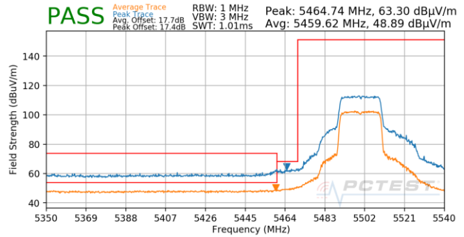
Plot 7-817. Antenna 4b (Pk & Avg, Ch.100, 802.11ax(SU), MCS3)
