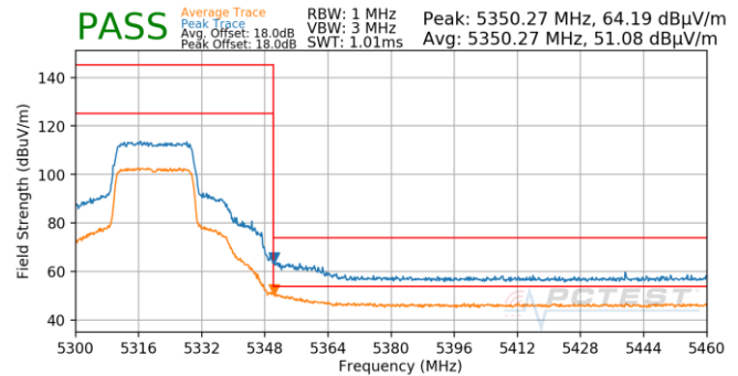
Plot 7-813. Antenna 4b (Pk & Avg, Ch.64, 802.11ax(SU), MCS0)
