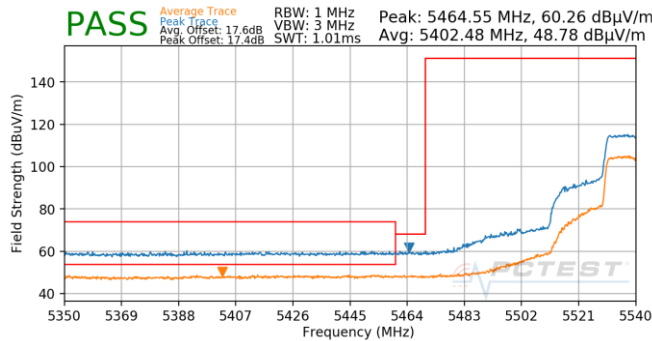
Plot 7-822. Antenna 4b (Pk & Avg, Ch.108, 802.11ax(SU), MCS3)
