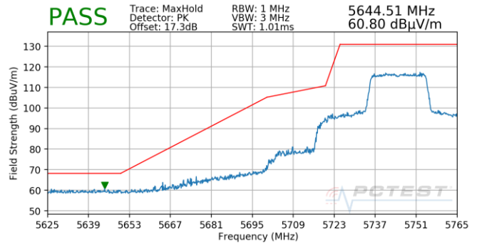
Plot 7-835. Antenna 4b (Pk, Ch.149, 802.11ax(SU), MCS0)
