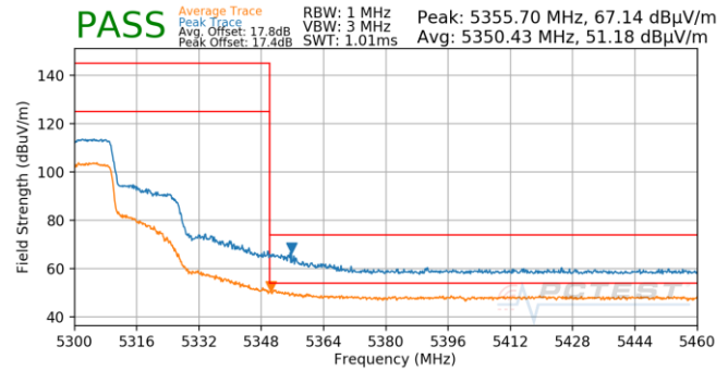
Plot 7-811. Antenna 4b (Pk & Avg, Ch.60, 802.11ax(SU), MCS3)
