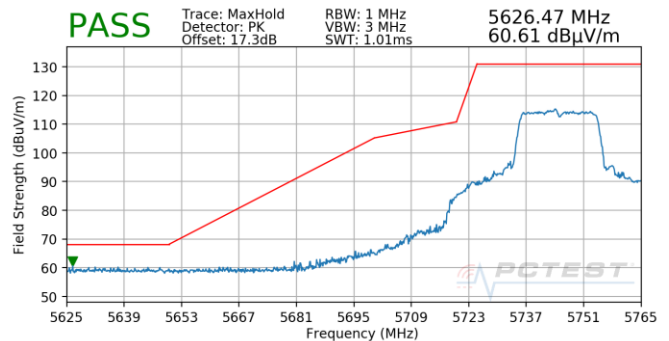
Plot 7-837. Antenna 4b (Pk, Ch.149, 802.11ax(SU), MCS11)
