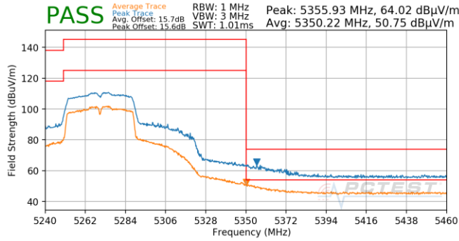
Plot 7-847. Antenna 4b (Pk & Avg, Ch.54, 802.11n, MCS0)
