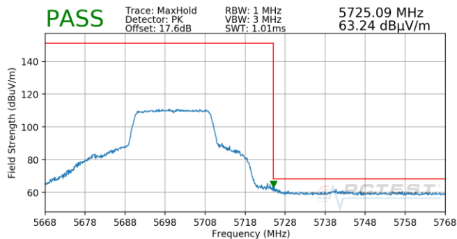
Plot 7-833. Antenna 4b (Pk, Ch.140, 802.11ax(SU), MCS3)
