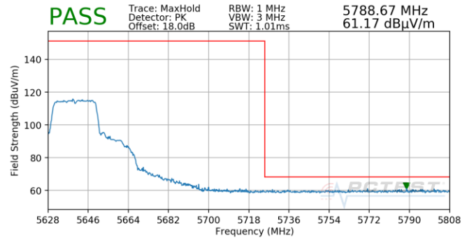
Plot 7-825. (FCC Only) Antenna 4b (Pk & Avg, Ch.128, 802.11ax(SU), MCS11)
