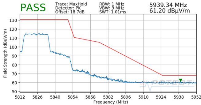
Plot 7-839. Antenna 4b (Pk, Ch.165, 802.11ax(SU), MCS3)
