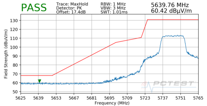
Plot 7-798. Antenna 4b (Pk, Ch.149, 802.11n, MCS5)
