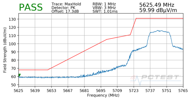
Plot 7-796. Antenna 4b (Pk, Ch.149, 802.11n, MCS0)
