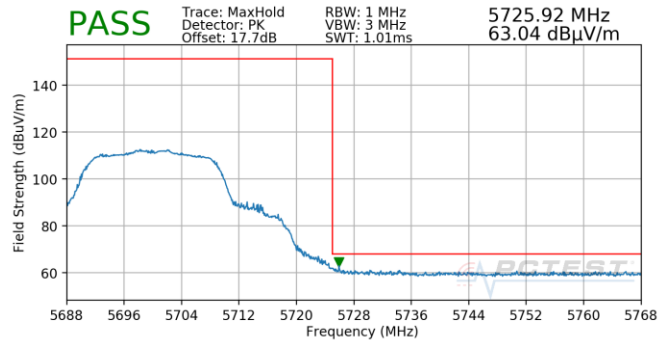
Plot 7-793. Antenna 4b (Pk, Ch.140, 802.11n, MCS0)
