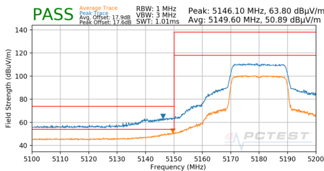
Plot 7-803. Antenna 4b (Pk & Avg, Ch.36, 802.11ax(SU), MCS3)
