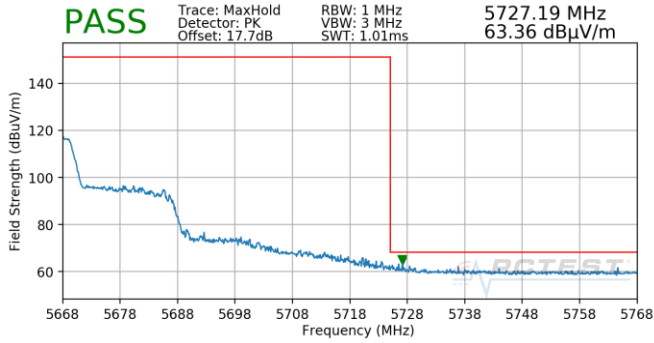
Plot 7-826. Antenna 4b (Pk, Ch.132, 802.11ax(SU), MCS0)
