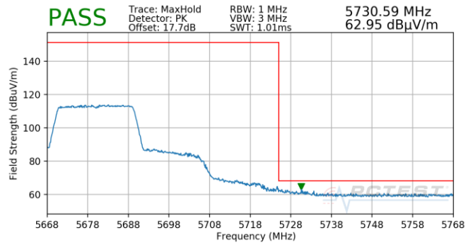
Plot 7-830. Antenna 4b (Pk, Ch.136, 802.11ax(SU), MCS3)
