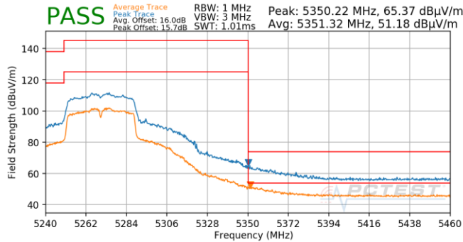
Plot 7-848. Antenna 4b (Pk & Avg, Ch.54, 802.11n, MCS3)
