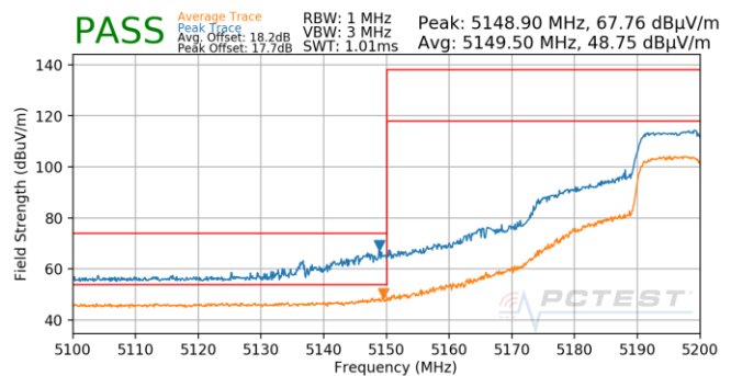
Plot 7-807. Antenna 4b (Pk & Avg, Ch.40, 802.11ax(SU), MCS11)
