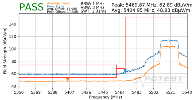
Plot 7-821. Antenna 4b (Pk & Avg, Ch.104, 802.11ax(SU), MCS11)
