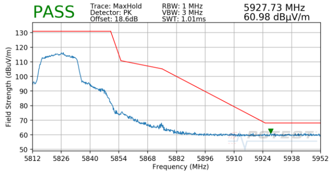
Plot 7-800. Antenna 4b (Pk, Ch.165, 802.11n, MCS3)
