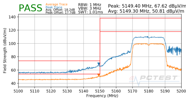
Plot 7-804. Antenna 4b (Pk & Avg, Ch.36, 802.11ax(SU), MCS11)
