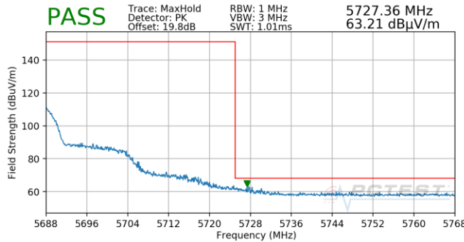
Plot 7-790. Antenna 4b (Pk, Ch.136, 802.11n, MCS0)
