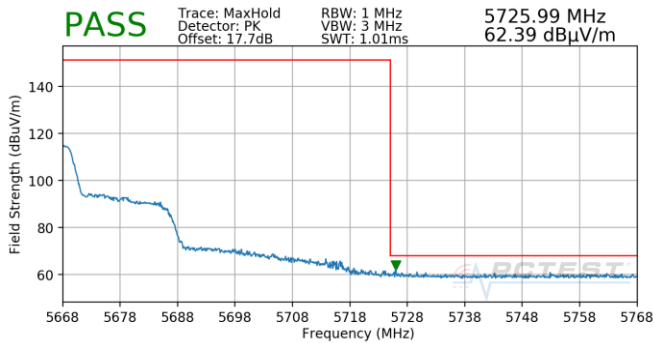
Plot 7-827. Antenna 4b (Pk, Ch.132, 802.11ax(SU), MCS3)
