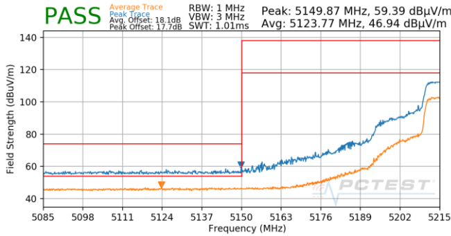
Plot 7-808. Antenna 4b (Pk & Avg, Ch.44, 802.11ax(SU), MCS11)
