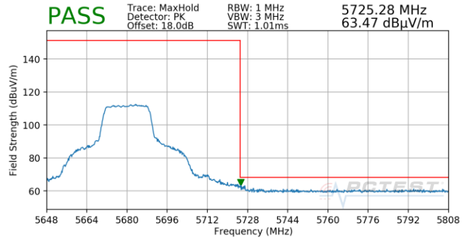
Plot 7-792. Antenna 4b (Pk, Ch.136, 802.11n, MCS5)
