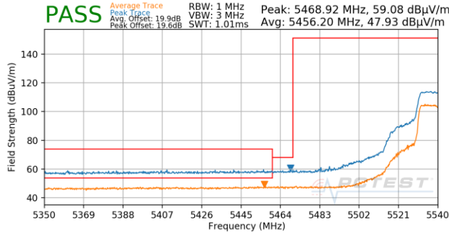
Plot 7-788. Antenna 4b (Pk & Avg, Ch.108, 802.11n, MCS5)
