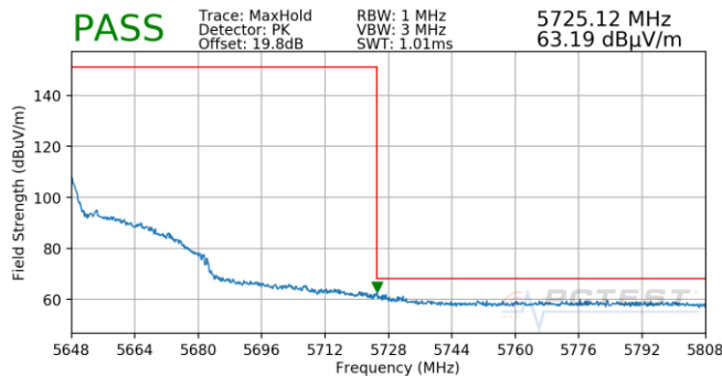
Plot 7-861. (FCC Only) Antenna 4b (Pk, Ch.126, 802.11n, MCS3)
