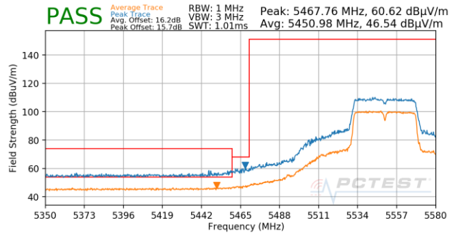
Plot 7-858. Antenna 4b (Pk & Avg, Ch.110, 802.11n, MCS5)
