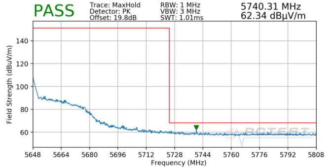
Plot 7-862. (FCC Only) Antenna 4b (Pk, Ch.126, 802.11n, MCS5)
