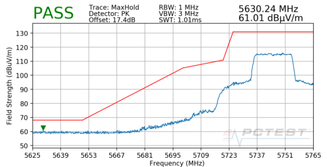
Plot 7-836. Antenna 4b (Pk, Ch.149, 802.11ax(SU), MCS3)
