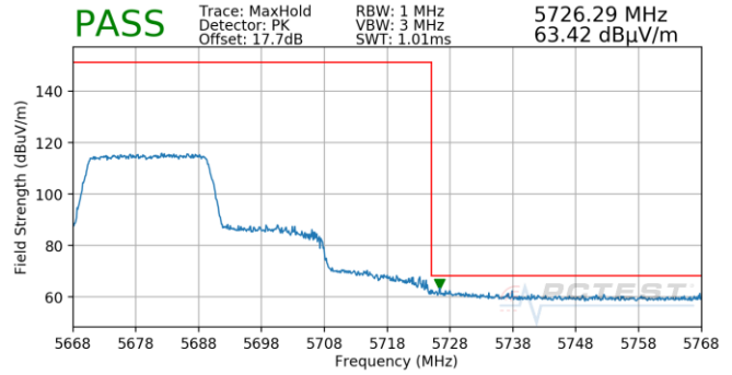
Plot 7-829. Antenna 4b (Pk, Ch.136, 802.11ax(SU), MCS0)
