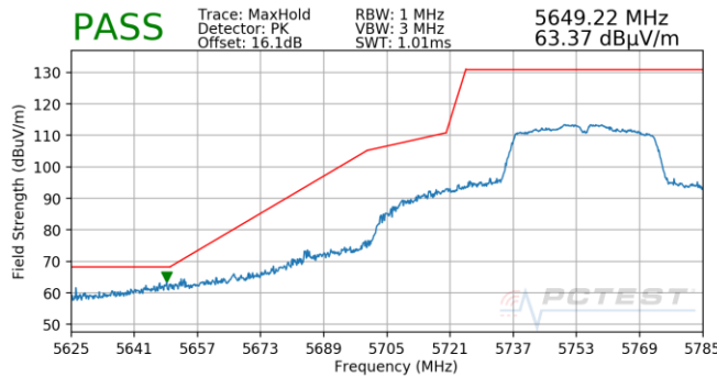
Plot 7-866. Antenna 4b (Pk, Ch.151, 802.11n, MCS0)
