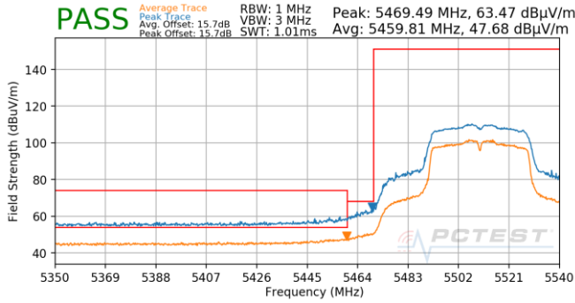
Plot 7-853. Antenna 4b (Pk & Avg, Ch.102, 802.11n, MCS0)
