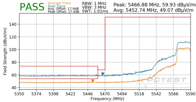
Plot 7-859. (FCC Only) Antenna 4b (Pk, Ch.118, 802.11n, MCS5)
