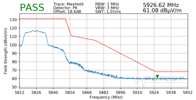
Plot 7-799. Antenna 4b (Pk, Ch.165, 802.11n, MCS0)
