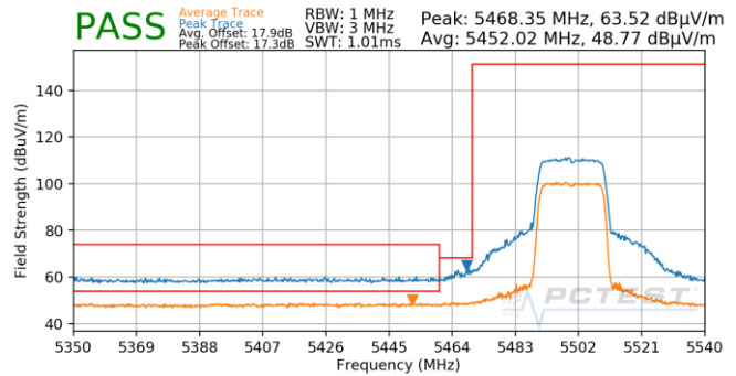
Plot 7-818. Antenna 4b (Pk & Avg, Ch.100, 802.11ax(SU), MCS11)
