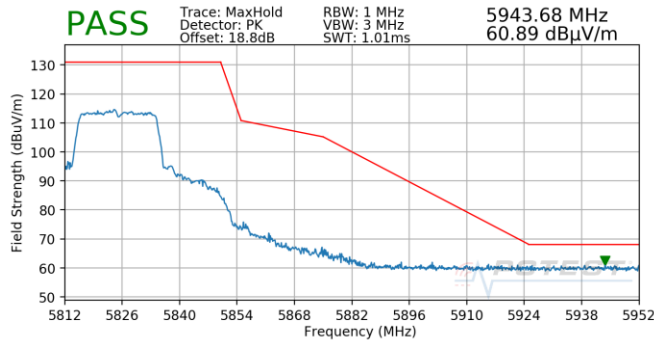
Plot 7-840. Antenna 4b (Pk, Ch.165, 802.11ax(SU), MCS11)
