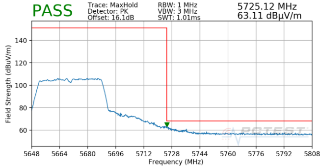
Plot 7-865. Antenna 4b (Pk, Ch.134, 802.11n, MCS5)
