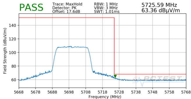
Plot 7-834. Antenna 4b (Pk, Ch.140, 802.11ax(SU), MCS11)
