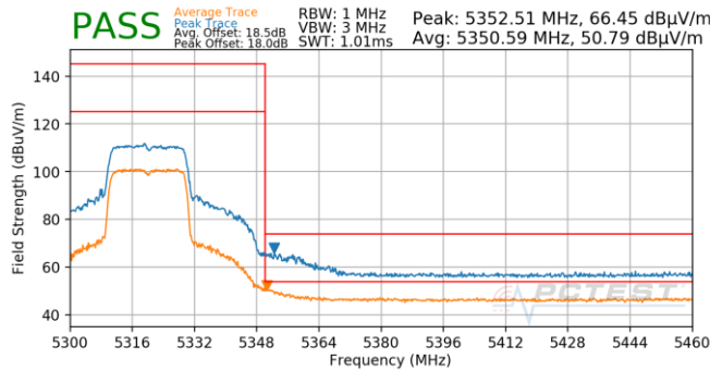
Plot 7-815. Antenna 4b (Pk & Avg, Ch.64, 802.11ax(SU), MCS11)
