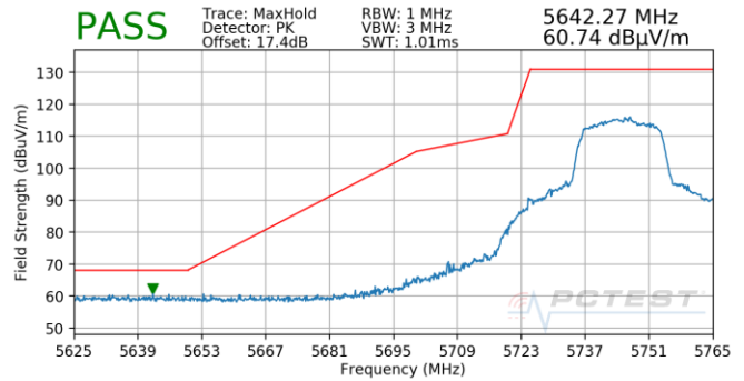
Plot 7-797. Antenna 4b (Pk, Ch.149, 802.11n, MCS3)
