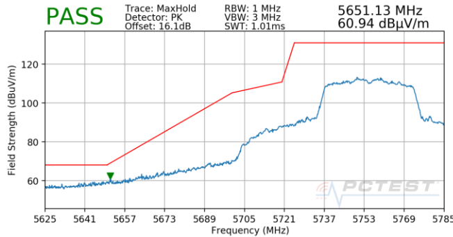
Plot 7-867. Antenna 4b (Pk, Ch.151, 802.11n, MCS3)
