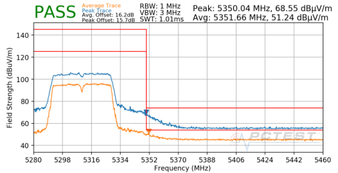
Plot 7-852. Antenna 4b (Pk & Avg, Ch.62, 802.11n, MCS5)
