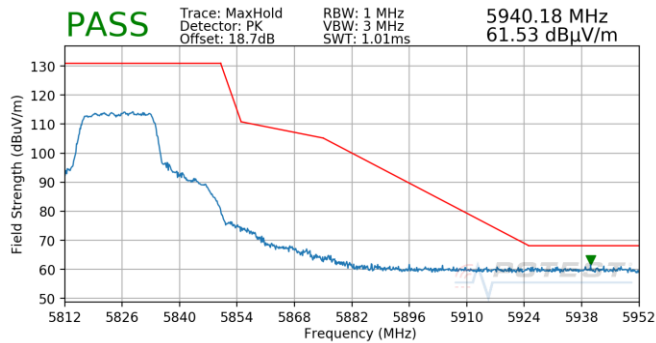
Plot 7-801. Antenna 4b (Pk, Ch.165, 802.11n, MCS5)
