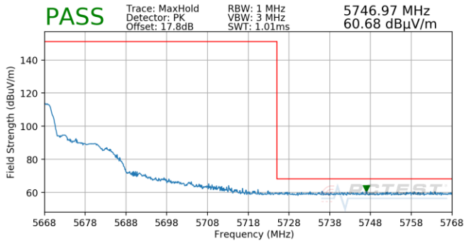
Plot 7-828. Antenna 4b (Pk, Ch.132, 802.11ax(SU), MCS11)
