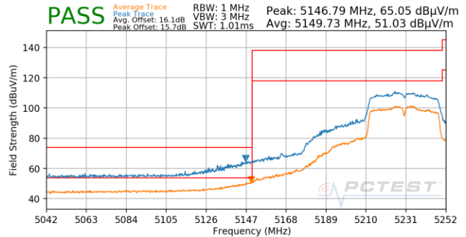
Plot 7-845. Antenna 4b (Pk & Avg, Ch.46, 802.11n, MCS3)
