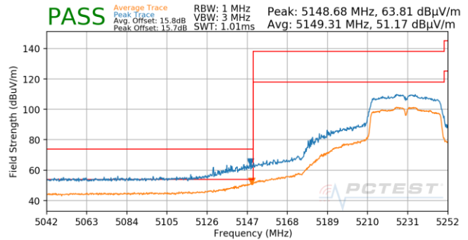
Plot 7-844. Antenna 4b (Pk & Avg, Ch.46, 802.11n, MCS0)
