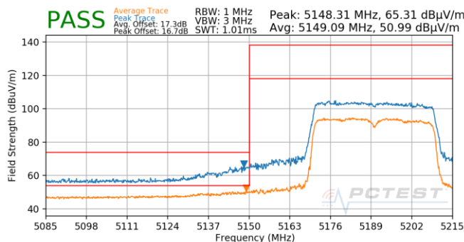
Plot 7-874. Antenna 4b (Pk & Avg, Ch.38, 80.11ax(SU), MCS11)
