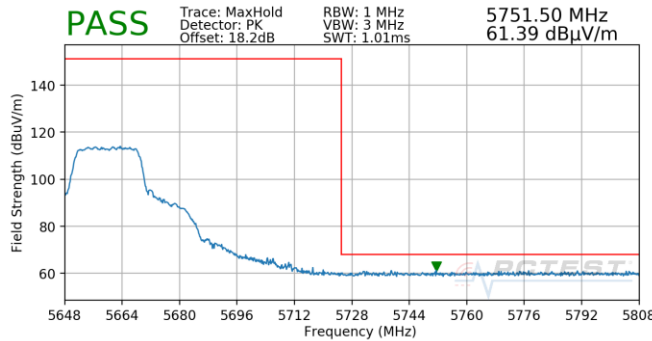
Plot 7-789. Antenna 4b (Pk, Ch.132, 802.11n, MCS5)
