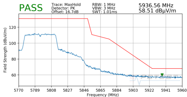
Plot 7-871. Antenna 4b (Pk, Ch.159, 802.11n, MCS5)
