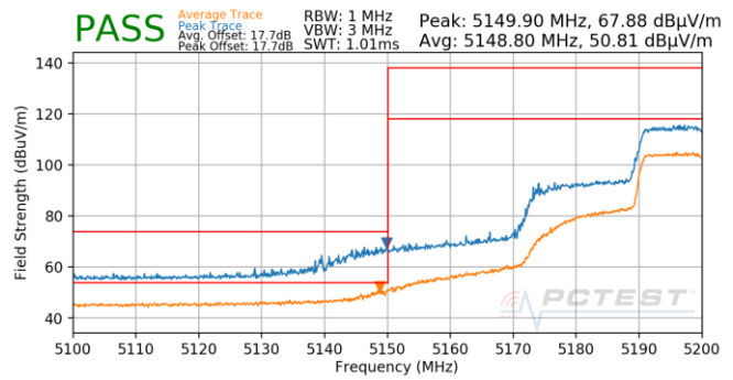
Plot 7-805. Antenna 4b (Pk & Avg, Ch.40, 802.11ax(SU), MCS0)
