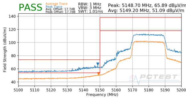
Plot 7-802. Antenna 4b (Pk & Avg, Ch.36, 802.11ax(SU), MCS0)
