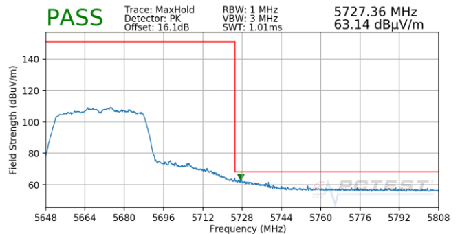
Plot 7-864. Antenna 4b (Pk, Ch.134, 802.11n, MCS3)
