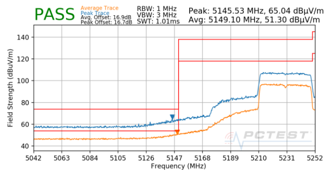
Plot 7-876. Antenna 4b (Pk & Avg, Ch.46, 80.11ax(SU), MCS3)
