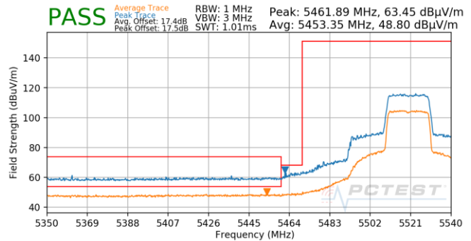
Plot 7-819. Antenna 4b (Pk & Avg, Ch.104, 802.11ax(SU), MCS0)
