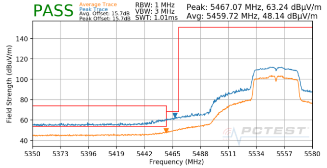
Plot 7-856. Antenna 4b (Pk & Avg, Ch.110, 802.11n, MCS0)
