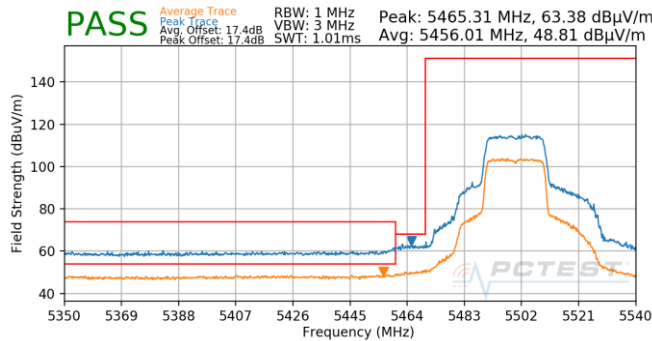
Plot 7-816. Antenna 4b (Pk & Avg, Ch.100, 802.11ax(SU), MCS0)
