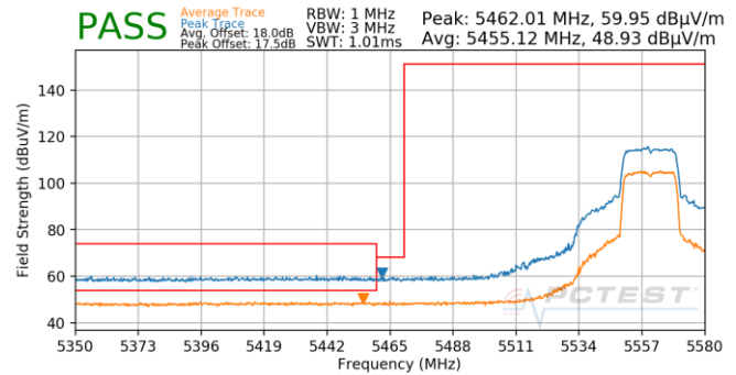
Plot 7-824. Antenna 4b (Pk & Avg, Ch.112, 802.11ax(SU), MCS11)
