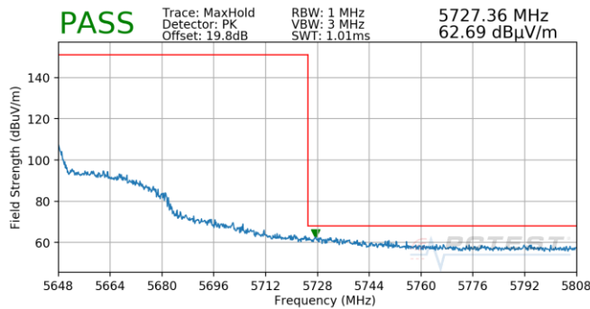
Plot 7-860. (FCC Only) Antenna 4b (Pk, Ch.126, 802.11n, MCS0)
