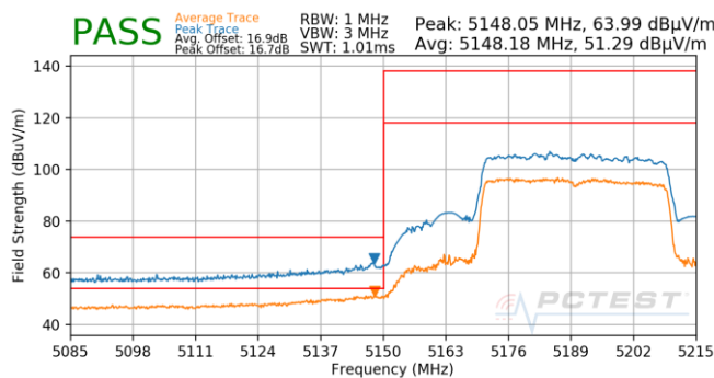
Plot 7-873. Antenna 4b (Pk & Avg, Ch.38, 80.11ax(SU), MCS3)
