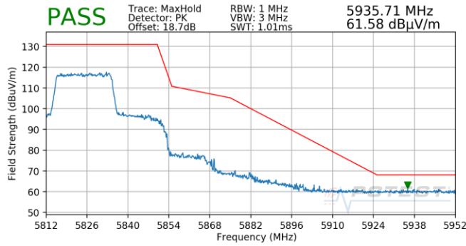
Plot 7-838. Antenna 4b (Pk, Ch.165, 802.11ax(SU), MCS0)
