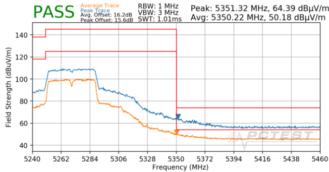
Plot 7-849. Antenna 4b (Pk & Avg, Ch.54, 802.11n, MCS5)
