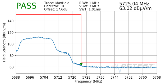
Plot 7-794. Antenna 4b (Pk, Ch.140, 802.11n, MCS3)
