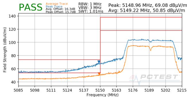
Plot 7-843. Antenna 4b (Pk & Avg, Ch.38, 802.11n, MCS5)
