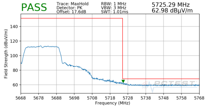
Plot 7-831. Antenna 4b (Pk, Ch.136, 802.11ax(SU), MCS11)
