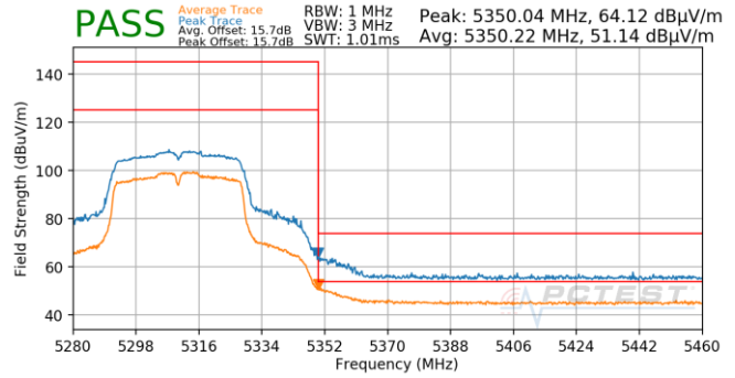
Plot 7-850. Antenna 4b (Pk & Avg, Ch.62, 802.11n, MCS0)
