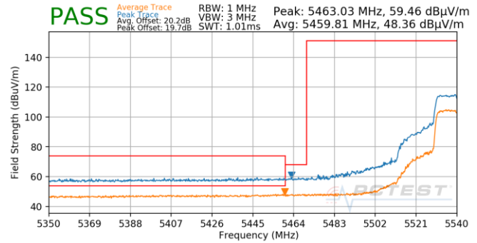
Plot 7-823. Antenna 4b (Pk & Avg, Ch.108, 802.11ax(SU), MCS11)
