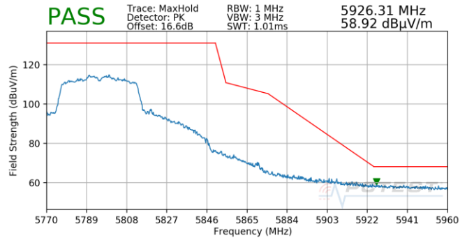
Plot 7-870. Antenna 4b (Pk, Ch.159, 802.11n, MCS3)
