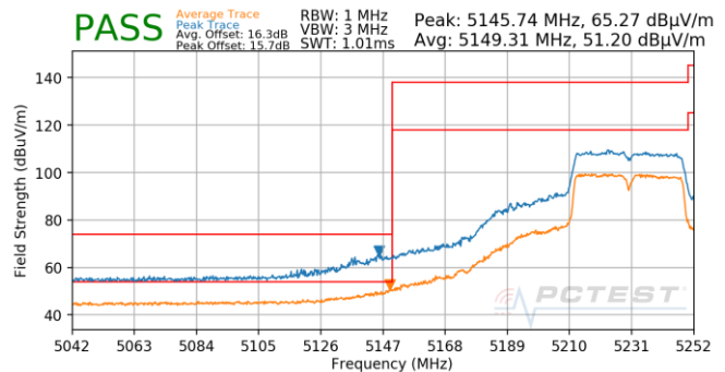
Plot 7-846. Antenna 4b (Pk & Avg, Ch.46, 802.11n, MCS5)
