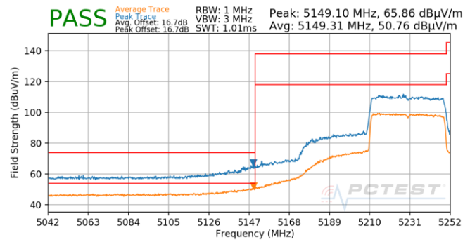
Plot 7-875. Antenna 4b (Pk & Avg, Ch.46, 80.11ax(SU), MCS0)
