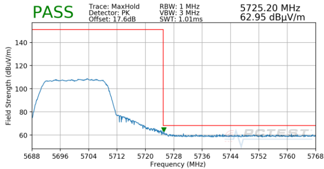
Plot 7-795. Antenna 4b (Pk, Ch.140, 802.11n, MCS5)
