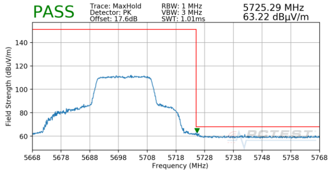
Plot 7-832. Antenna 4b (Pk, Ch.140, 802.11ax(SU), MCS0)
