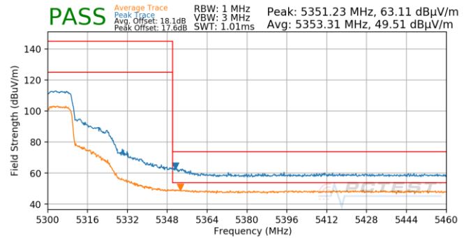
Plot 7-812. Antenna 4b (Pk & Avg, Ch.60, 802.11ax(SU), MCS11)
