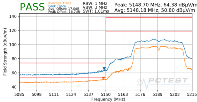
Plot 7-842. Antenna 4b (Pk & Avg, Ch.38, 802.11n, MCS3)
