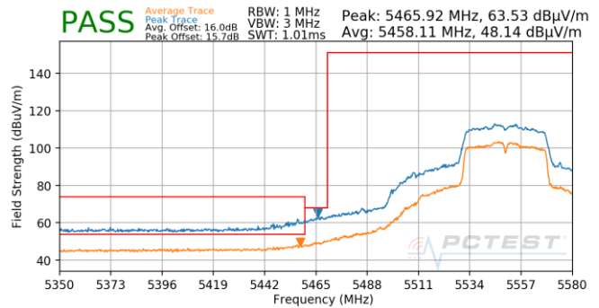
Plot 7-857. Antenna 4b (Pk & Avg, Ch.110, 802.11n, MCS3)
