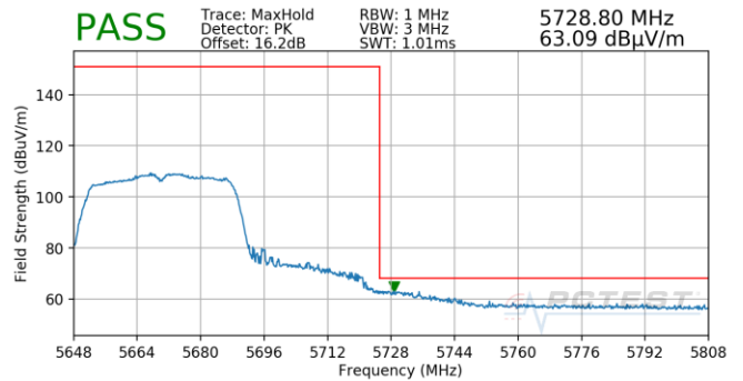
Plot 7-863. Antenna 4b (Pk, Ch.134, 802.11n, MCS0)
