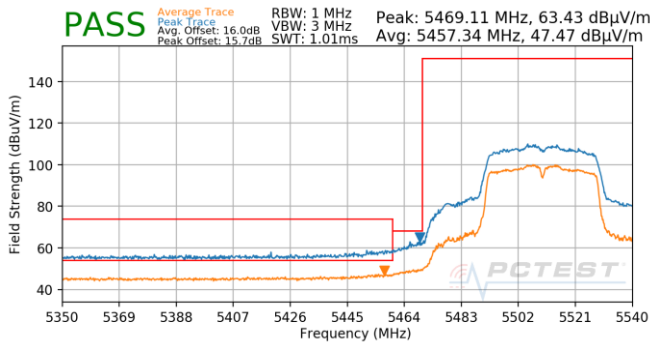
Plot 7-854. Antenna 4b (Pk & Avg, Ch.102, 802.11n, MCS3)
