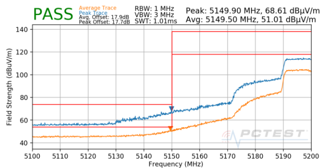
Plot 7-806. Antenna 4b (Pk & Avg, Ch.40, 802.11ax(SU), MCS3)
