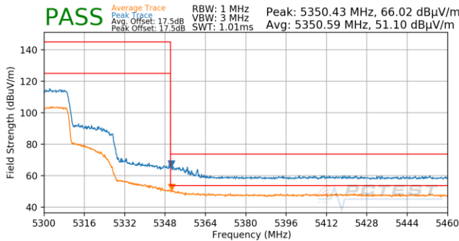
Plot 7-810. Antenna 4b (Pk & Avg, Ch.60, 802.11ax(SU), MCS0)
