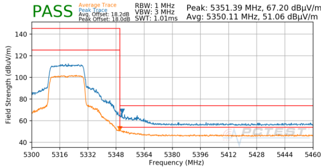
Plot 7-814. Antenna 4b (Pk & Avg, Ch.64, 802.11ax(SU), MCS3)
