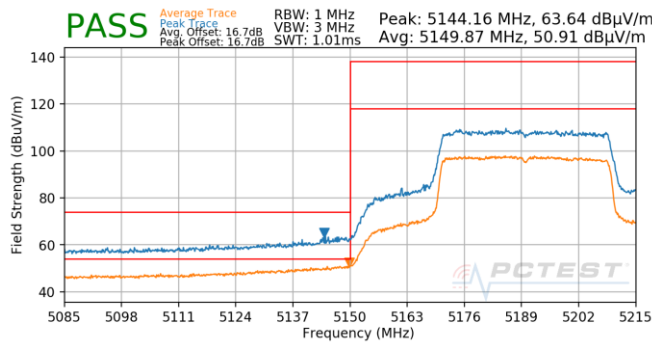
Plot 7-872. Antenna 4b (Pk & Avg, Ch.38, 80.11ax(SU), MCS0)
