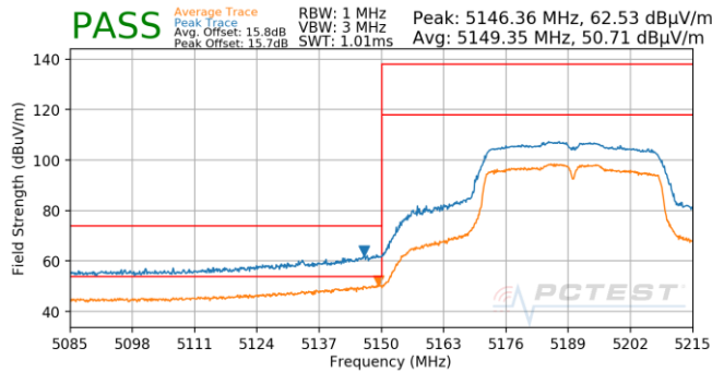
Plot 7-841. Antenna 4b (Pk & Avg, Ch.38, 802.11n, MCS0)
