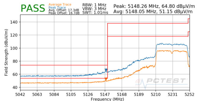
Plot 7-877. Antenna 4b (Pk & Avg, Ch.46, 80.11ax(SU), MCS11)
