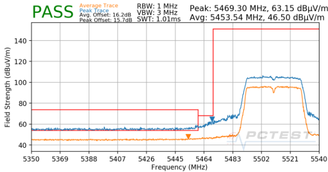
Plot 7-855. Antenna 4b (Pk & Avg, Ch.102, 802.11n, MCS5)
