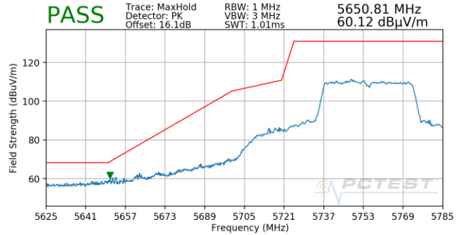
Plot 7-868. Antenna 4b (Pk, Ch.151, 802.11n, MCS5)
