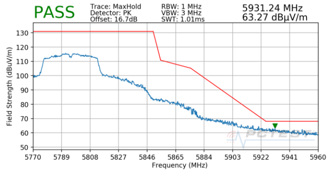
Plot 7-869. Antenna 4b (Pk, Ch.159, 802.11n, MCS0)
