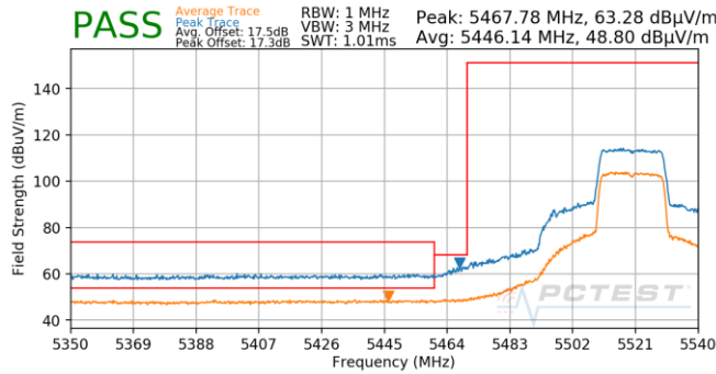
Plot 7-820. Antenna 4b (Pk & Avg, Ch.104, 802.11ax(SU), MCS3)
