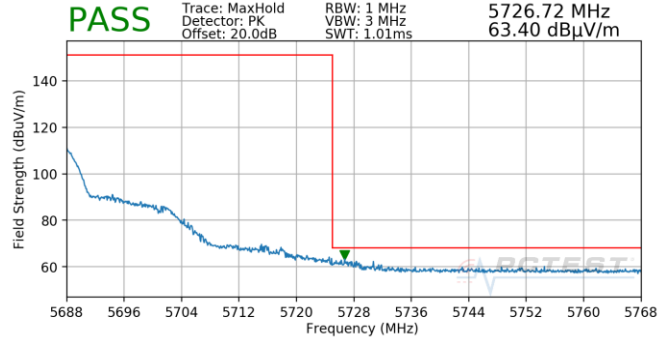
Plot 7-791. Antenna 4b (Pk, Ch.136, 802.11n, MCS3)
