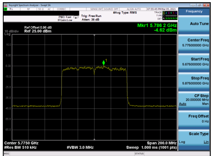
Plot 7-306. PSD Antenna 4b (80MHz BW 802.11ax(SU) – Ch. 155, MCS11)
