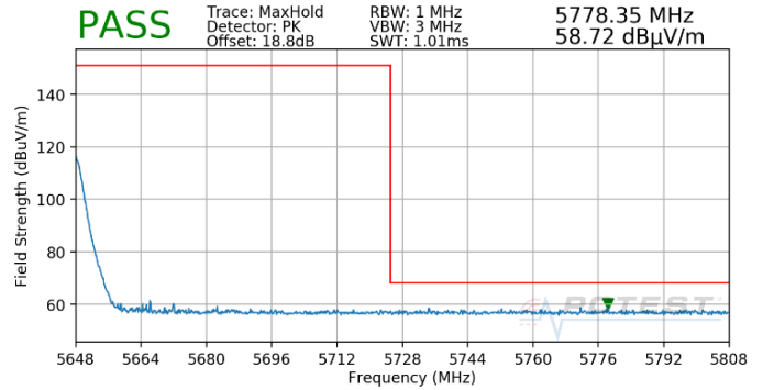
Plot 7-524. (FCC Only) Antenna 4b (Pk, RU26, Index 36, Ch.122, MCS11)
