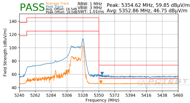
Plot 7-521. Antenna 4b (Pk & Avg, RU26, Index 36, Ch.58, MCS11)
