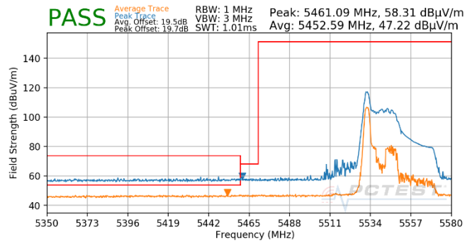
Plot 7-505. Antenna 4b (Pk & Avg, RU26, Index 0, Ch.110, MCS11)
