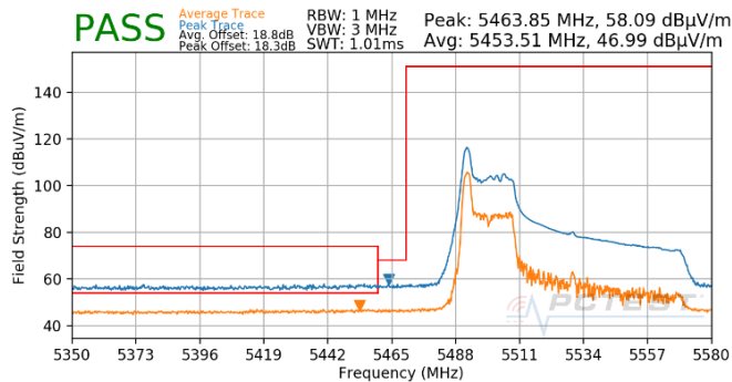
Plot 7-522. Antenna 4b (Pk & Avg, RU26, Index 0, Ch.106, MCS11)
