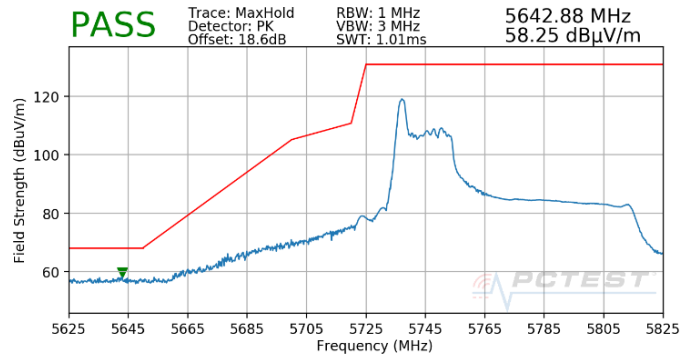
Plot 7-525. Antenna 4b (Pk, RU26, Index 0, Ch.155, MCS11)
