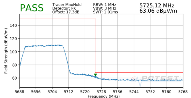
Plot 7-499. Antenna 4b (Pk, RU242, Index 61, Ch.140, MCS11)
