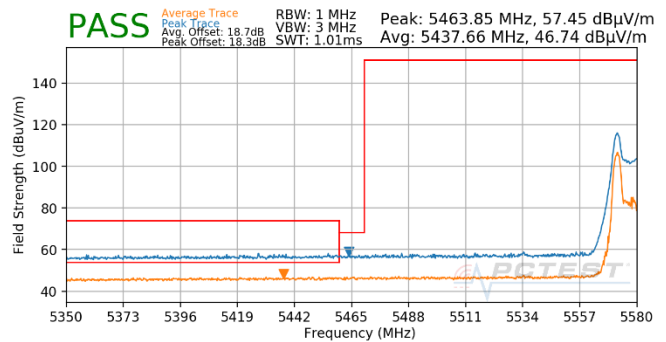
Plot 7-523. (FCC Only) Antenna 4b (Pk & Avg, RU26, Index 0, Ch.122, MCS11)
