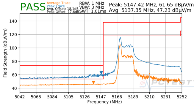
Plot 7-520. Antenna 4b (Pk & Avg, RU26, Index 0, Ch.42, MCS11)
