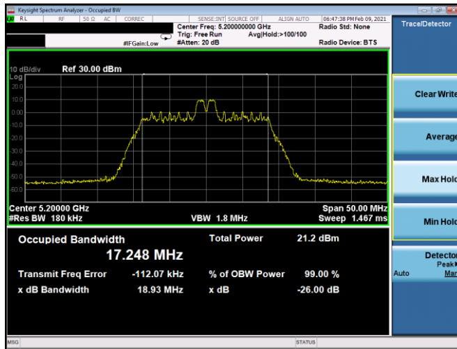
Plot 7-2. 26dB BW & 99% OBW Antenna 5b (20MHz BW 11ax Index 4 - RU26 - Ch.40)
