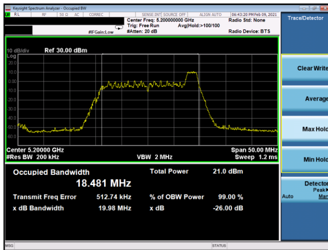
Plot 7-3. 26dB BW & 99% OBW Antenna 5b (20MHz BW 11ax Index 8- RU26 - Ch.40)
