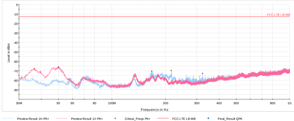
Plot 7-381. Radiated Spurious Emissions – Simultaneous Transmission 30MHz – 1GHz
