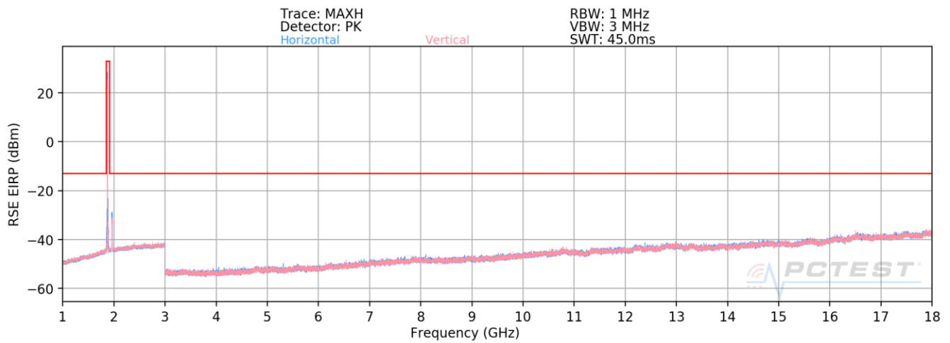
Plot 7-263. Radiated Spurious Plot (LTE Band 25/2)
