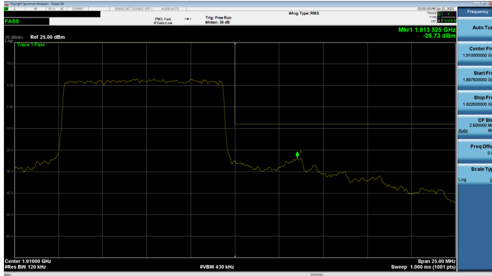
Plot 7-158. Upper Band Edge Plot (NR Band n2 – 10.0MHz DFT-s-OFDM \pi/2 BPSK - Full RB)
