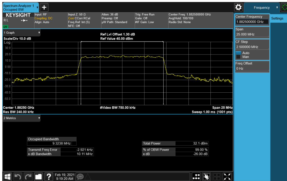
Plot 7-36. Occupied Bandwidth Plot (NR Band n25/n2 - 10.0MHz DFT-s-OFDM QPSK - Full RB)
