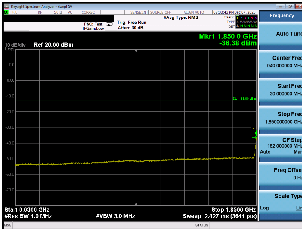
Plot 7-51. CSE (LTE Band 25/2 - 20MHz QPSK - RB Size 1, RB Offset 0 - Mid Channel)
