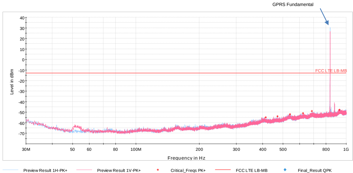
Plot 7-120. Radiated Spurious Emission below 1GHz (GPRS Cell)
