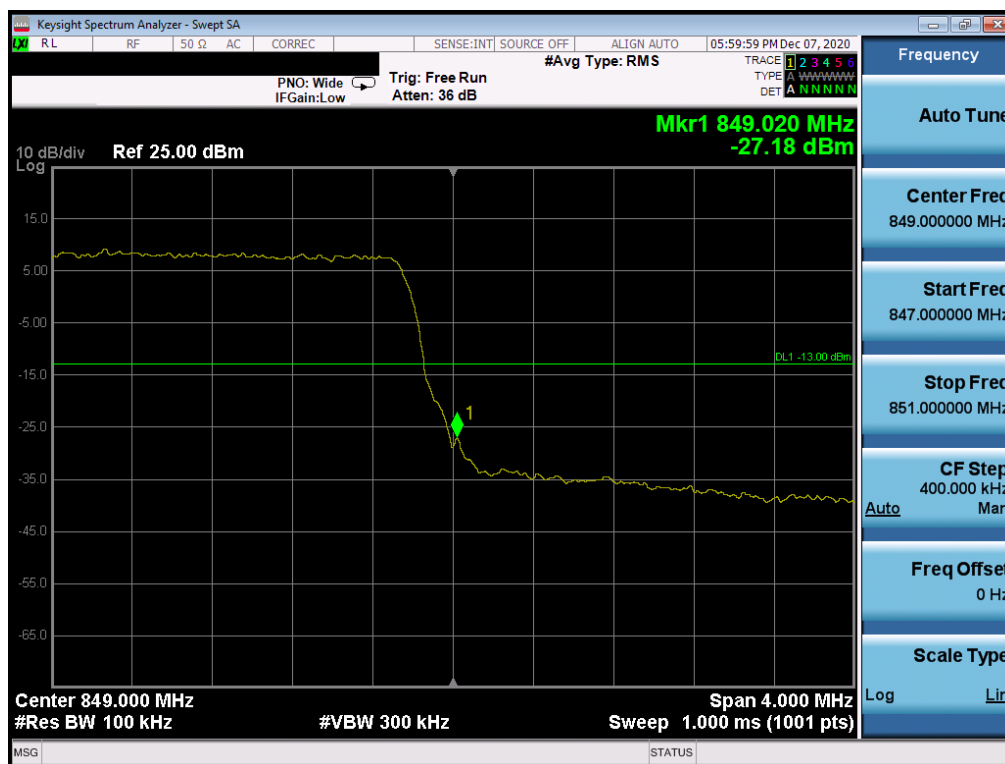
Plot 7-97. Upper Band Edge Plot (LTE Band 26 - 5MHz QPSK - Full RB Configuration)
