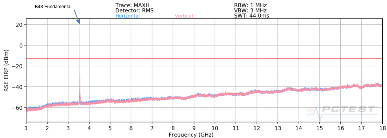
Plot 7-126. Radiated Spurious Emission 1GHz – 18GHz (NR Band n5 + Anchor LTE Band 48 – EN-DC)
