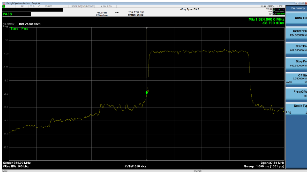
Plot 7-104. Lower Band Edge Plot (NR Band n5 DFT-s-OFDM \pi/2 BPSK– 15.0MHz - Full RB)
