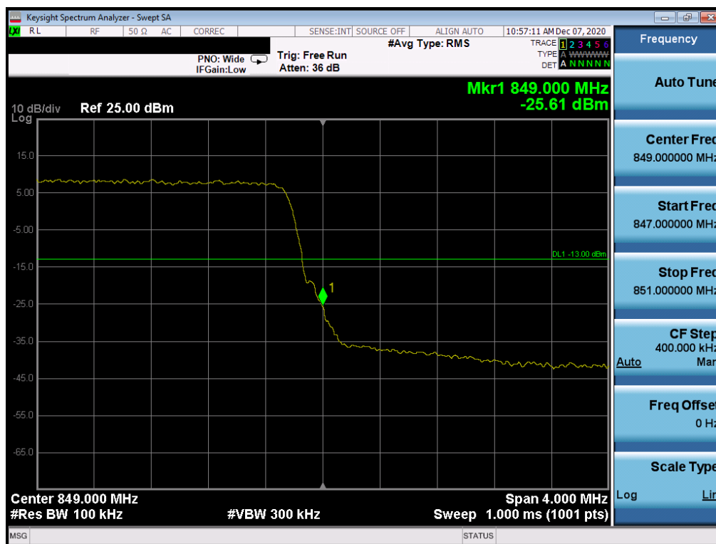
Plot 7-89. Upper Band Edge Plot (LTE Band 5 - 5MHz QPSK - Full RB Configuration)
