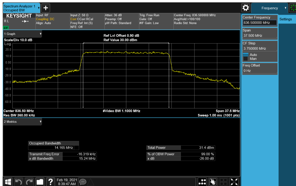
Plot 7-31. Occupied Bandwidth Plot (NR Band n5 - 15MHz CP-OFDM 16-QAM - Full RB Configuration)
