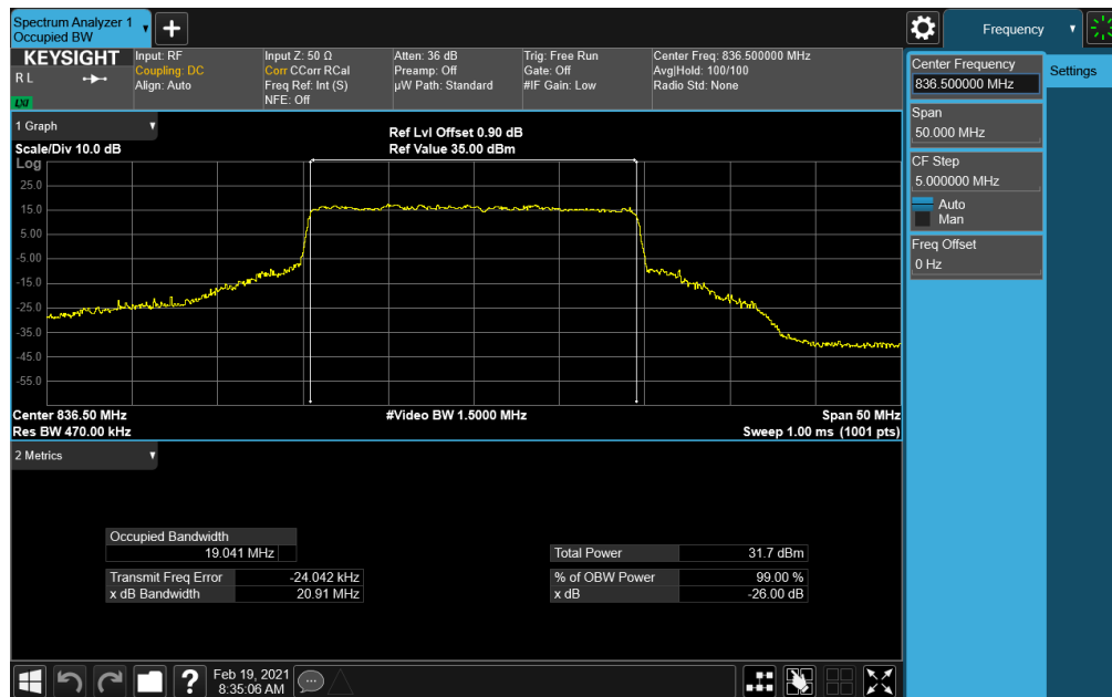
Plot 7-26. Occupied Bandwidth Plot (NR Band n5 - 20MHz CP-OFDM 16-QAM - Full RB Configuration)
