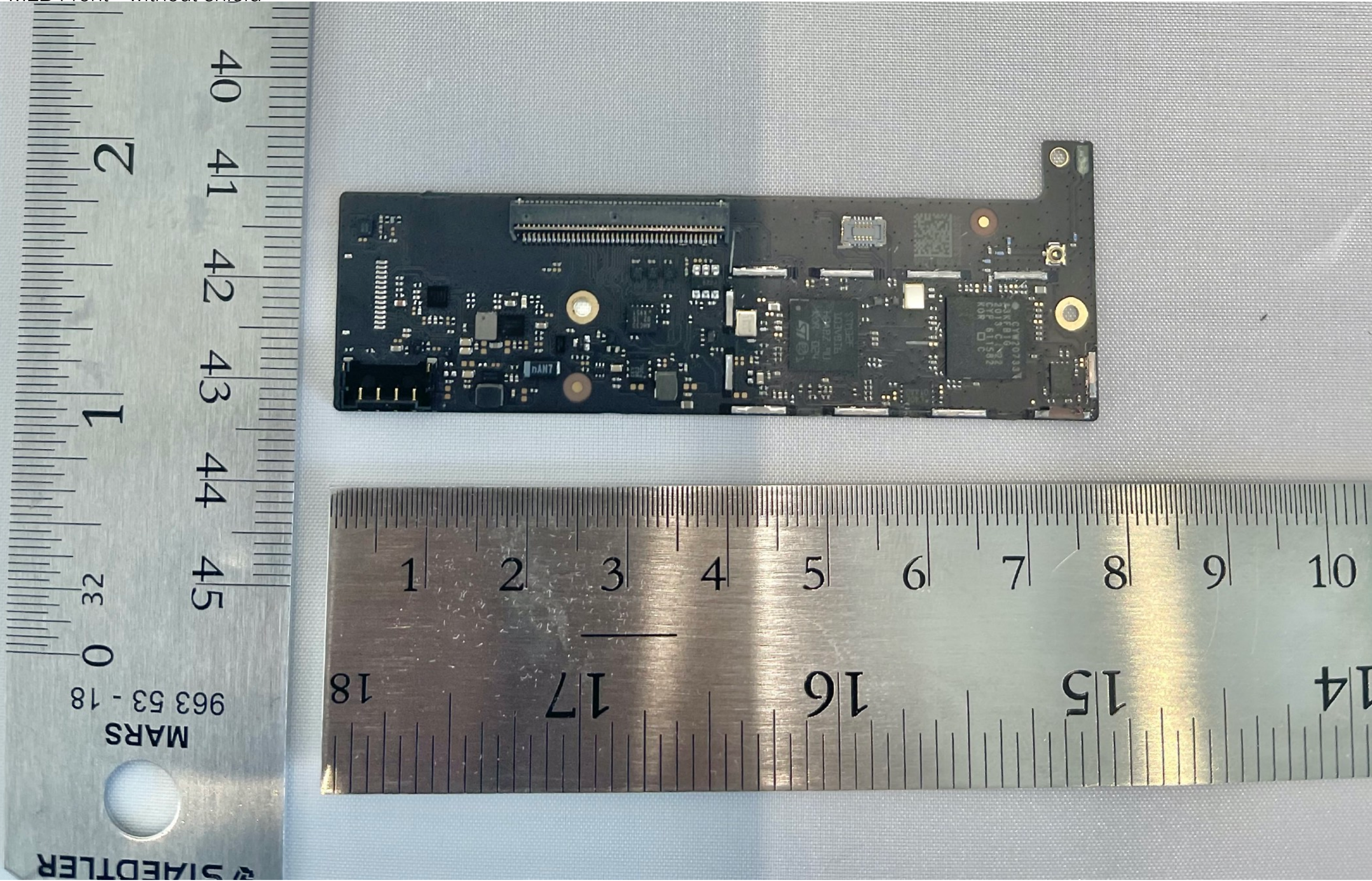
A2450 MLB Front - without shield
