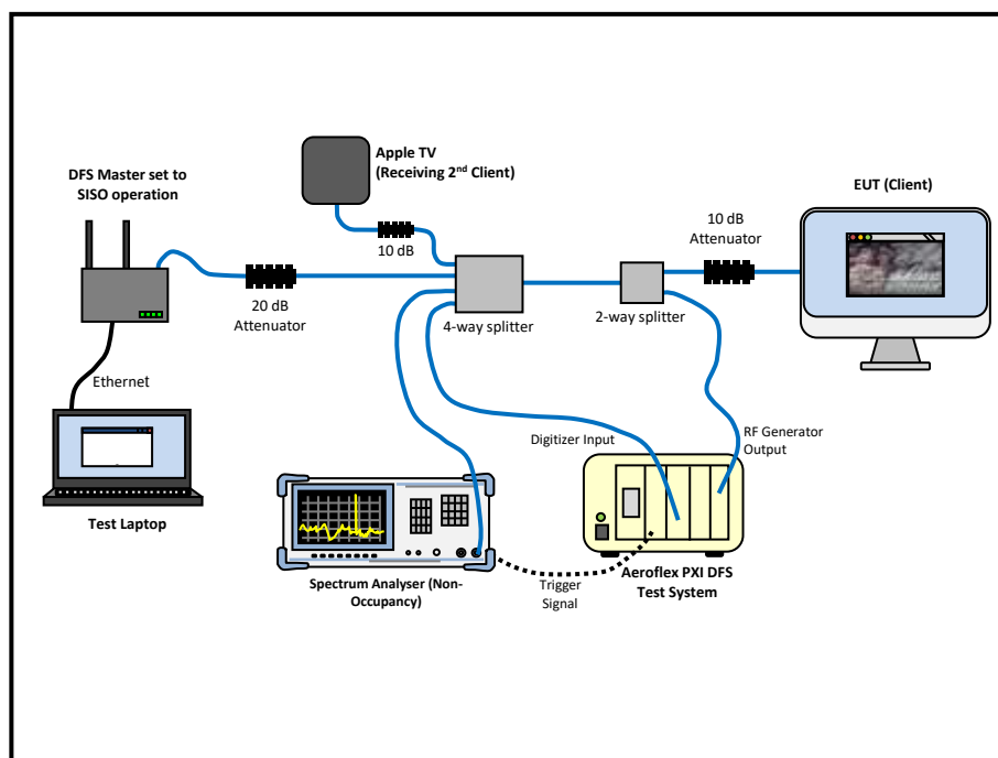
Figure 1149 - Test Equipment Setup Diagram for Client without Radar Detection with Injection at the Master – Client-to-Client Mode
