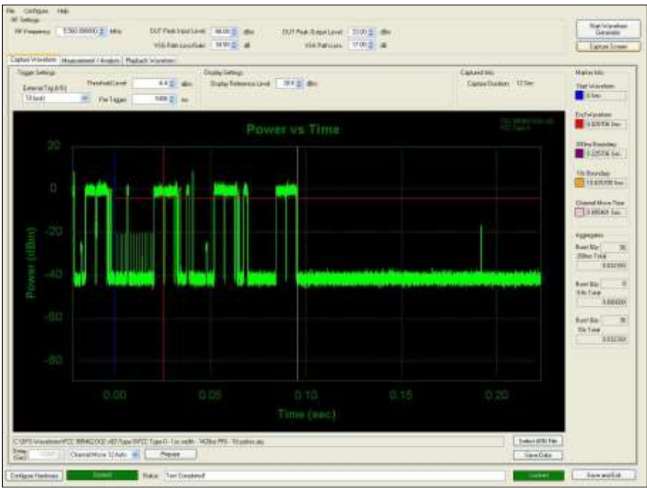
Figure 1152 - First 200 ms of Channel Shutdown Period
