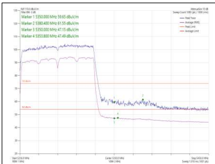
Figure 1060 - 802.11ac VHT80, Core 0 - 5290 MHz Band Edge Frequency 5350 MHz
