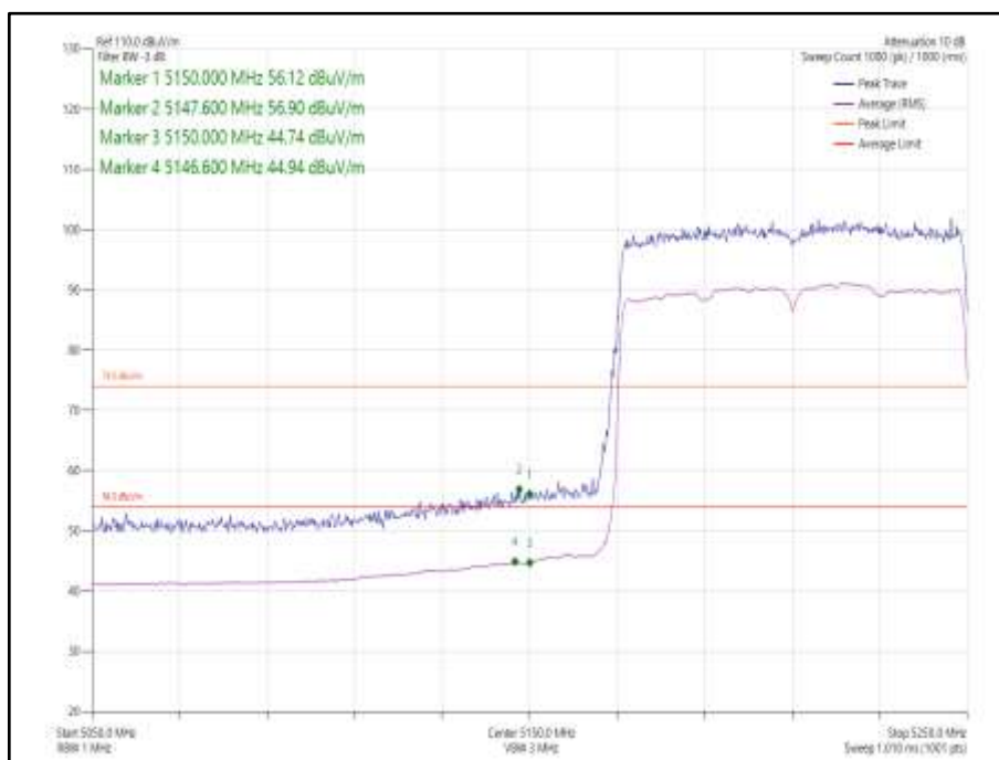
Figure 1072 - 802.11ax HE80 SDM, Cores 0-1, SU - 5210 MHz Band Edge Frequency 5150 MHz
