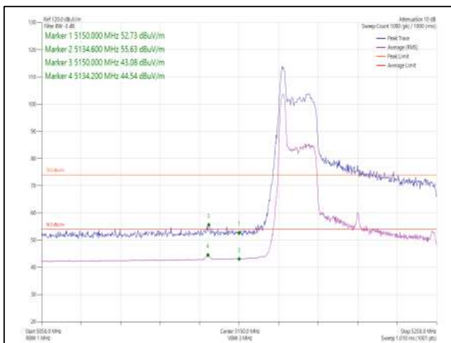
Figure 1073 - 802.11ax HE80 SDM, Cores 0-1, 26-0 - 5210 MHz Band Edge Frequency 5150 MHz
