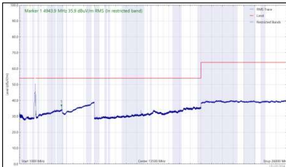
Figure 155 - 2472 MHz (CH13), 802.11b, Core 0, 1 GHz to 26 GHz, Horizontal (RMS)
