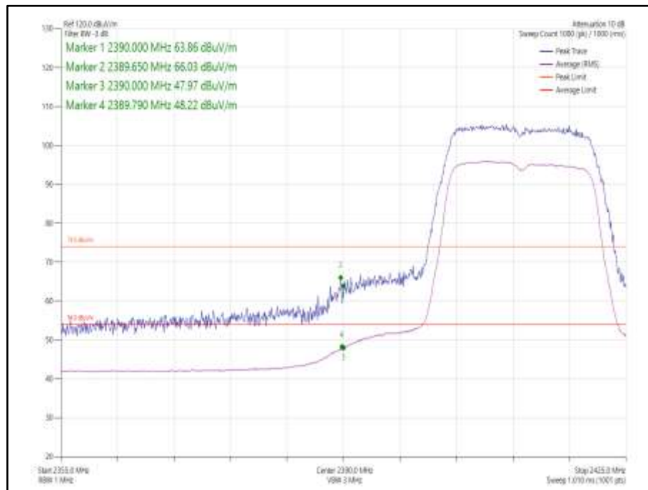
Figure 77 - 802.11n, HT20, Core 1 - 2412 MHz, Band Edge Frequency 2390 MHz
