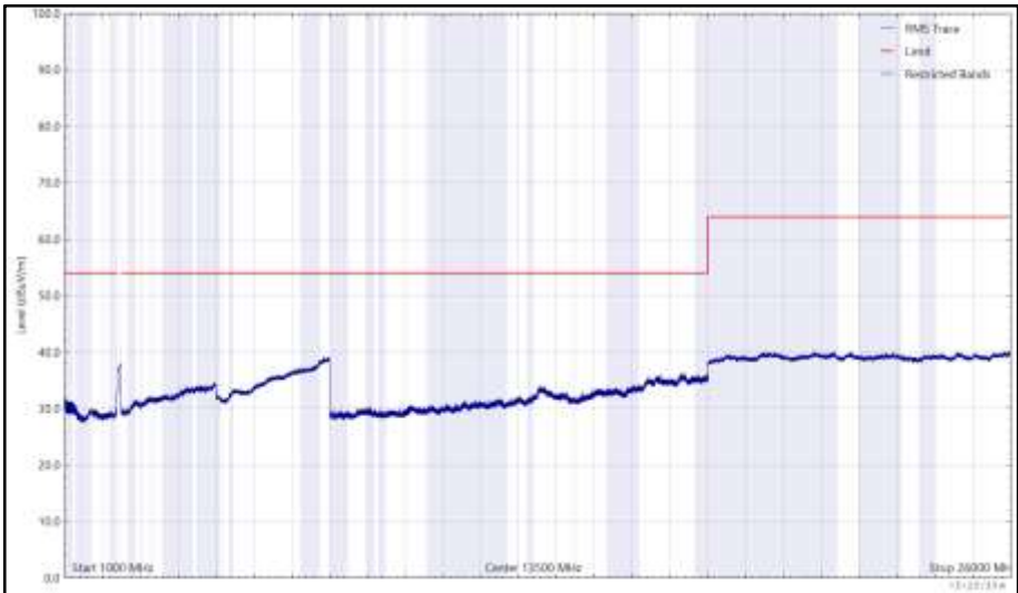
Figure 178 - 2437 MHz (CH6), HE20, RU26-0, Core 0 + Core 1, 1 GHz to 26 GHz, Horizontal (RMS)
