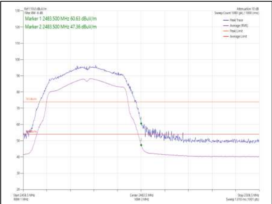
Figure 76 - 802.11g, Core 1 - 2472 MHz, Band Edge Frequency 2483.5 MHz
