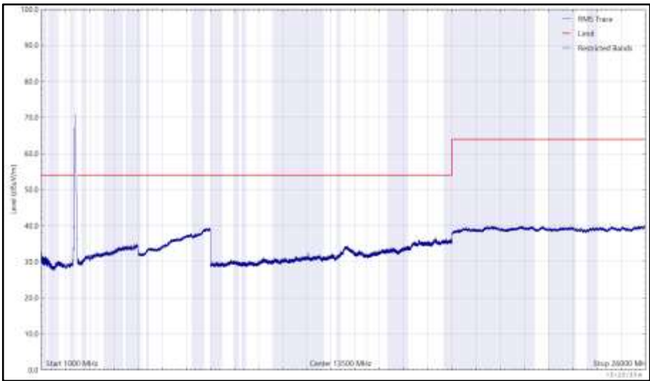
Figure 105 - 2412 MHz (CH1), HT20, CDD, Core 0 + Core 1, 1 GHz to 26 GHz, Vertical (RMS)
