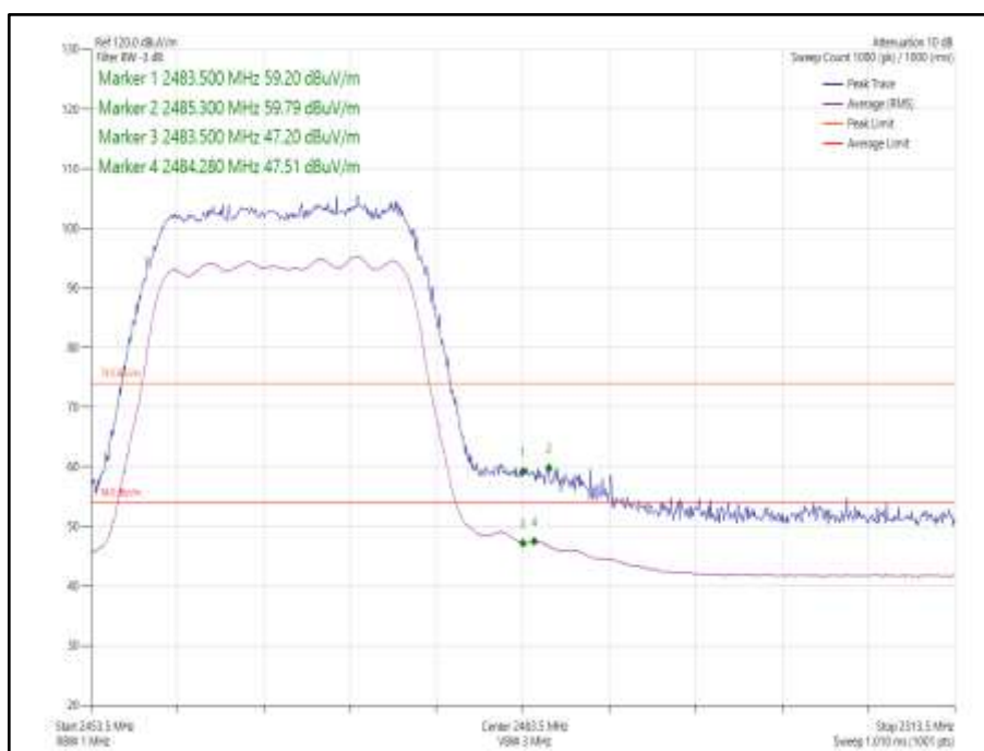
Figure 91 - 802.11n HT20, Core 0-1 - 2467 MHz, Band Edge Frequency 2483.5 MHz
