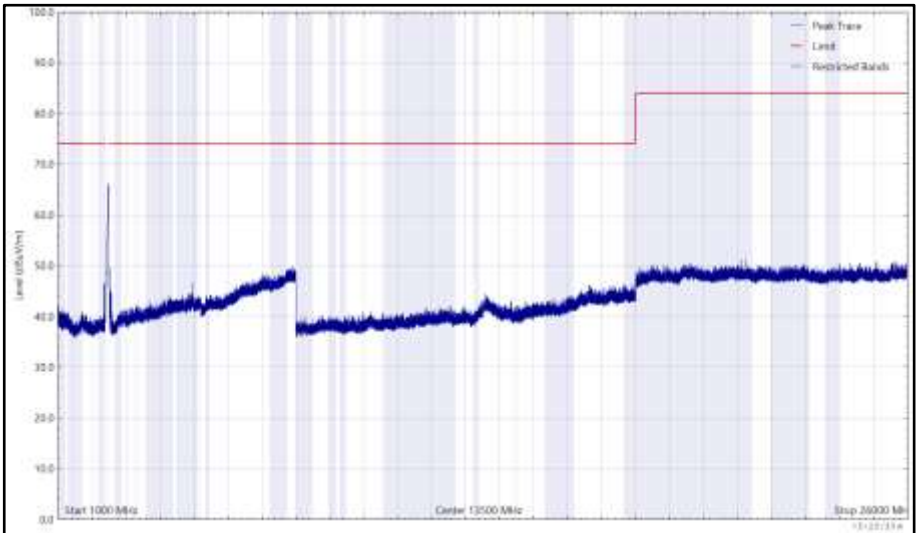
Figure 128 - 2472 MHz (CH13), 802.11g, Core 0, 1 GHz to 26 GHz, Vertical (Peak)
