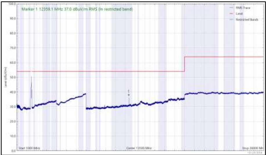
Figure 169 - 2472 MHz (CH13), 802.11b, Core 1, 1 GHz to 26 GHz, Horizontal (RMS)
