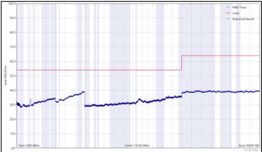
Figure 181 - 2437 MHz (CH6), HE20, RU26-0, Core 0 + Core 1, 1 GHz to 26 GHz, Vertical (RMS)
