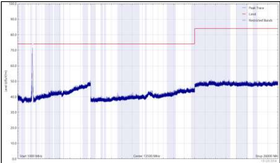
Figure 132 - 2412 MHz (CH1), 802.11g, Core 1, 1 GHz to 26 GHz, Vertical (Peak)
