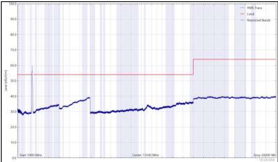
Figure 119 - 2412 MHz (CH1), 802.11g, Core 0, 1 GHz to 26 GHz, Vertical (RMS)
