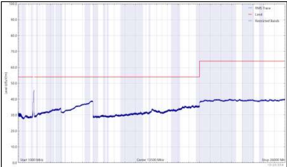
Figure 136 - 2437 MHz (CH6), 802.11g, Core 1, 1 GHz to 26 GHz, Horizontal (RMS)
