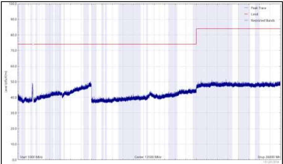
Figure 174 - 2412 MHz (CH1), HE20, RU26-0, Core 0 + Core 1, 1 GHz to 26 GHz, Vertical (Peak)
