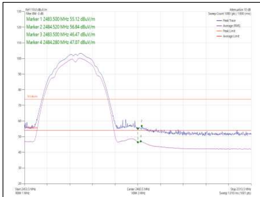
Figure 71 - 802.11b, Core 1 - 2467 MHz, Band Edge Frequency 2483.5 MHz
