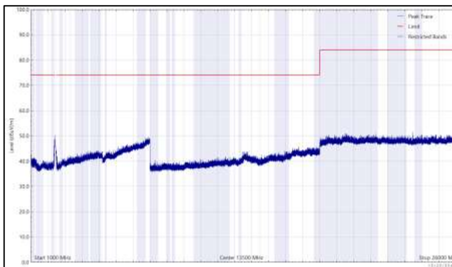
Figure 177 - 2437 MHz (CH6), HE20, RU26-0, Core 0 + Core 1, 1 GHz to 26 GHz, Horizontal (Peak)
