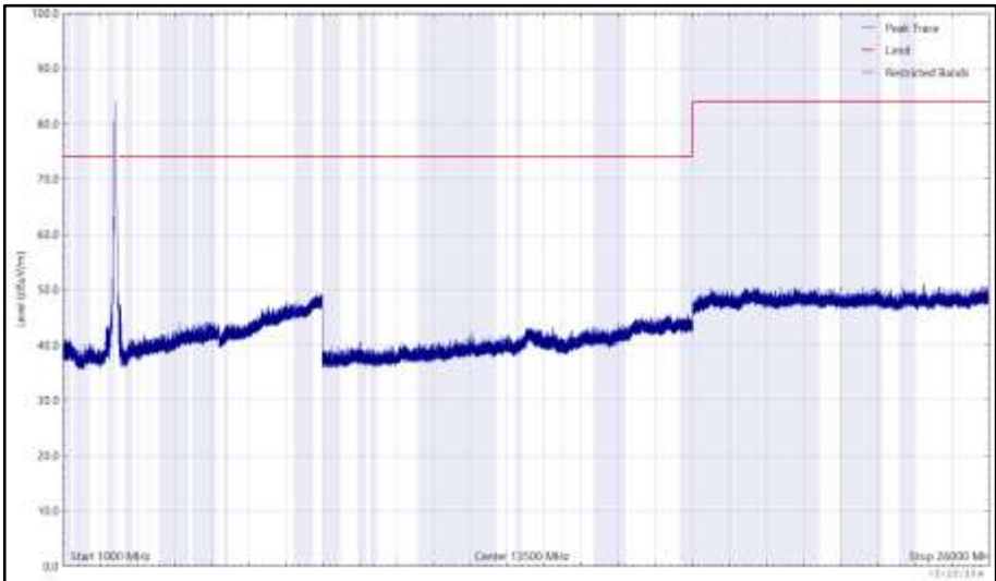
Figure 102 - 2412 MHz (CH1), HT20, CDD, Core 0 + Core 1, 1 GHz to 26 GHz, Horizontal (Peak)
