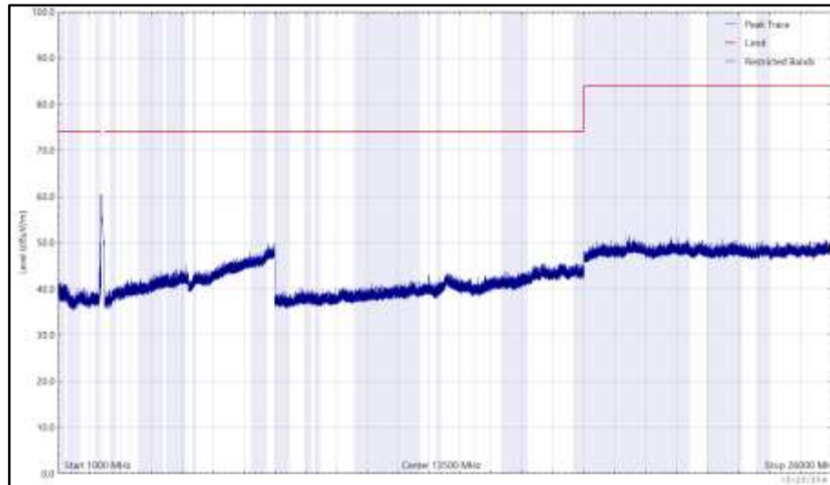
Figure 144 - 2412 MHz (CH1), 802.11b, Core 0, 1 GHz to 26 GHz, Horizontal (Peak)
