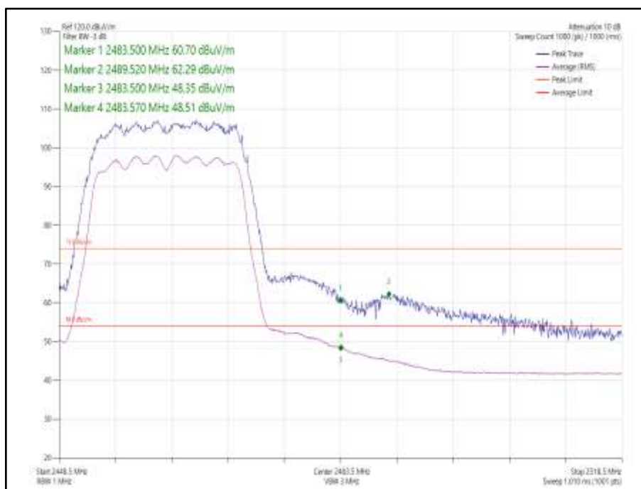
Figure 90 - 802.11n HT20, Core 0-1 - 2462 MHz, Band Edge Frequency 2483.5 MHz
