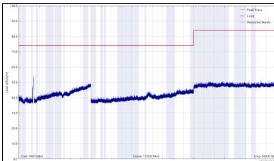
Figure 166 - 2437 MHz (CH6), 802.11b, Core 1, 1 GHz to 26 GHz, Vertical (Peak)
