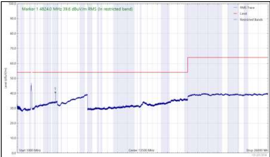
Figure 147 - 2412 MHz (CH1), 802.11b, Core 0, 1 GHz to 26 GHz, Vertical (RMS)
