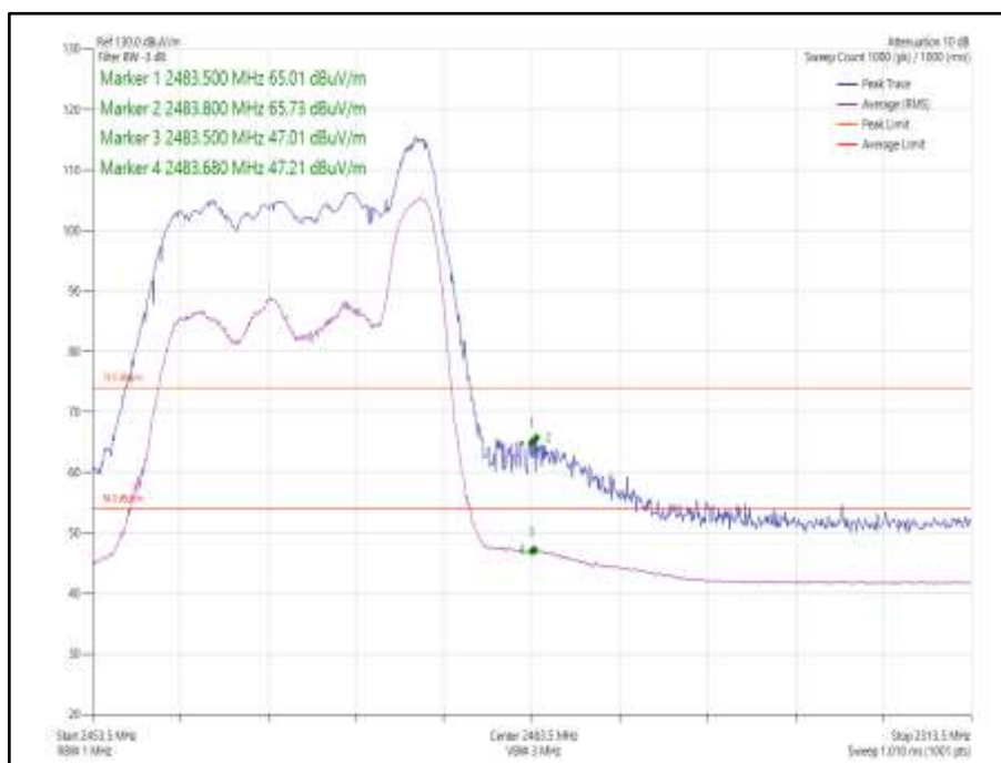
Figure 98 - 802.11ax HE20, Core 0-1, 26-8 - 2467 MHz, Band Edge Frequency 2483.5 MHz
