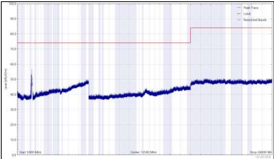
Figure 138 - 2437 MHz (CH6), 802.11g, Core 1, 1 GHz to 26 GHz, Vertical (Peak)
