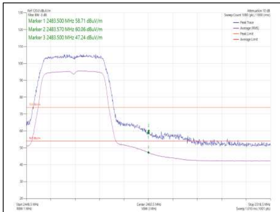
Figure 78 - 802.11n HT20, Core 1 - 2462 MHz, Band Edge Frequency 2483.5 MHz
