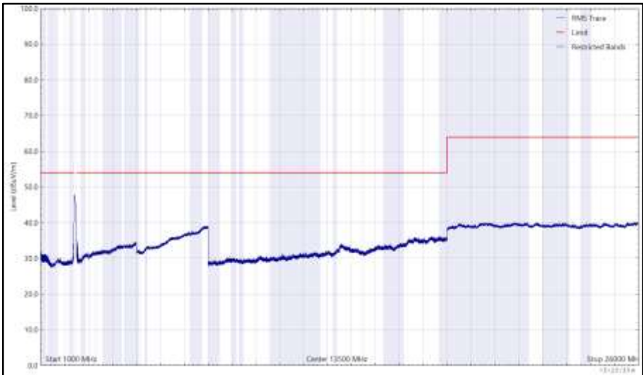
Figure 122 - 2437 MHz (CH6), 802.11g, Core 0, 1 GHz to 26 GHz, Horizontal (RMS)
