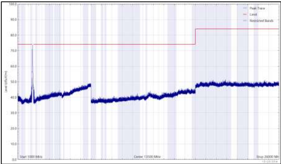
Figure 116 - 2412 MHz (CH1), 802.11g, Core 0, 1 GHz to 26 GHz, Horizontal (Peak)
