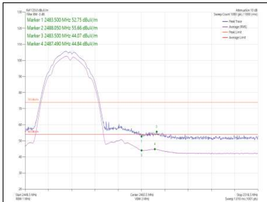
Figure 70 - 802.11b, Core 1 - 2462 MHz, Band Edge Frequency 2483.5 MHz
