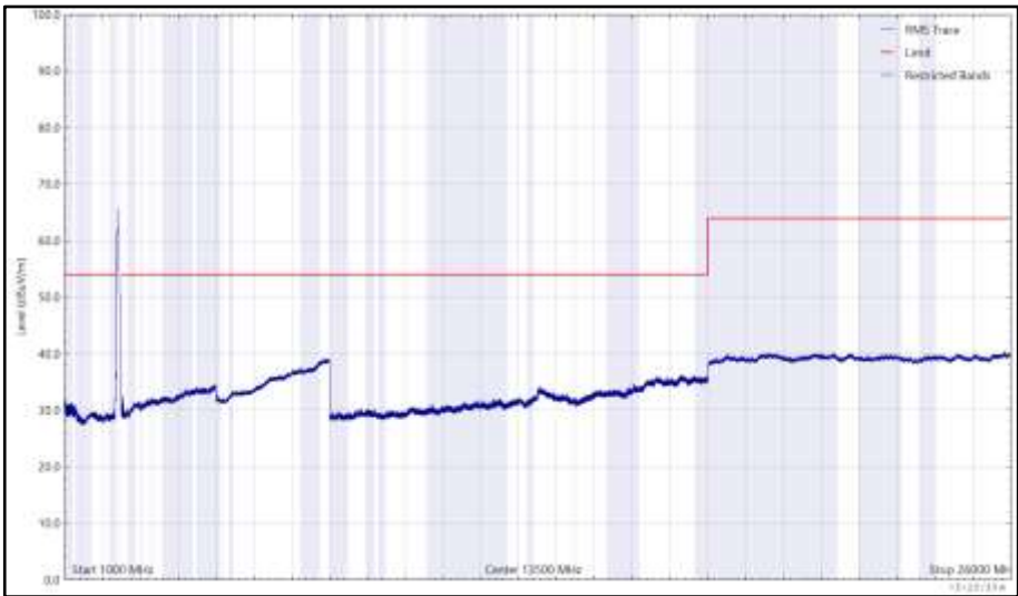
Figure 117 - 2412 MHz (CH1), 802.11g, Core 0, 1 GHz to 26 GHz, Horizontal (RMS)
