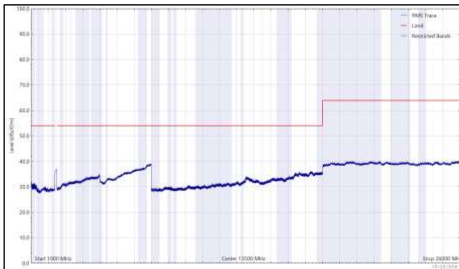
Figure 173 - 2412 MHz (CH1), HE20, RU26-0, Core 0 + Core 1, 1 GHz to 26 GHz, Horizontal (RMS)
