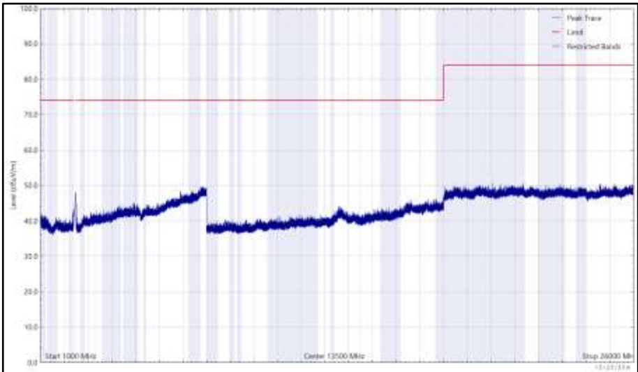
Figure 184 - 2472 MHz (CH13), HE20, RU26-8, Core 0 + Core 1, 1 GHz to 26 GHz, Vertical (Peak)
