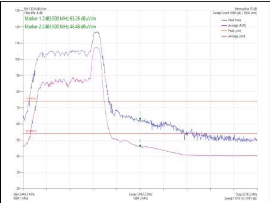
Figure 84 - 802.11ax HE20, Core 1, 26-8 - 2462 MHz, Band Edge Frequency 2483.5 MHz
