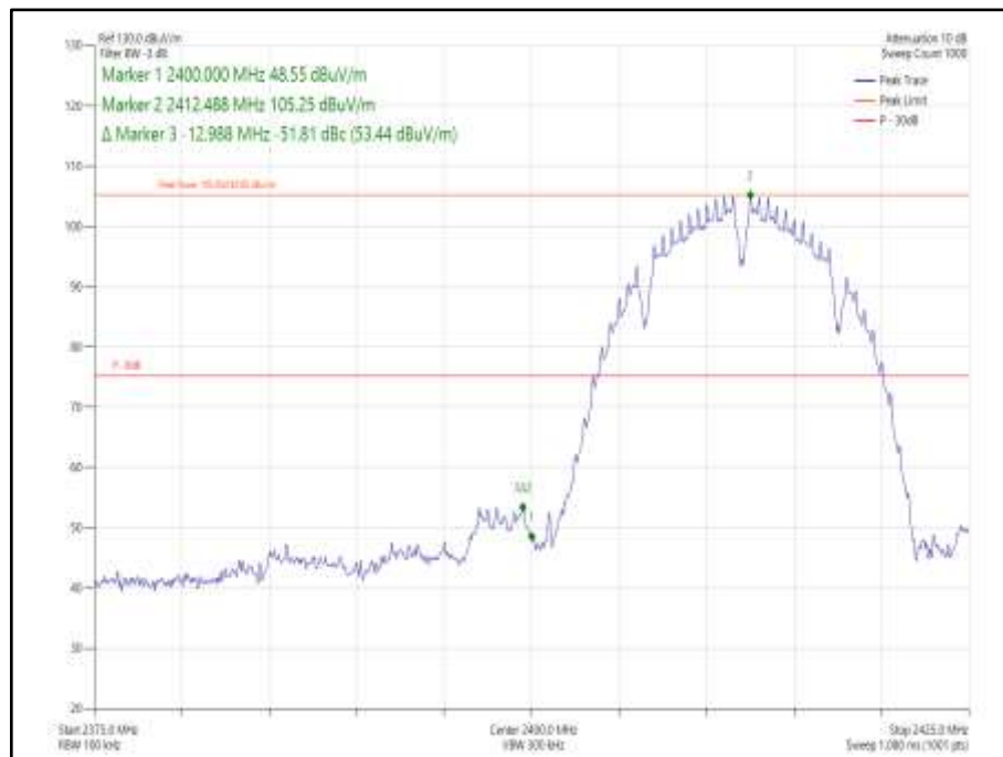
Figure 61 - 802.11b, Core 1 - 2412 MHz Band Edge Frequency 2400 MHz
