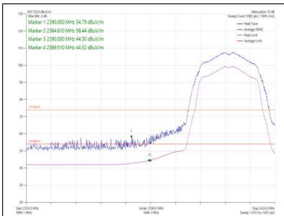
Figure 73 - 802.11g, Core 1 - 2412 MHz, Band Edge Frequency 2390.0 MHz
