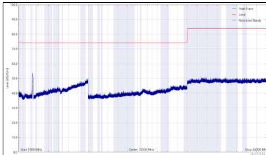
Figure 149 - 2437 MHz (CH6), 802.11b, Core 0, 1 GHz to 26 GHz, Horizontal (Peak)
