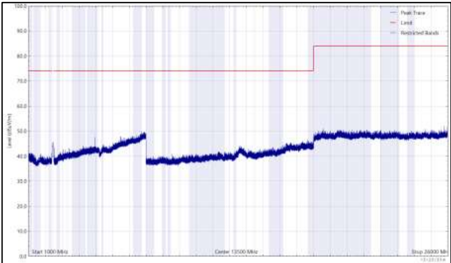
Figure 156 - 2472 MHz (CH13), 802.11b, Core 0, 1 GHz to 26 GHz, Vertical (Peak)
