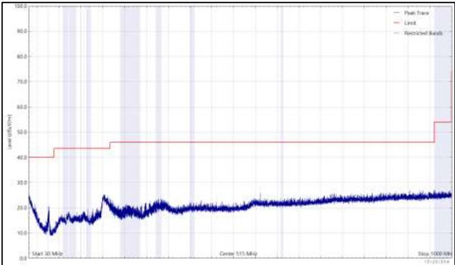
Figure 179 - 2437 MHz (CH6), HE20, RU26-0, Core 0 + Core 1, 30 MHz to 1 GHz, Vertical (Peak)
