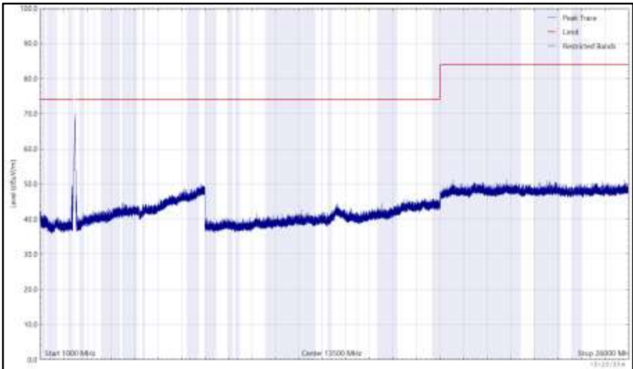
Figure 142 - 2472 MHz (CH13), 802.11g, Core 1, 1 GHz to 26 GHz, Vertical (Peak)
