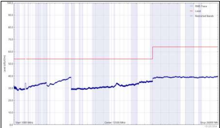
Figure 175 - 2412 MHz (CH1), HE20, RU26-0, Core 0 + Core 1, 1 GHz to 26 GHz, Vertical (RMS)
