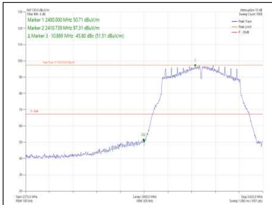
Figure 62- 802.11g, Core 1 - 2412 MHz Band Edge Frequency 2400 MHz
