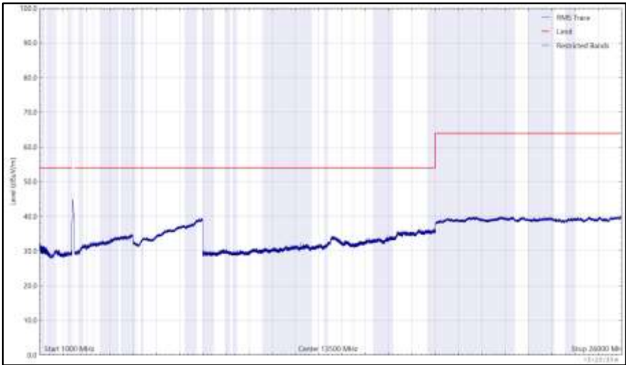
Figure 167 - 2437 MHz (CH6), 802.11b, Core 1, 1 GHz to 26 GHz, Vertical (RMS)
