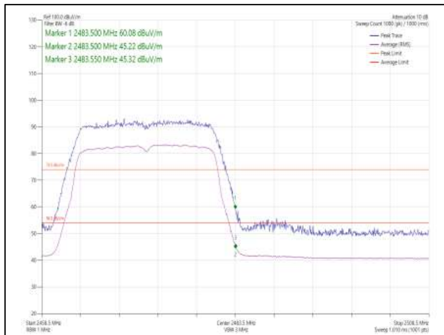
Figure 80 - 802.11n HT20, Core 1 - 2472 MHz, Band Edge Frequency 2483.5 MHz
