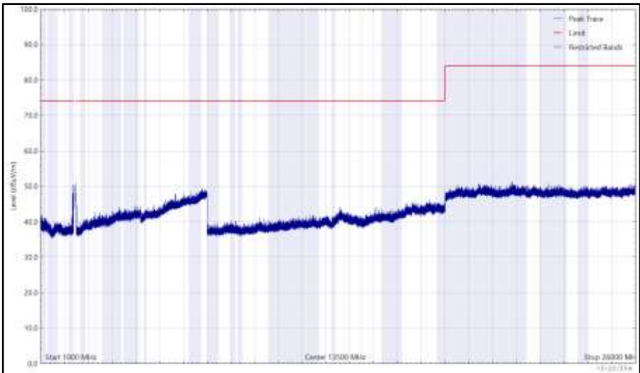
Figure 135 - 2437 MHz (CH6), 802.11g, Core 1, 1 GHz to 26 GHz, Horizontal (Peak)
