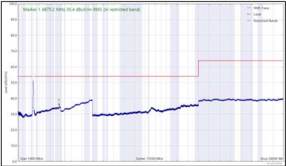
Figure 111 - 2437 MHz (CH6), HT20, CDD, Core 0 + Core 1, 1 GHz to 26 GHz, Vertical (RMS)
