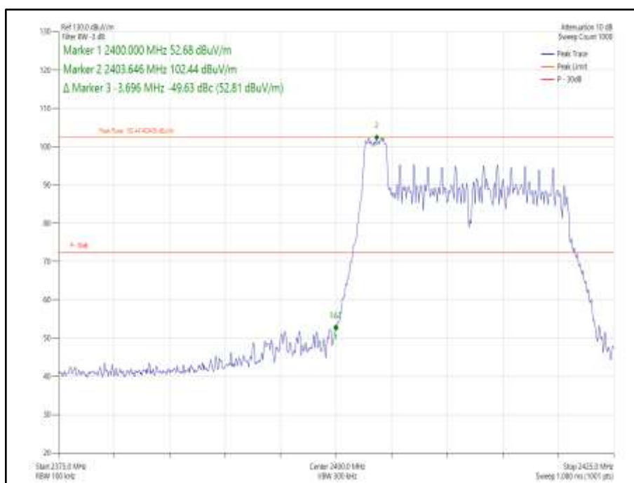
Figure 65- 802.11ax HE20, Core 1, 26-0 - 2412 MHz Band Edge Frequency 2400 MHz
