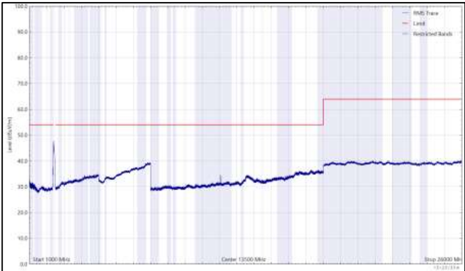
Figure 161 - 2412 MHz (CH1), 802.11b, Core 1, 1 GHz to 26 GHz, Vertical (RMS)
