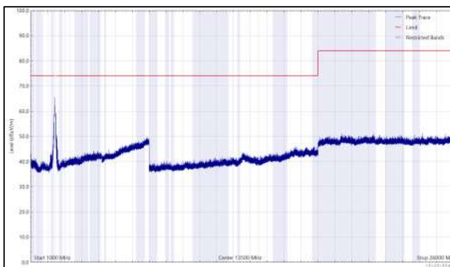
Figure 107 - 2437 MHz (CH6), HT20, CDD, Core 0 + Core 1, 1 GHz to 26 GHz, Horizontal (Peak)
