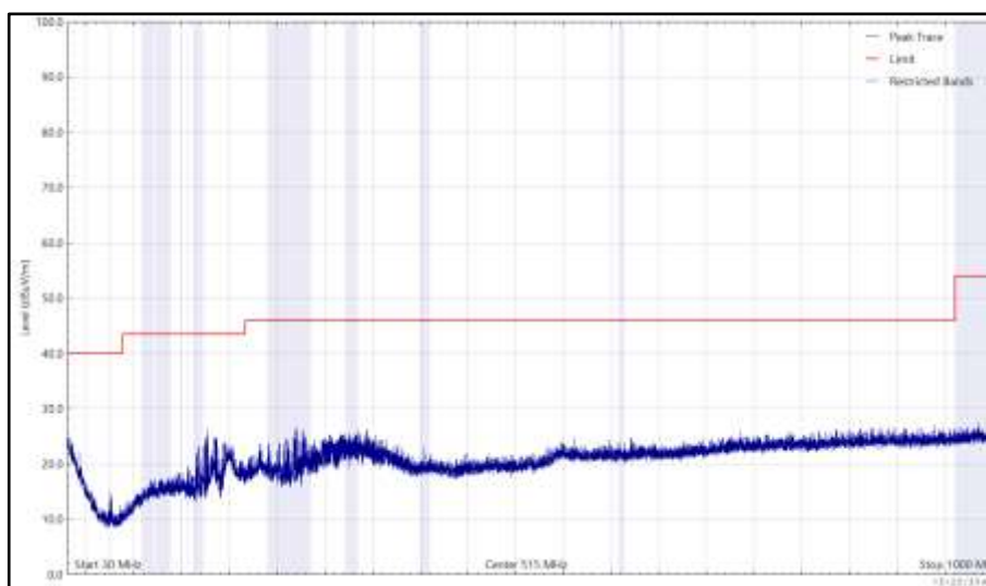
Figure 106 - 2437 MHz (CH6), HT20, CDD, Core 0 + Core 1, 30 MHz to 1 GHz, Horizontal (Peak)
