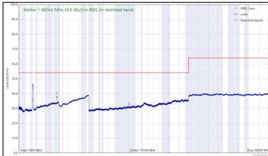
Figure 159 - 2412 MHz (CH1), 802.11b, Core 1, 1 GHz to 26 GHz, Horizontal (RMS)
