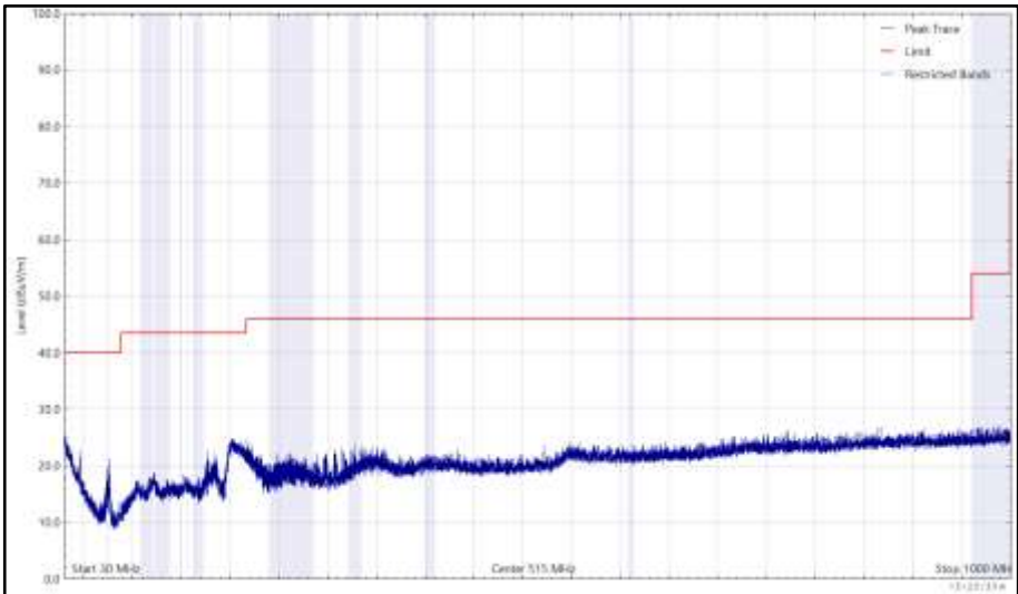
Figure 123 - 2437 MHz (CH6), 802.11g, Core 0, 30 MHz to 1 GHz, Vertical (Peak)
