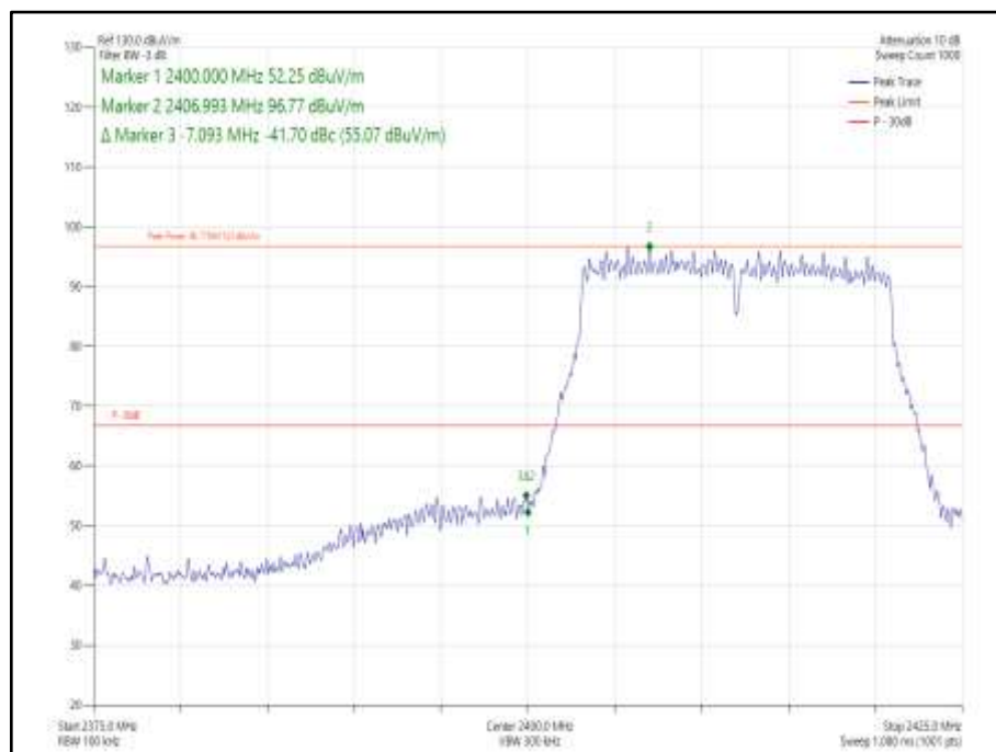
Figure 63- 802.11n HT20, Core 1 - 2412 MHz Band Edge Frequency 2400 MHz
