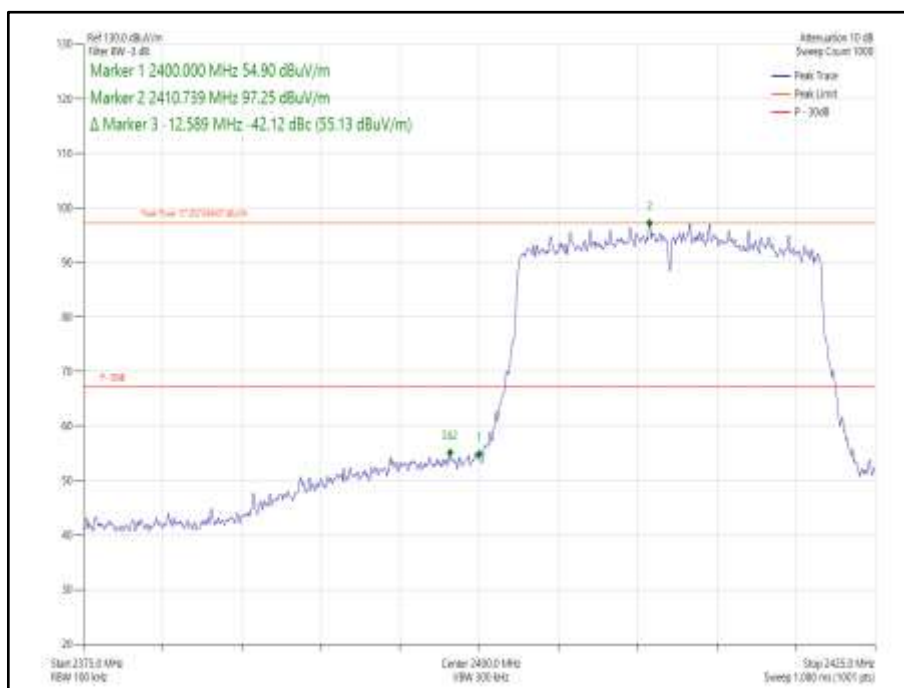
Figure 64- 802.11ax HE20, Core 1, SU - 2412 MHz Band Edge Frequency 2400 MHz
