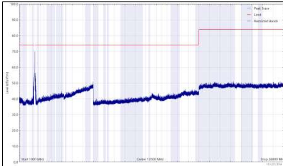
Figure 126 - 2472 MHz (CH13), 802.11g, Core 0, 1 GHz to 26 GHz, Horizontal (Peak)
