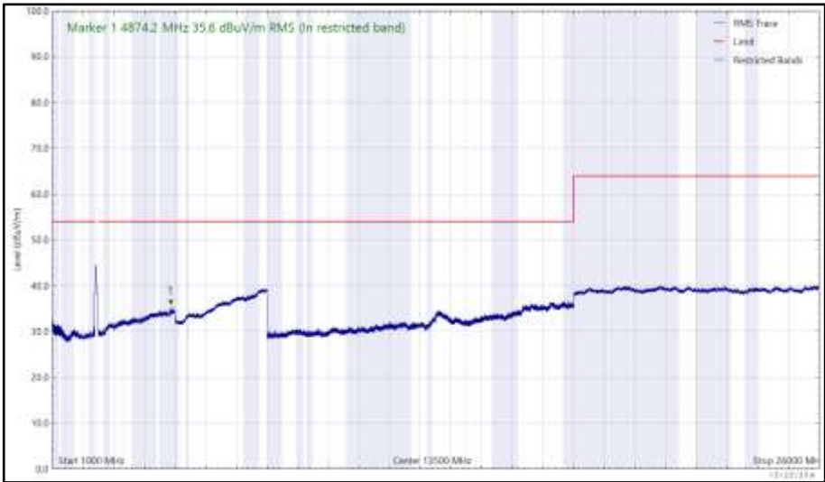
Figure 125 - 2437 MHz (CH6), 802.11g, Core 0, 1 GHz to 26 GHz, Vertical (RMS)
