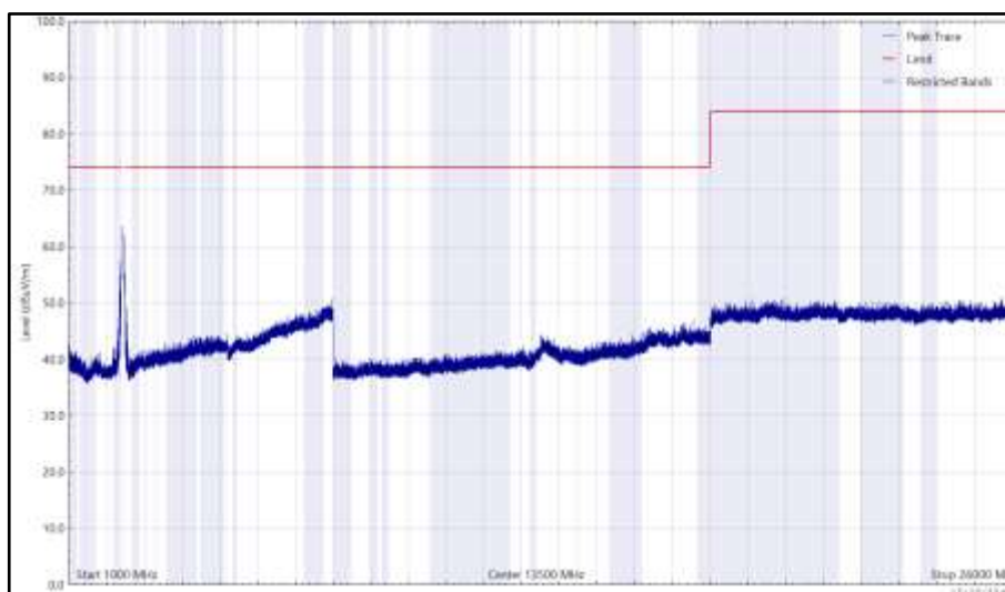
Figure 110 - 2437 MHz (CH6), HT20, CDD, Core 0 + Core 1, 1 GHz to 26 GHz, Vertical (Peak)
