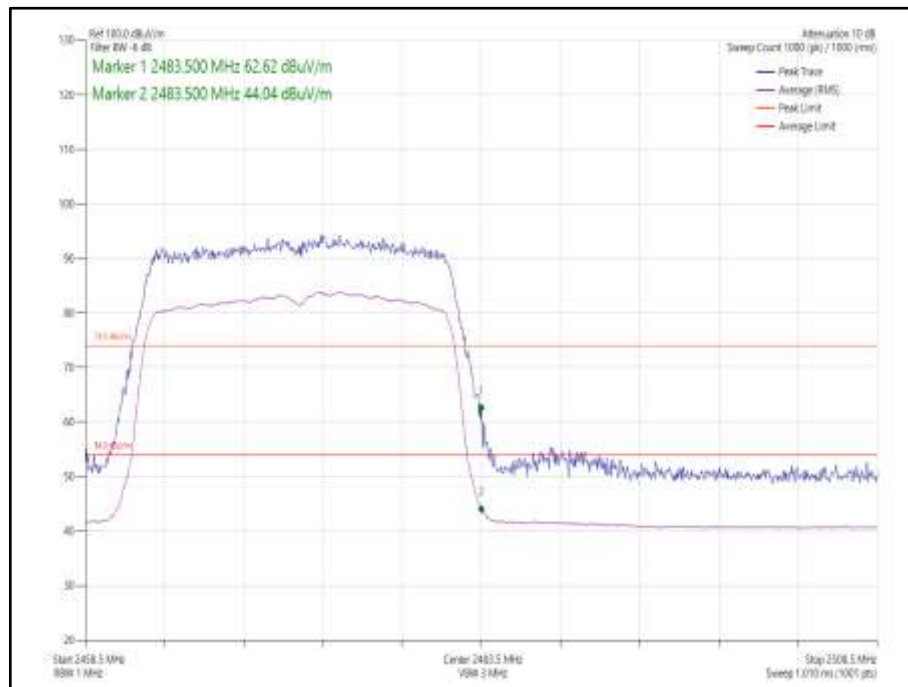
Figure 87 - 802.11ax HE20, Core 1, SU - 2472 MHz, Band Edge Frequency 2483.5 MHz
