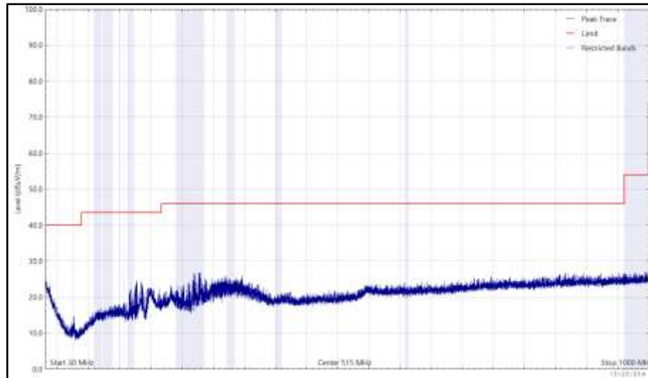
Figure 162 - 2437 MHz (CH6), 802.11b, Core 1, 30 MHz to 1 GHz, Horizontal (Peak)
