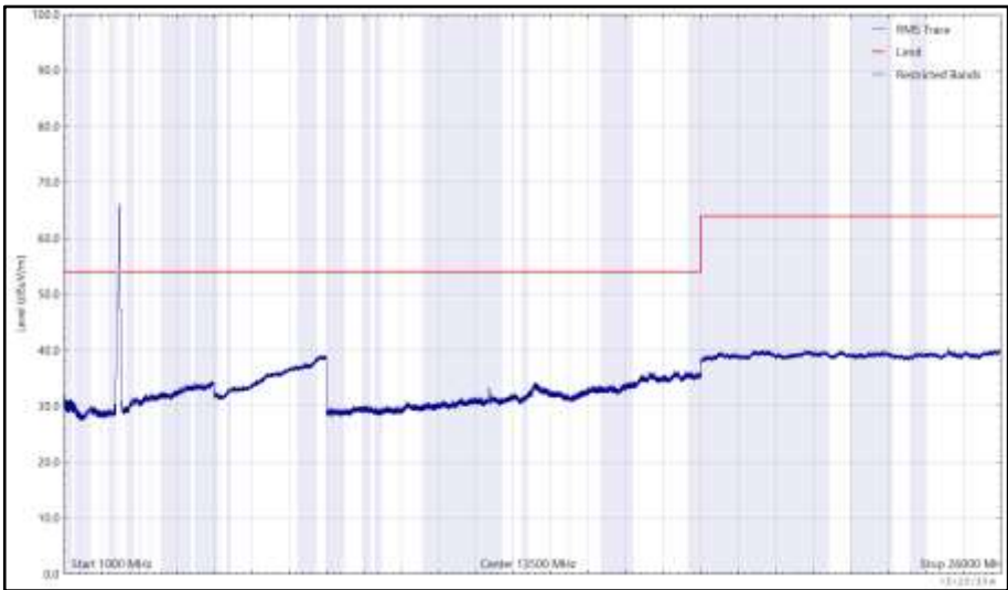
Figure 141 - 2472 MHz (CH13), 802.11g, Core 1, 1 GHz to 26 GHz, Horizontal (RMS)
