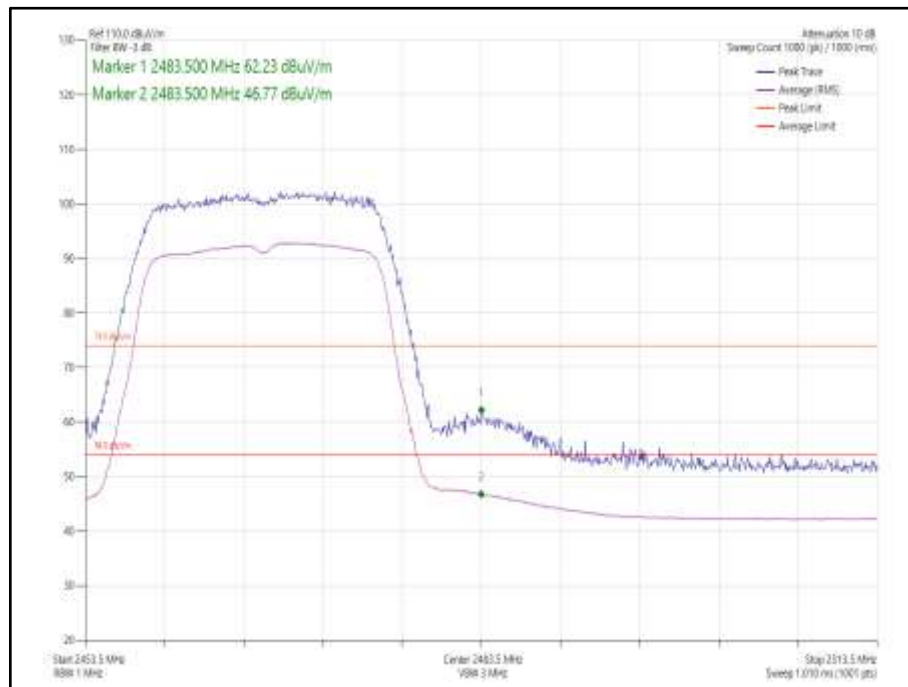
Figure 79 - 802.11n HT20, Core 1 - 2467 MHz, Band Edge Frequency 2483.5 MHz
