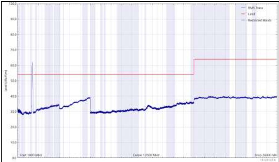
Figure 133 - 2412 MHz (CH1), 802.11g, Core 1, 1 GHz to 26 GHz, Vertical (RMS)
