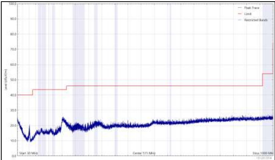
Figure 137 - 2437 MHz (CH6), 802.11g, Core 1, 30 MHz to 1 GHz, Vertical (Peak)
