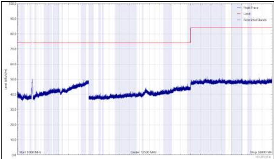
Figure 170 - 2472 MHz (CH13), 802.11b, Core 1, 1 GHz to 26 GHz, Vertical (Peak)
