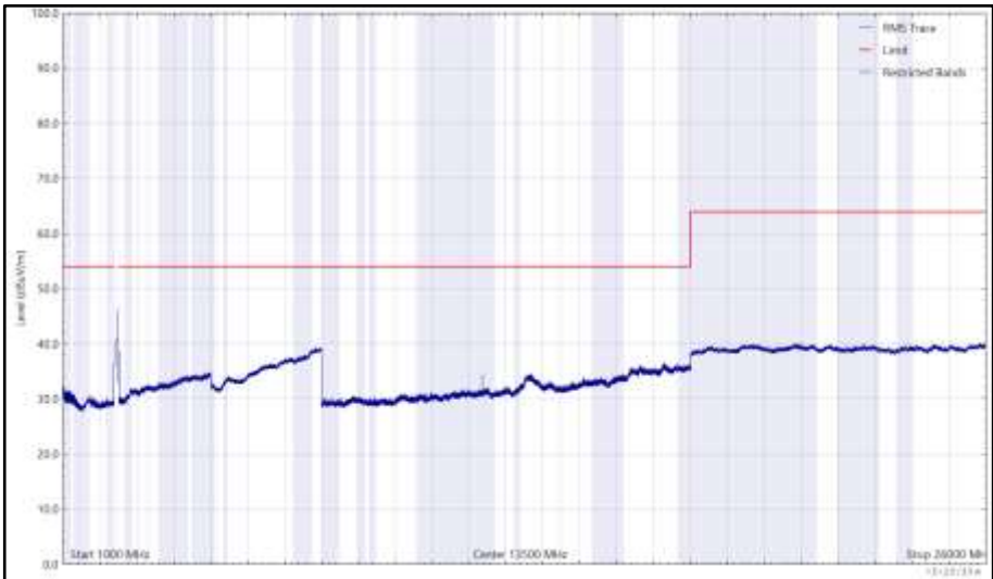
Figure 171 - 2472 MHz (CH13), 802.11b, Core 1, 1 GHz to 26 GHz, Vertical (RMS)
