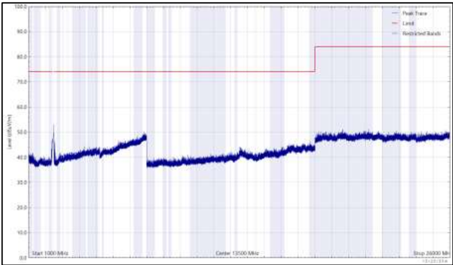
Figure 182 - 2472 MHz (CH13), HE20, RU26-8, Core 0 + Core 1, 1 GHz to 26 GHz, Horizontal (Peak)
