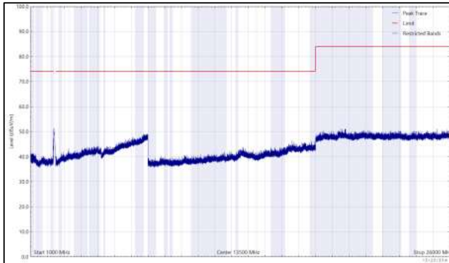
Figure 172 - 2412 MHz (CH1), HE20, RU26-0, Core 0 + Core 1, 1 GHz to 26 GHz, Horizontal (Peak)
