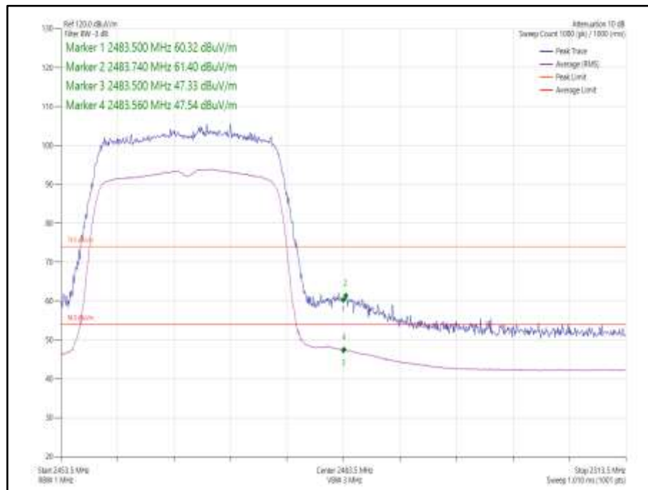
Figure 85 - 802.11ax HE20, Core 1, SU - 2467 MHz, Band Edge Frequency 2483.5 MHz
