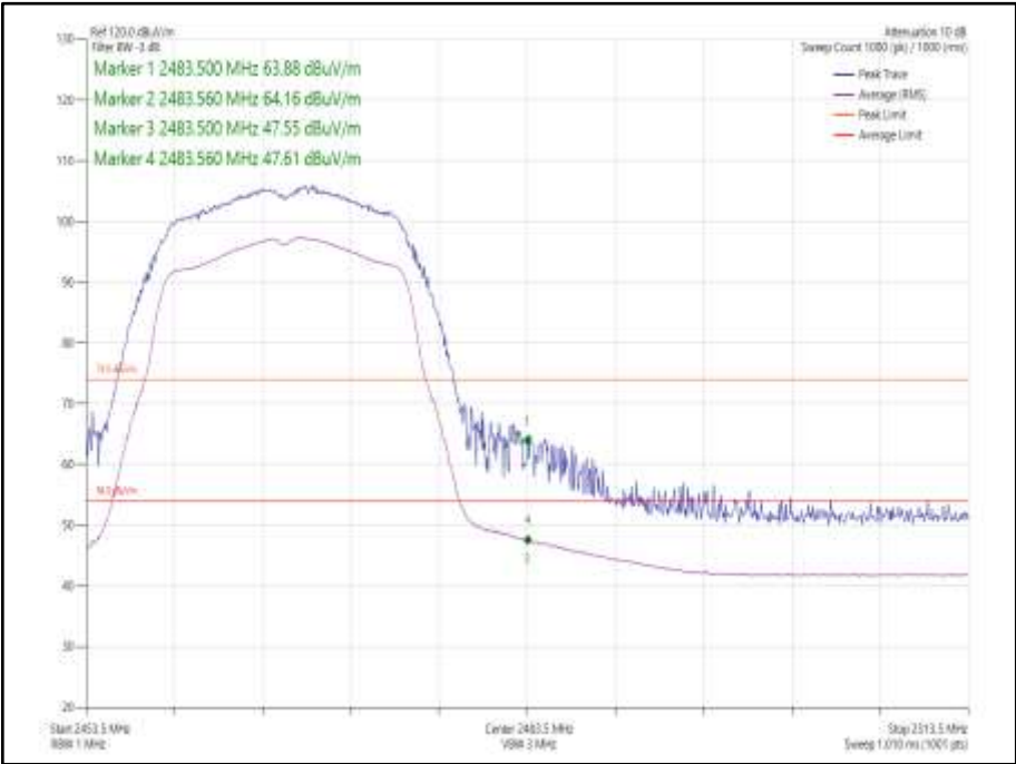
Figure 75 - 802.11g, Core 1 - 2467 MHz, Band Edge Frequency 2483.5 MHz
