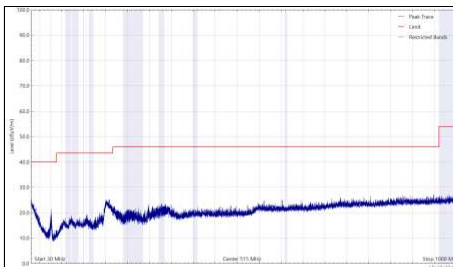
Figure 151 - 2437 MHz (CH6), 802.11b, Core 0, 30 MHz to 1 GHz, Vertical (Peak)
