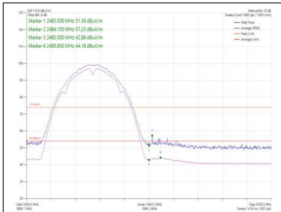
Figure 72 - 802.11b, Core 1 - 2472 MHz, Band Edge Frequency 2483.5 MHz
