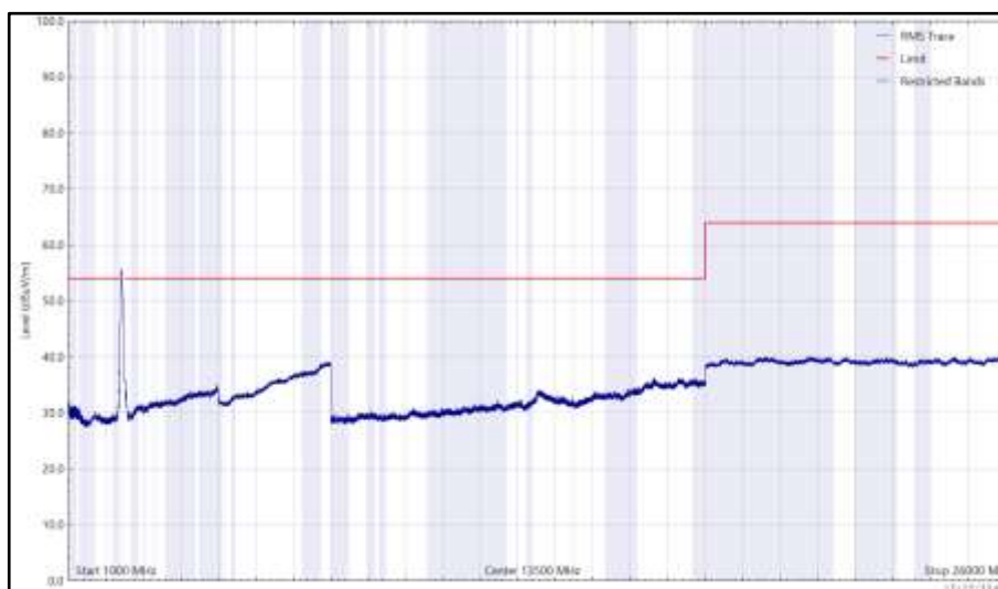
Figure 108 - 2437 MHz (CH6), HT20, CDD, Core 0 + Core 1, 1 GHz to 26 GHz, Horizontal (RMS)
