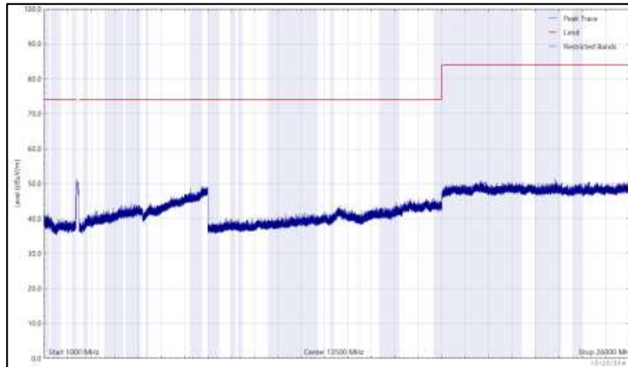
Figure 158 - 2412 MHz (CH1), 802.11b, Core 1, 1 GHz to 26 GHz, Horizontal (Peak)
