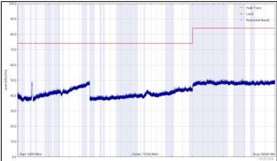
Figure 146 - 2412 MHz (CH1), 802.11b, Core 0, 1 GHz to 26 GHz, Vertical (Peak)
