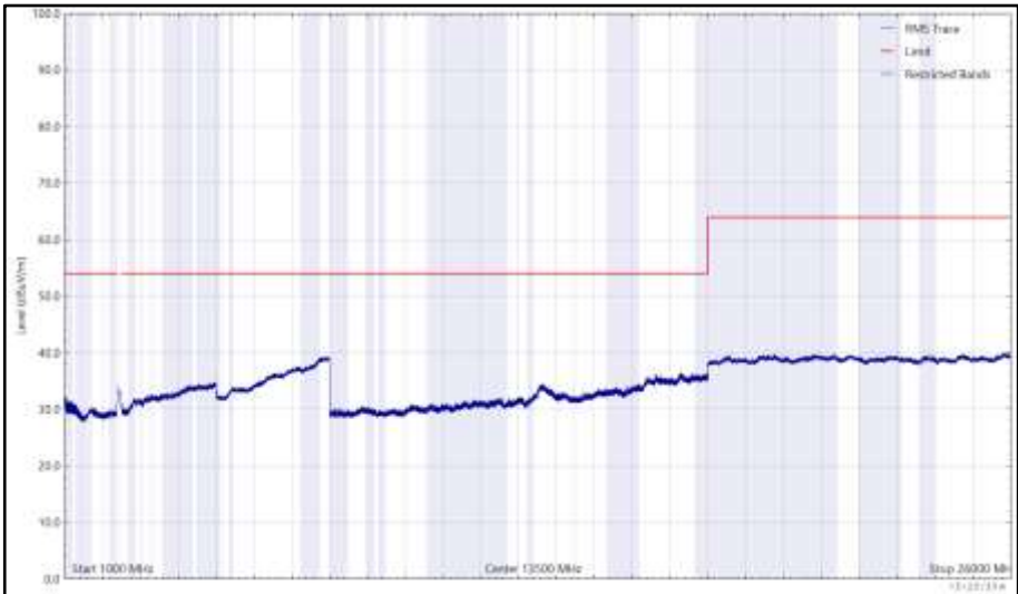
Figure 185 - 2472 MHz (CH13), HE20, RU26-8, Core 0 + Core 1, 1 GHz to 26 GHz, Vertical (RMS)
