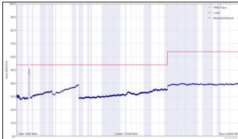
Figure 145 - 2412 MHz (CH1), 802.11b, Core 0, 1 GHz to 26 GHz, Horizontal (RMS)
