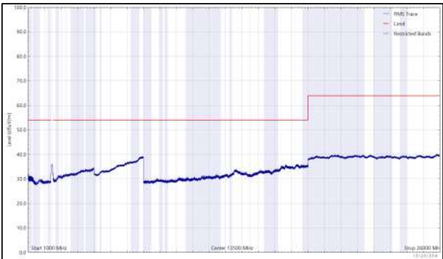
Figure 183 - 2472 MHz (CH13), HE20, RU26-8, Core 0 + Core 1, 1 GHz to 26 GHz, Horizontal (RMS)
