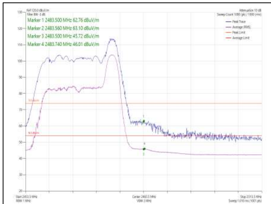
Figure 86 - 802.11ax HE20, Core 1, 26-8 - 2467 MHz, Band Edge Frequency 2483.5 MHz
