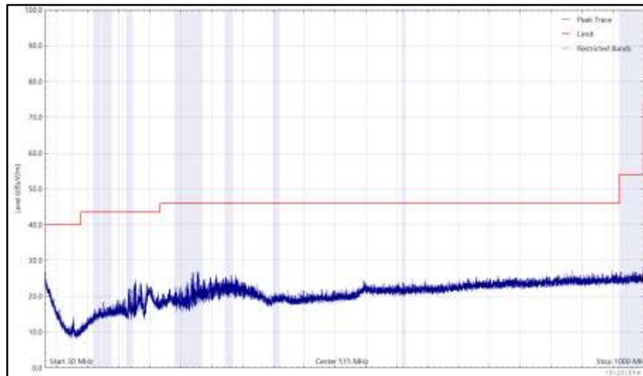
Figure 148 - 2437 MHz (CH6), 802.11b, Core 0, 30 MHz to 1 GHz, Horizontal (Peak)
