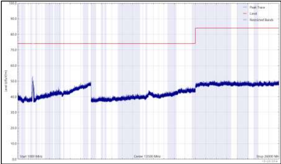
Figure 124 - 2437 MHz (CH6), 802.11g, Core 0, 1 GHz to 26 GHz, Vertical (Peak)
