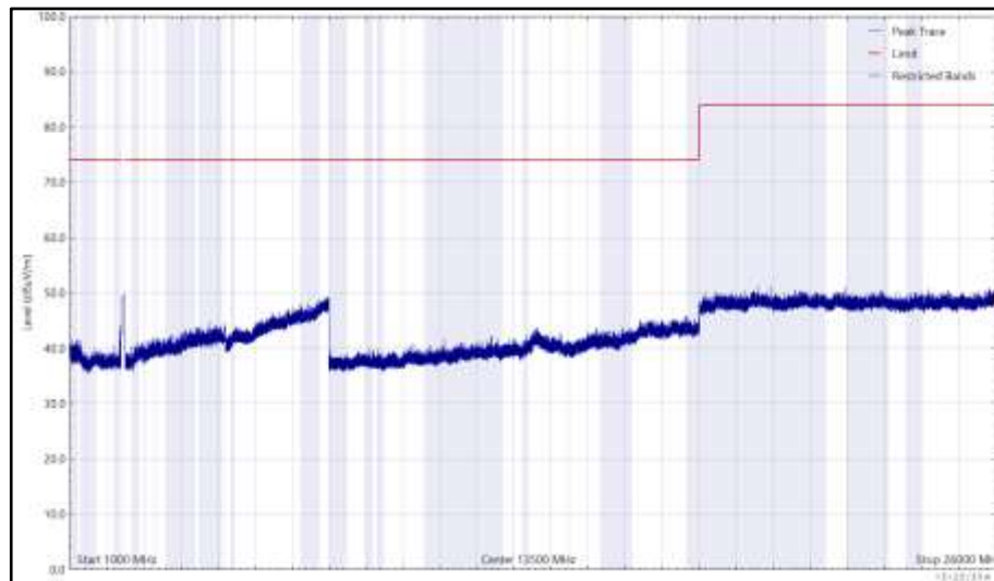
Figure 163 - 2437 MHz (CH6), 802.11b, Core 1, 1 GHz to 26 GHz, Horizontal (Peak)
