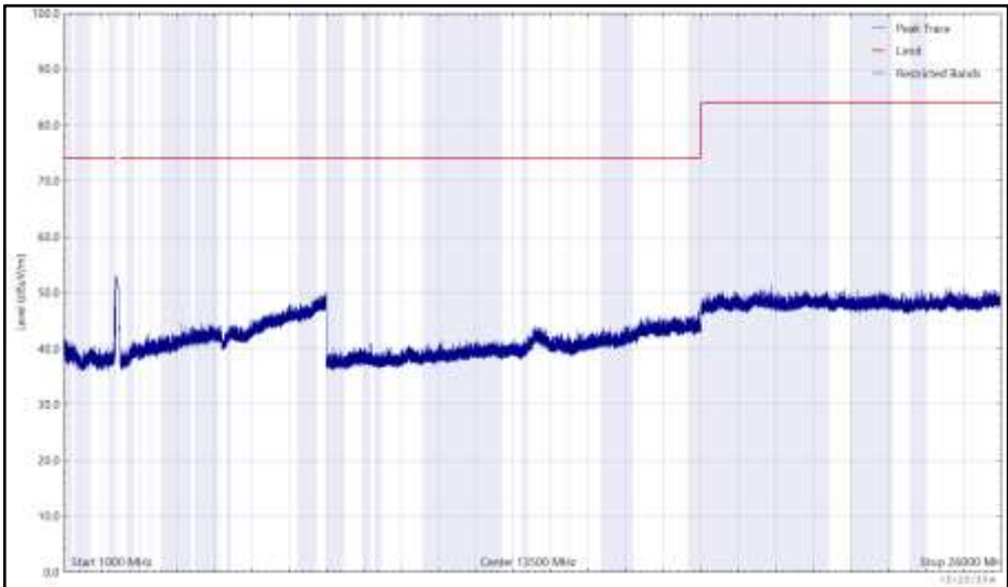
Figure 160 - 2412 MHz (CH1), 802.11b, Core 1, 1 GHz to 26 GHz, Vertical (Peak)
