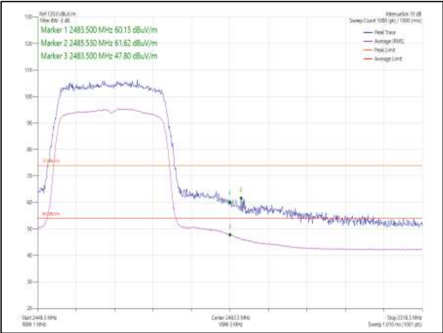
Figure 83 - 802.11ax HE20, Core 1, SU - 2462 MHz, Band Edge Frequency 2483.5 MHz
