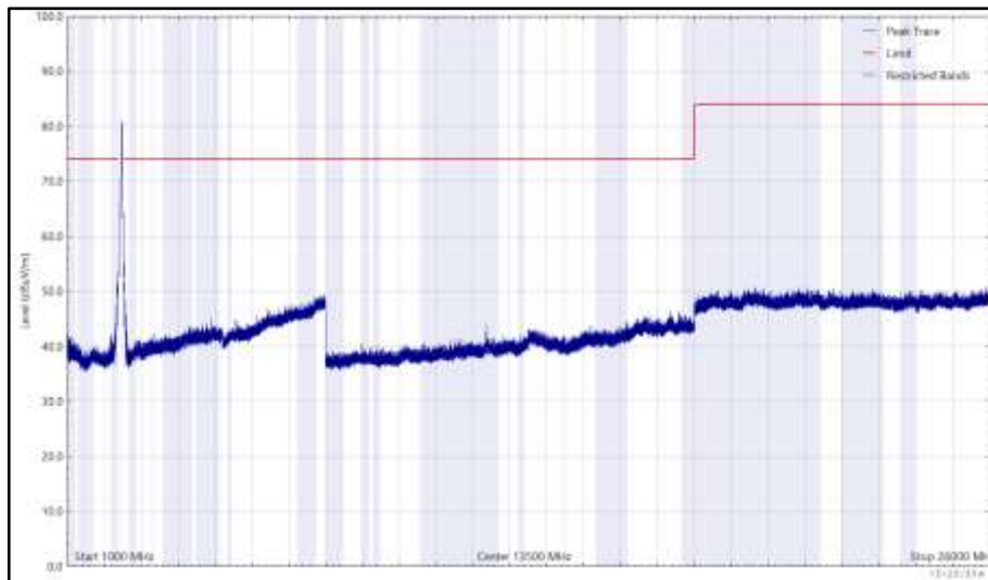
Figure 112 - 2472 MHz (CH13), HT20, CDD, Core 0 + Core 1, 1 GHz to 26 GHz, Horizontal (Peak)
