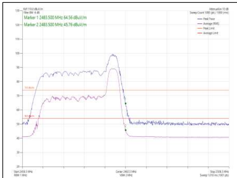
Figure 88 - 802.11ax HE20, Core 1, 26-8 - 2472 MHz, Band Edge Frequency 2483.5 MHz
