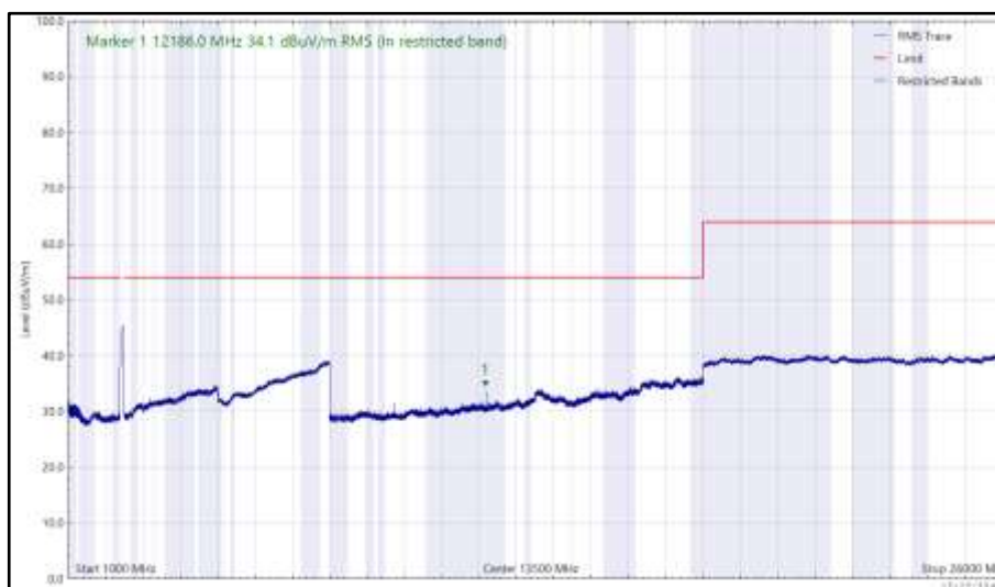
Figure 164 - 2437 MHz (CH6), 802.11b, Core 1, 1 GHz to 26 GHz, Horizontal (RMS)
