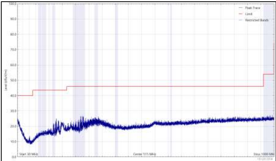
Figure 134 - 2437 MHz (CH6), 802.11g, Core 1, 30 MHz to 1 GHz, Horizontal (Peak)
