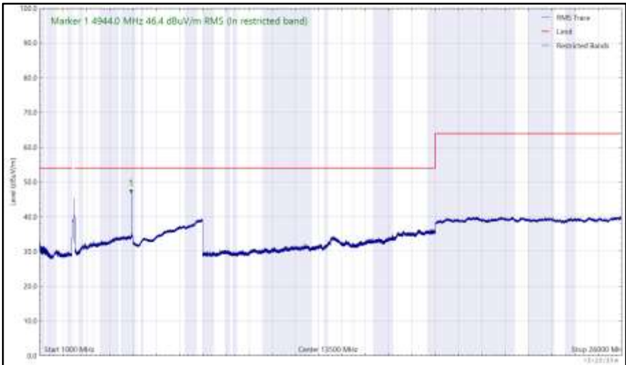
Figure 157 - 2472 MHz (CH13), 802.11b, Core 0, 1 GHz to 26 GHz, Vertical (RMS)
