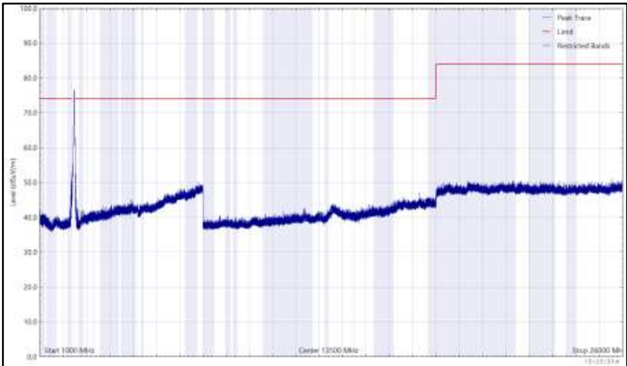
Figure 114 - 2472 MHz (CH13), HT20, CDD, Core 0 + Core 1, 1 GHz to 26 GHz, Vertical (Peak)
