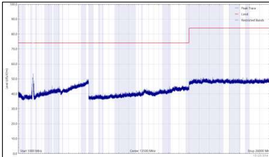
Figure 154 - 2472 MHz (CH13), 802.11b, Core 0, 1 GHz to 26 GHz, Horizontal (Peak)
