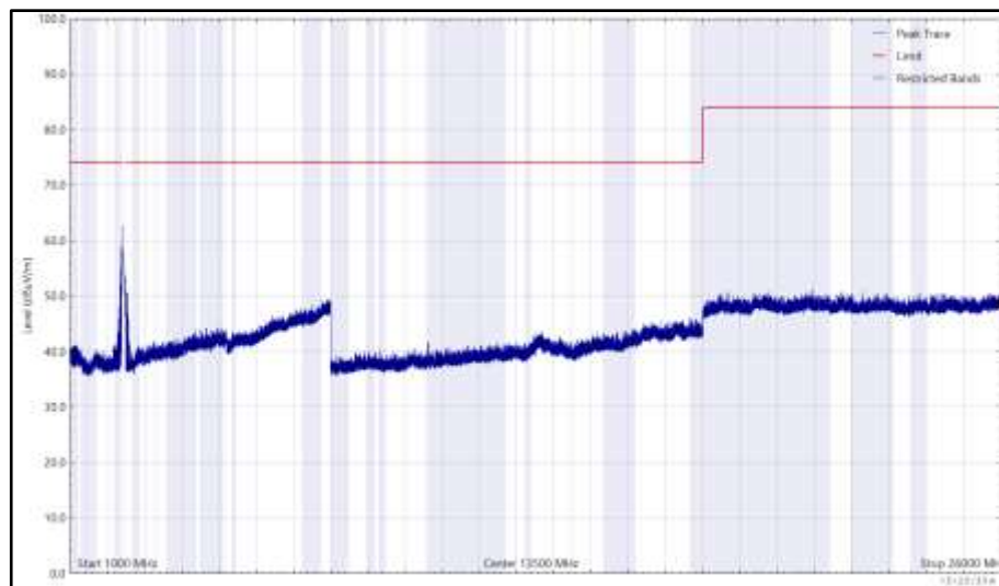
Figure 121 - 2437 MHz (CH6), 802.11g, Core 0, 1 GHz to 26 GHz, Horizontal (Peak)
