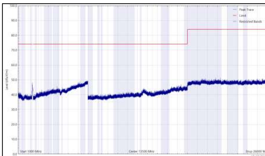
Figure 152 - 2437 MHz (CH6), 802.11b, Core 0, 1 GHz to 26 GHz, Vertical (Peak)
