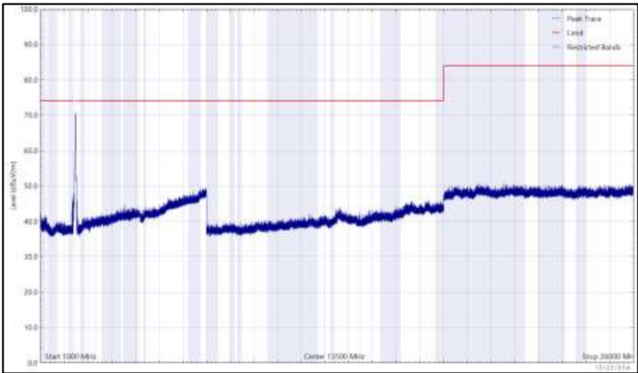
Figure 140 - 2472 MHz (CH13), 802.11g, Core 1, 1 GHz to 26 GHz, Horizontal (Peak)
