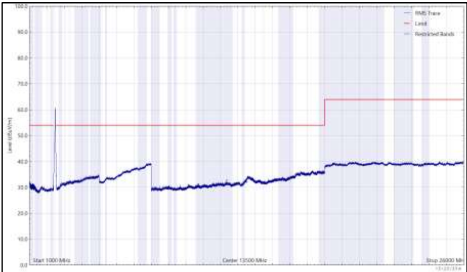
Figure 143 - 2472 MHz (CH13), 802.11g, Core 1, 1 GHz to 26 GHz, Vertical (RMS)
