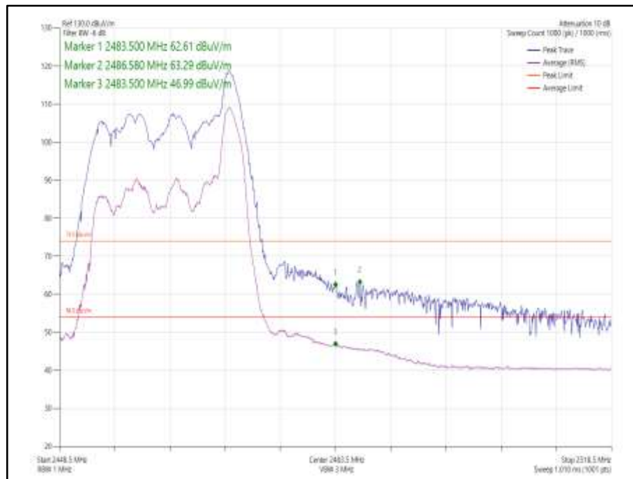
Figure 96 - 802.11ax HE20, Core 0-1, 26-8 - 2462 MHz, Band Edge Frequency 2483.5 MHz
