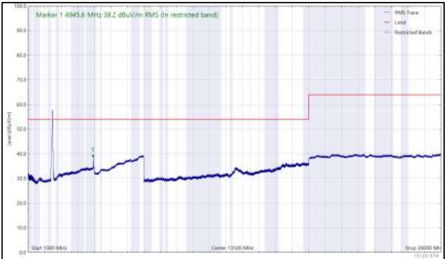
Figure 129 - 2472 MHz (CH13), 802.11g, Core 0, 1 GHz to 26 GHz, Vertical (RMS)
