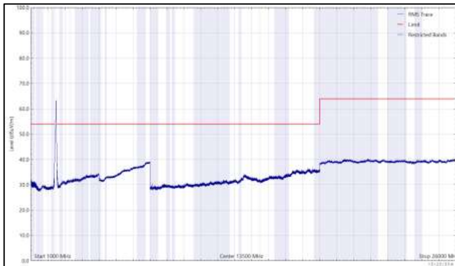
Figure 127 - 2472 MHz (CH13), 802.11g, Core 0, 1 GHz to 26 GHz, Horizontal (RMS)
