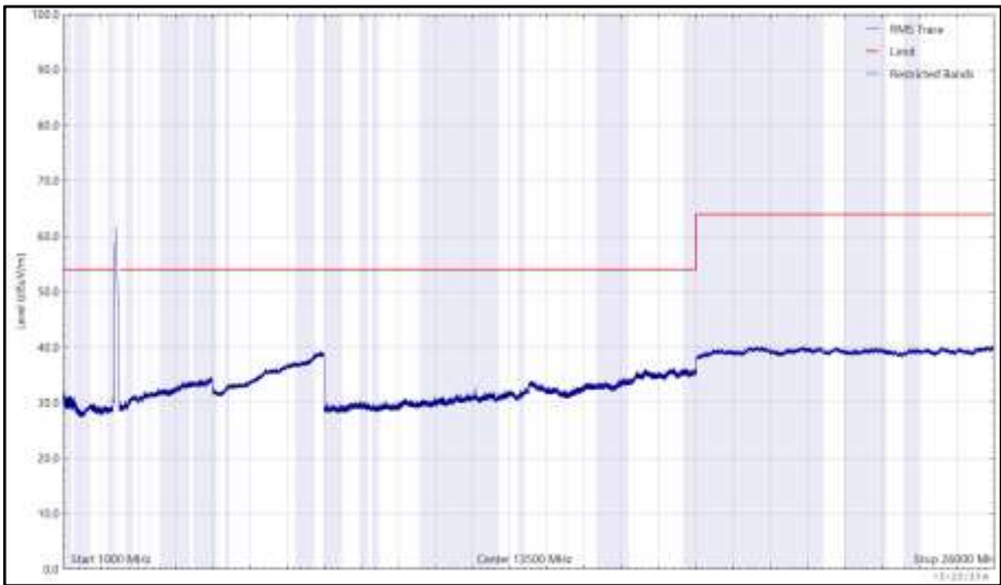
Figure 131 - 2412 MHz (CH1), 802.11g, Core 1, 1 GHz to 26 GHz, Horizontal (RMS)
