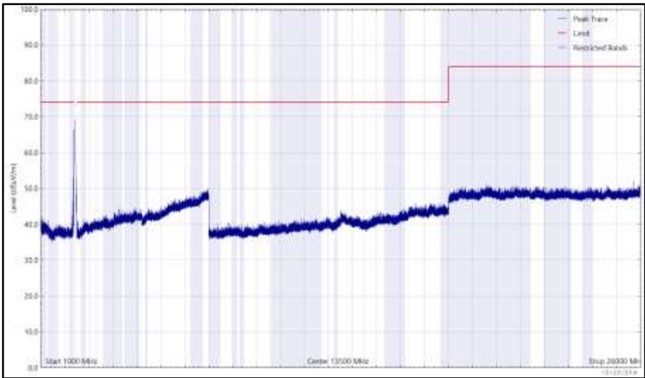
Figure 130 - 2412 MHz (CH1), 802.11g, Core 1, 1 GHz to 26 GHz, Horizontal (Peak)
