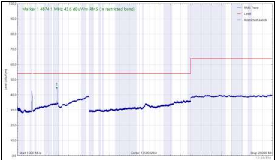
Figure 153 - 2437 MHz (CH6), 802.11b, Core 0, 1 GHz to 26 GHz, Vertical (RMS)
