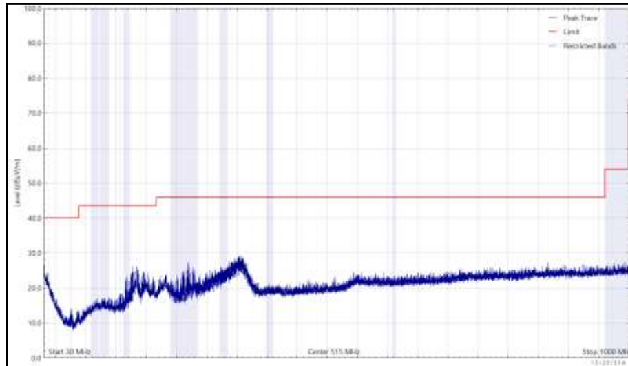
Figure 120 - 2437 MHz (CH6), 802.11g, Core 0, 30 MHz to 1 GHz, Horizontal (Peak)
