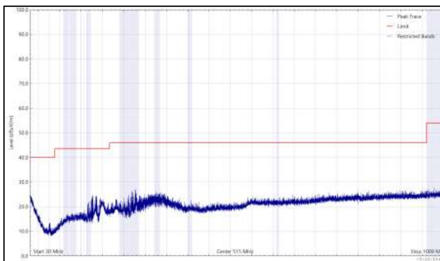
Figure 176 - 2437 MHz (CH6), HE20, RU26-0, Core 0 + Core 1, 30 MHz to 1 GHz, Horizontal (Peak)
