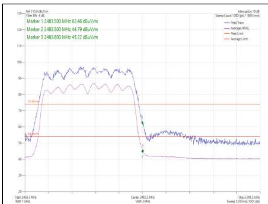
Figure 99 - 802.11ax HE20, Core 0-1, SU - 2472 MHz, Band Edge Frequency 2483.5 MHz
