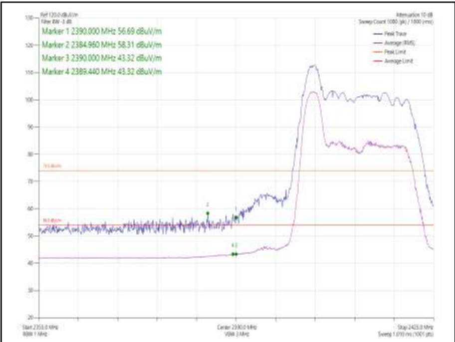
Figure 82 - 802.11ax HE20, Core 1, 26-0 - 2412 MHz, Band Edge Frequency 2390 MHz
