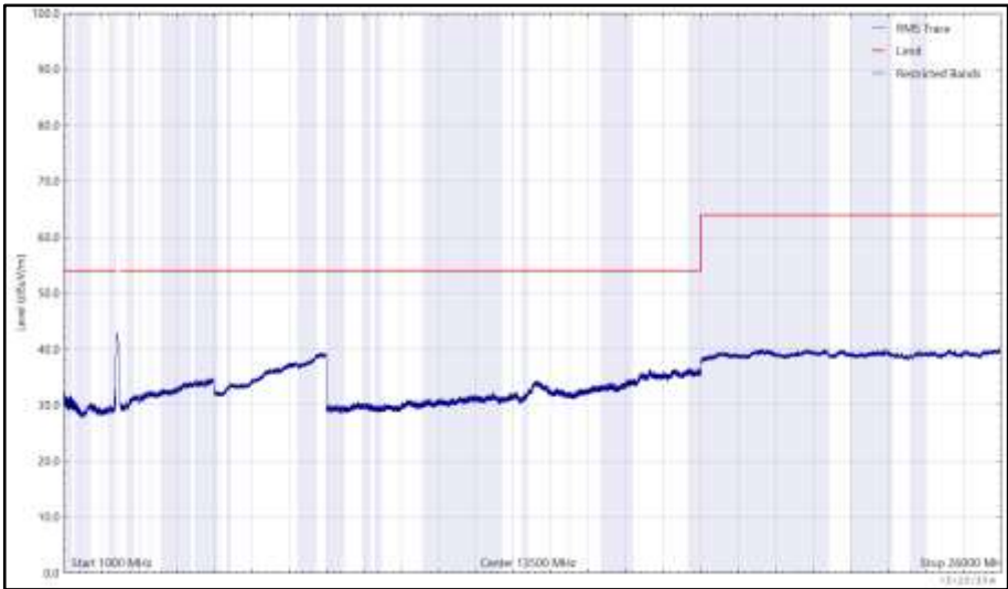
Figure 139 - 2437 MHz (CH6), 802.11g, Core 1, 1 GHz to 26 GHz, Vertical (RMS)
