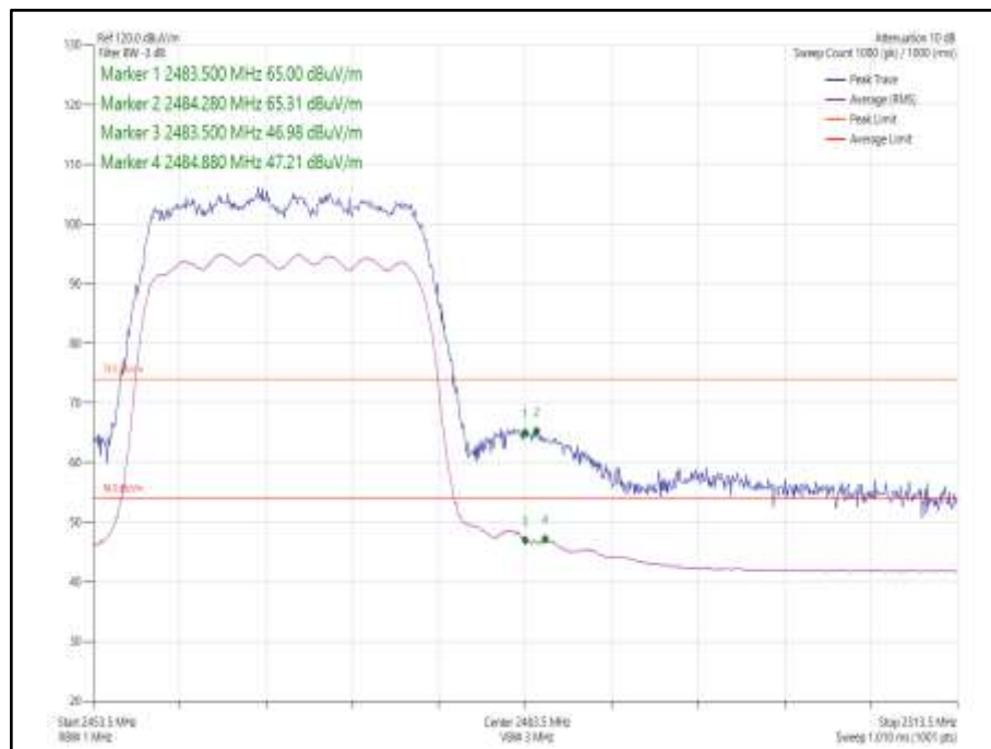
Figure 97 - 802.11ax HE20, Core 0-1, SU - 2467 MHz, Band Edge Frequency 2483.5 MHz
