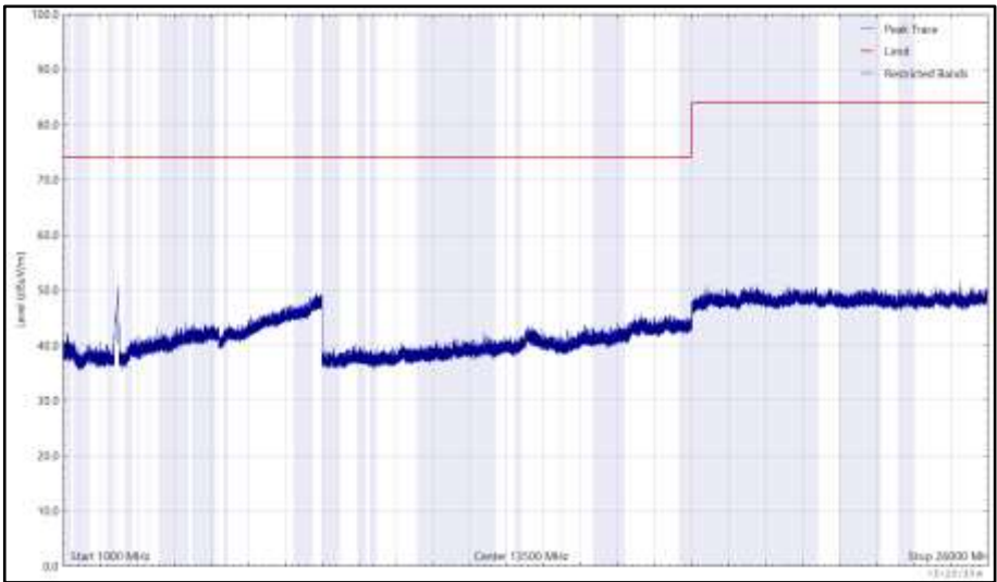
Figure 168 - 2472 MHz (CH13), 802.11b, Core 1, 1 GHz to 26 GHz, Horizontal (Peak)
