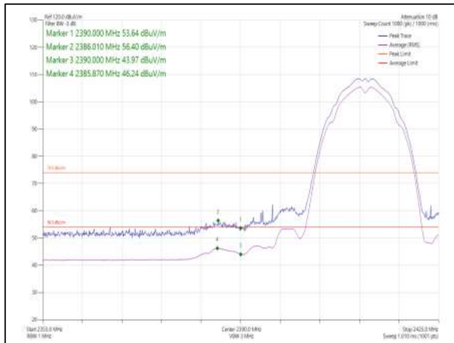
Figure 69 - 802.11b, Core 1 - 2412 MHz, Band Edge Frequency 2390.0 MHz
