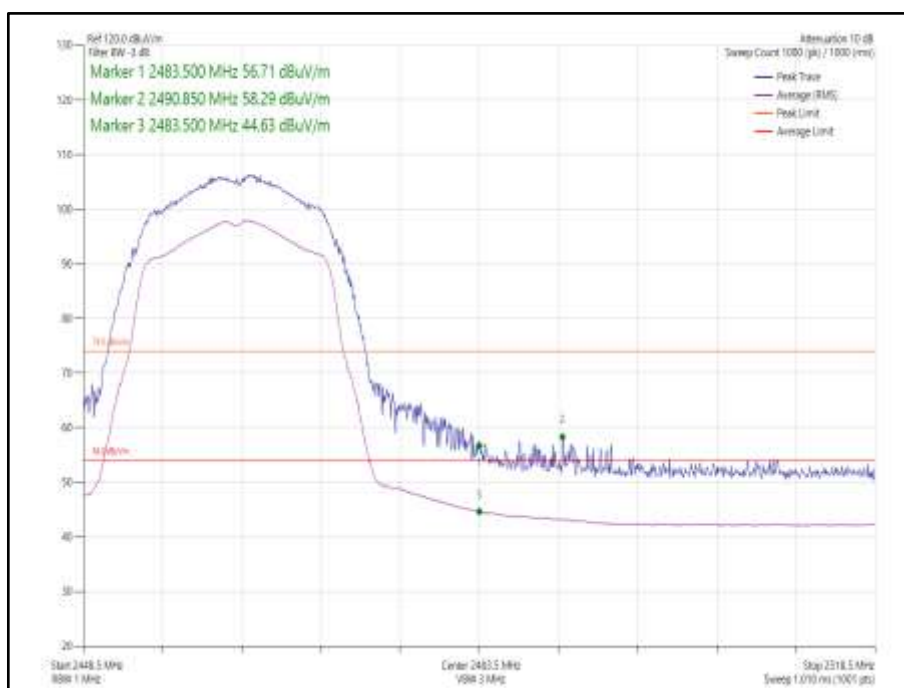
Figure 74 - 802.11g, Core 1 - 2462 MHz, Band Edge Frequency 2483.5 MHz
