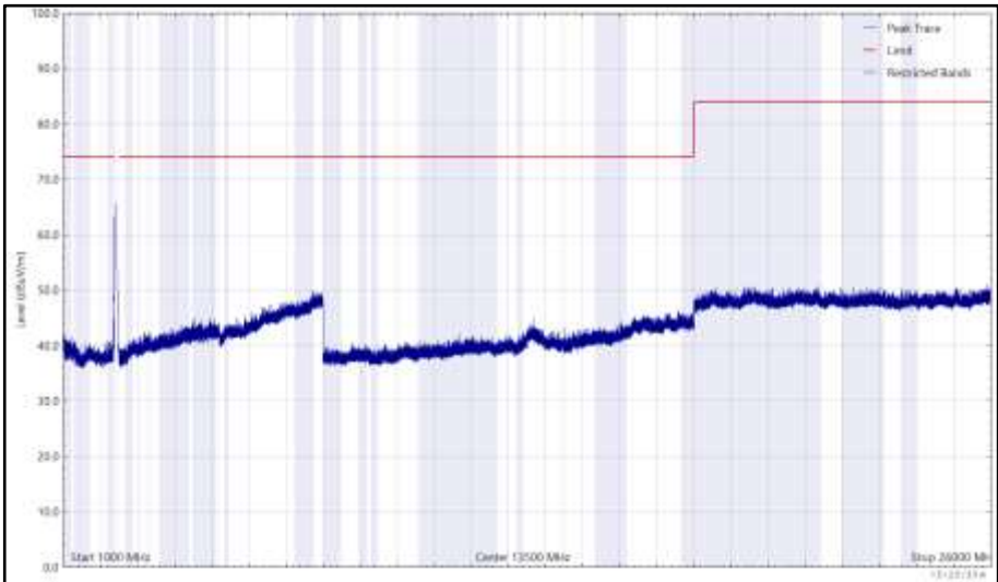
Figure 118 - 2412 MHz (CH1), 802.11g, Core 0, 1 GHz to 26 GHz, Vertical (Peak)
