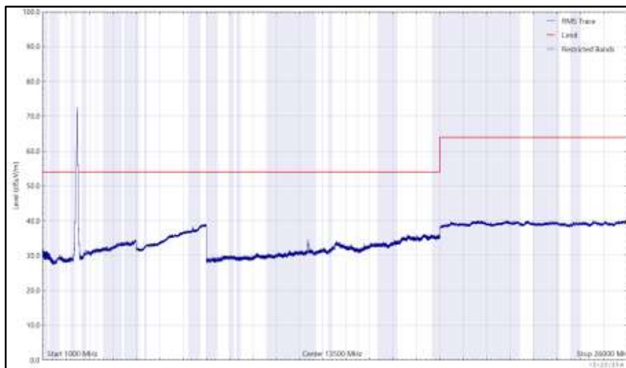
Figure 113 - 2472 MHz (CH13), HT20, CDD, Core 0 + Core 1, 1 GHz to 26 GHz, Horizontal (RMS)
