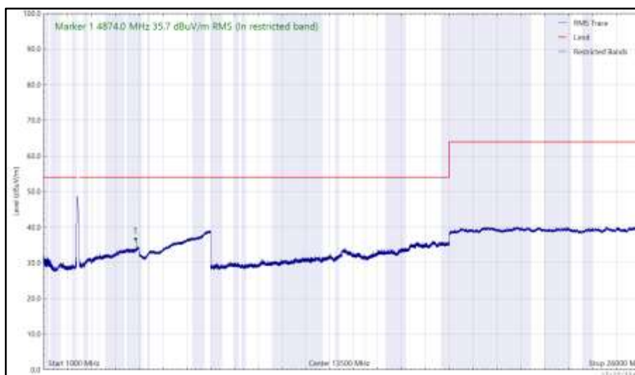
Figure 150 - 2437 MHz (CH6), 802.11b, Core 0, 1 GHz to 26 GHz, Horizontal (RMS)
