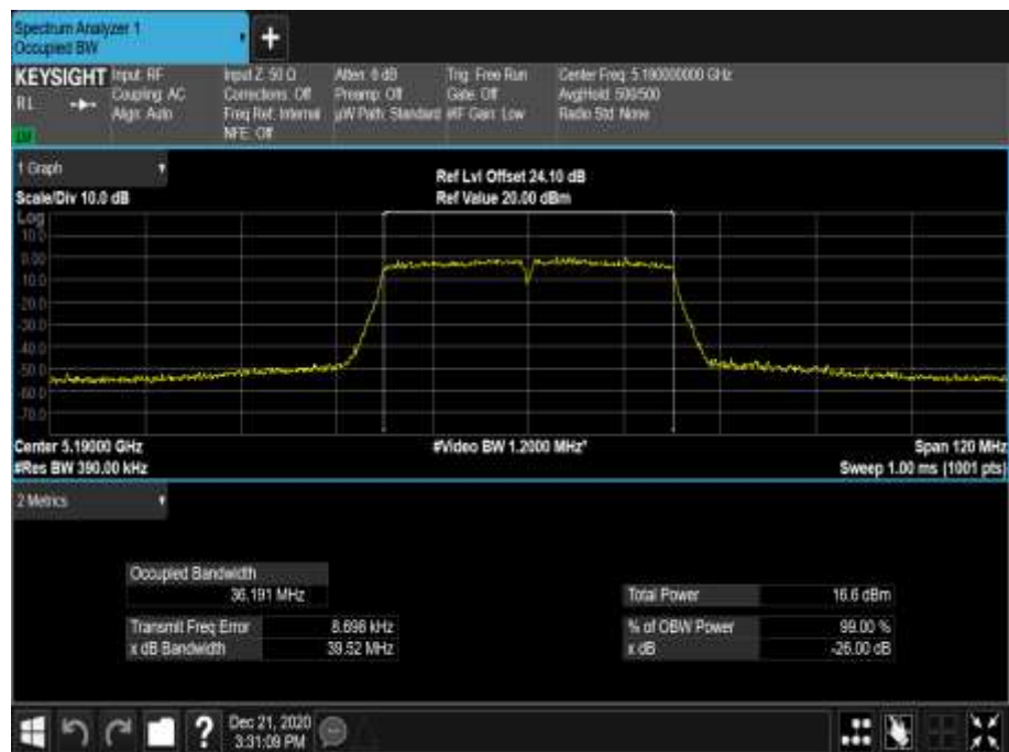
Figure 188 - 5190 MHz - 99% Occupied Bandwidth
