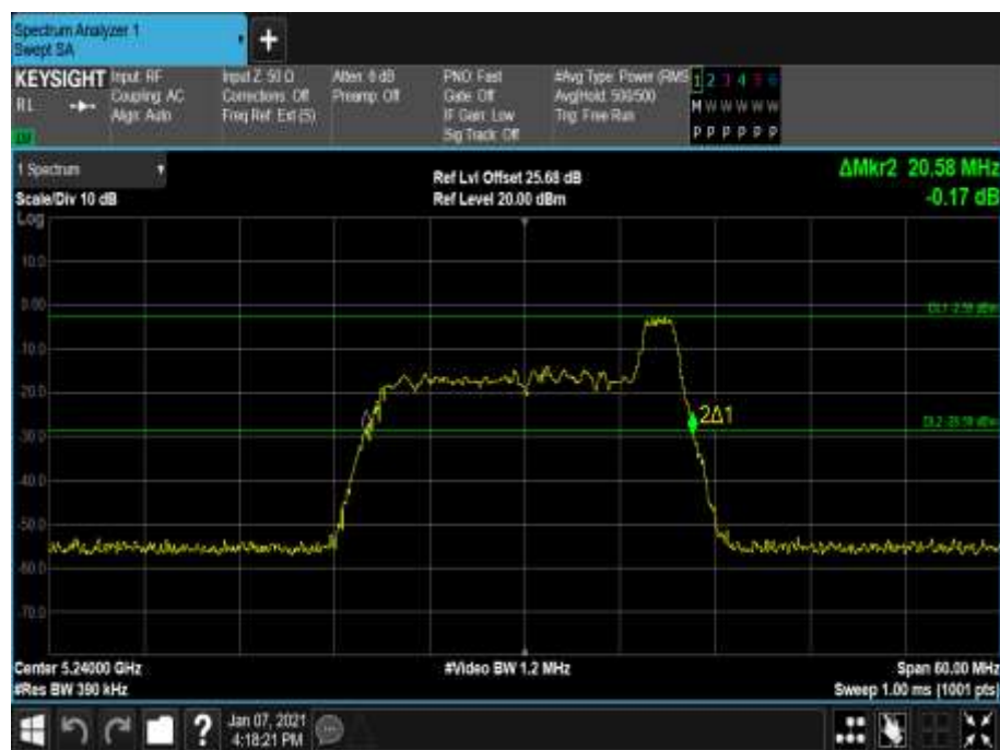
Figure 141 - 5240 MHz - 26 dB Emission Bandwidth
