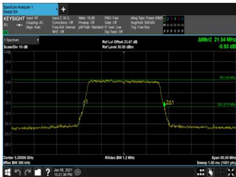
Figure 151 - 5200 MHz - 26 dB Emission Bandwidth
