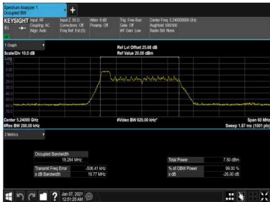
Figure 80 - 5240 MHz - 99% Occupied Bandwidth
