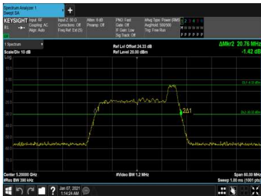
Figure 95 - 5200 MHz - 26 dB Emission Bandwidth
