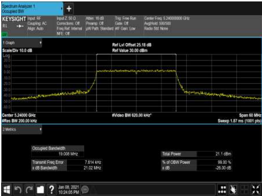
Figure 148 - 5240 MHz - 99% Occupied Bandwidth
