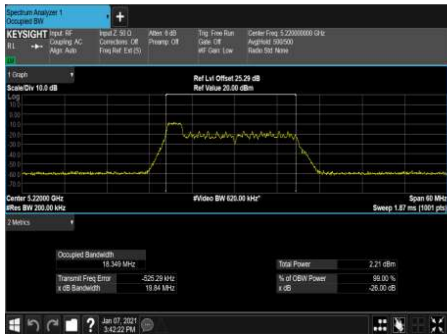
Figure 124 - 5220 MHz - 99% Occupied Bandwidth
