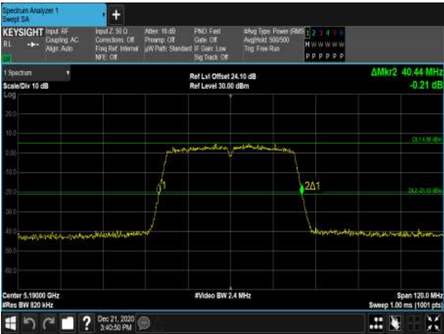
Figure 191 - 5190 MHz - 26 dB Emission Bandwidth
