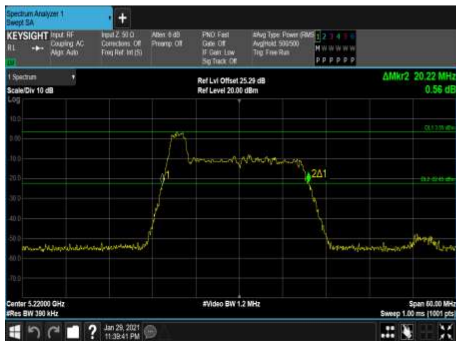
Figure 167 - 5220 MHz - 26 dB Emission Bandwidth
