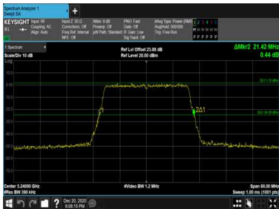
Figure 153 - 5240 MHz - 26 dB Emission Bandwidth
