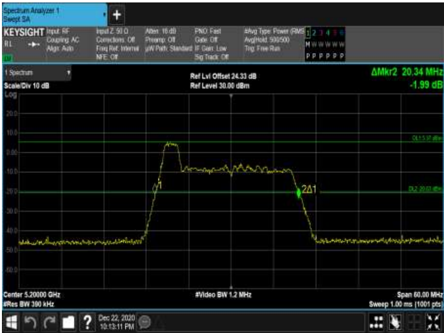
Figure 113 - 5200 MHz - 26 dB Emission Bandwidth
