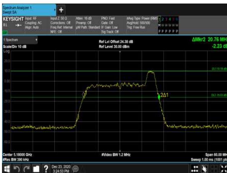
Figure 87 - 5180 MHz - 26 dB Emission Bandwidth
