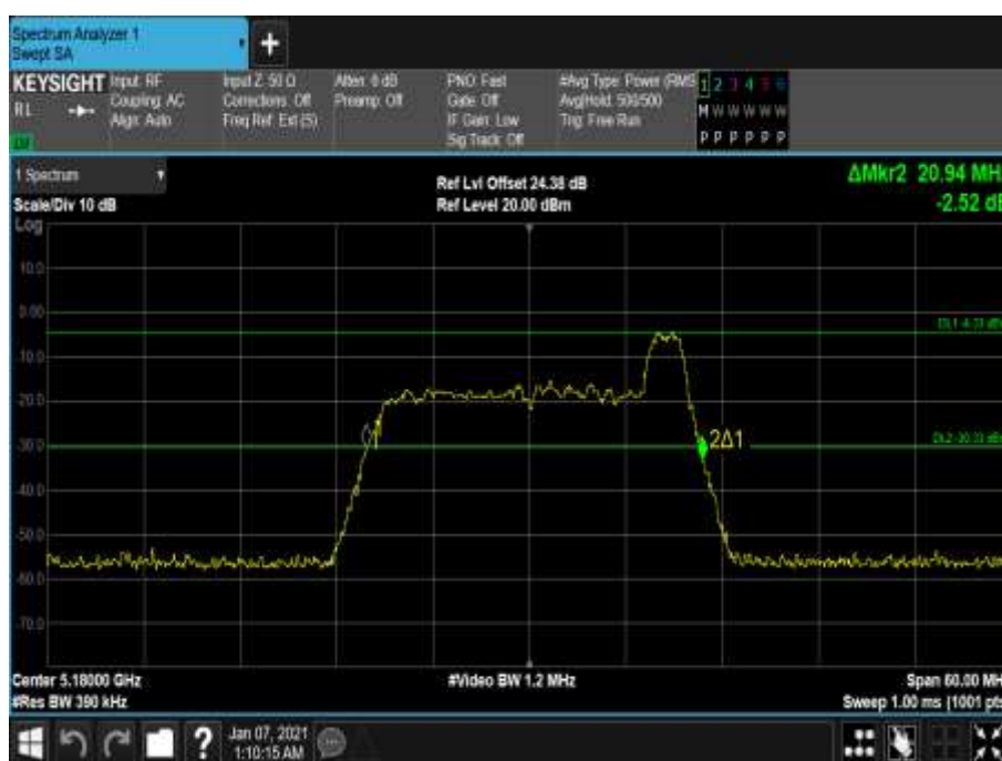
Figure 93 - 5180 MHz - 26 dB Emission Bandwidth
