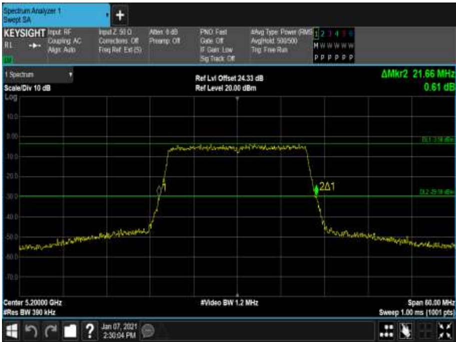
Figure 101 - 5200 MHz - 26 dB Emission Bandwidth
