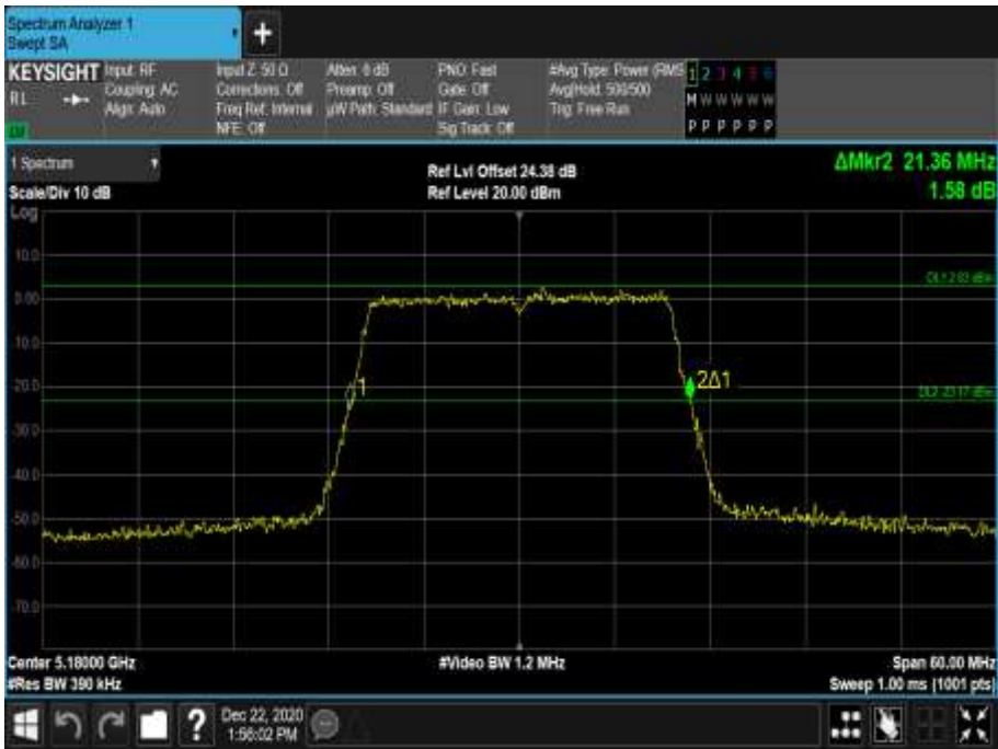
Figure 149 - 5180 MHz - 26 dB Emission Bandwidth
