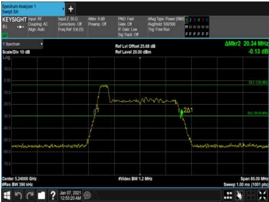
Figure 85 - 5240 MHz - 26 dB Emission Bandwidth
