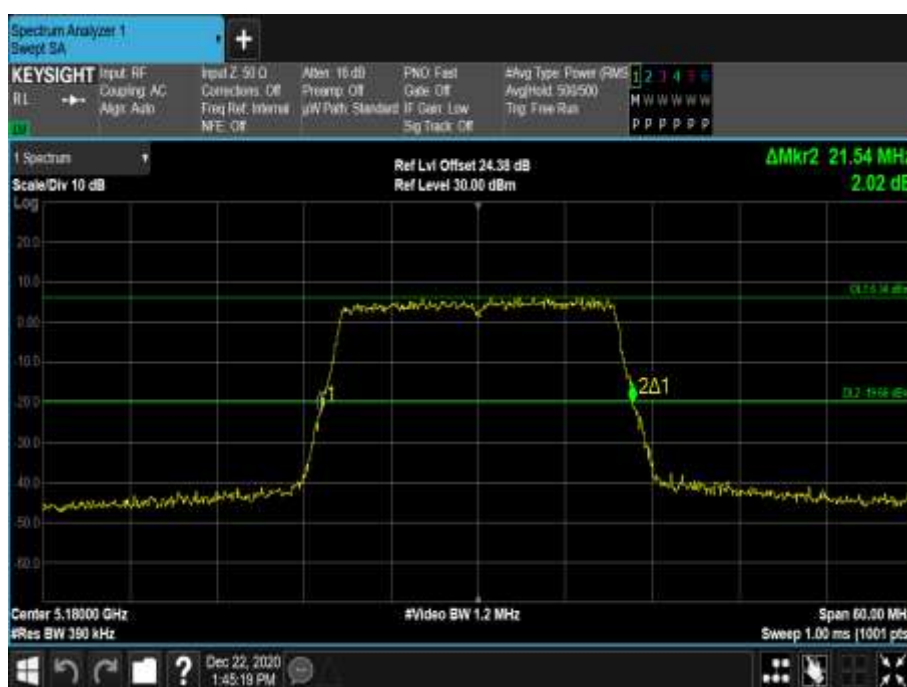
Figure 143 - 5180 MHz - 26 dB Emission Bandwidth
