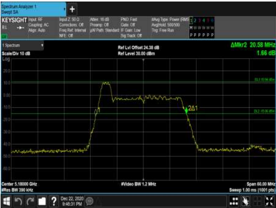
Figure 75 - 5180 MHz - 26 dB Emission Bandwidth
