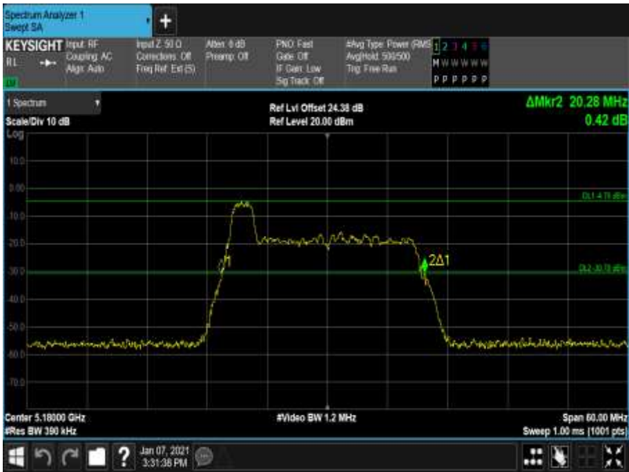
Figure 119 - 5180 MHz - 26 dB Emission Bandwidth
