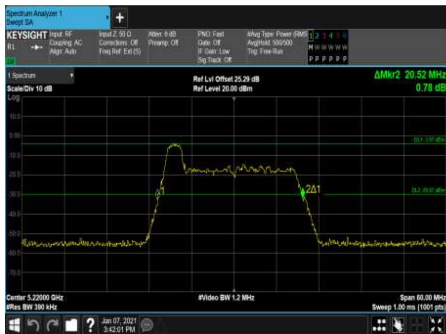
Figure 123 - 5220 MHz - 26 dB Emission Bandwidth
