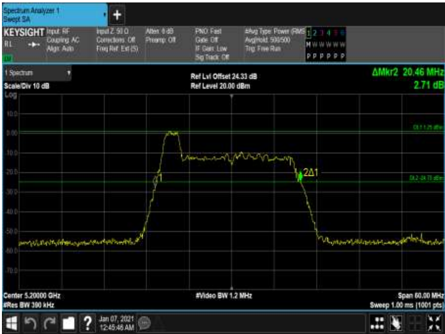
Figure 77 - 5200 MHz - 26 dB Emission Bandwidth
