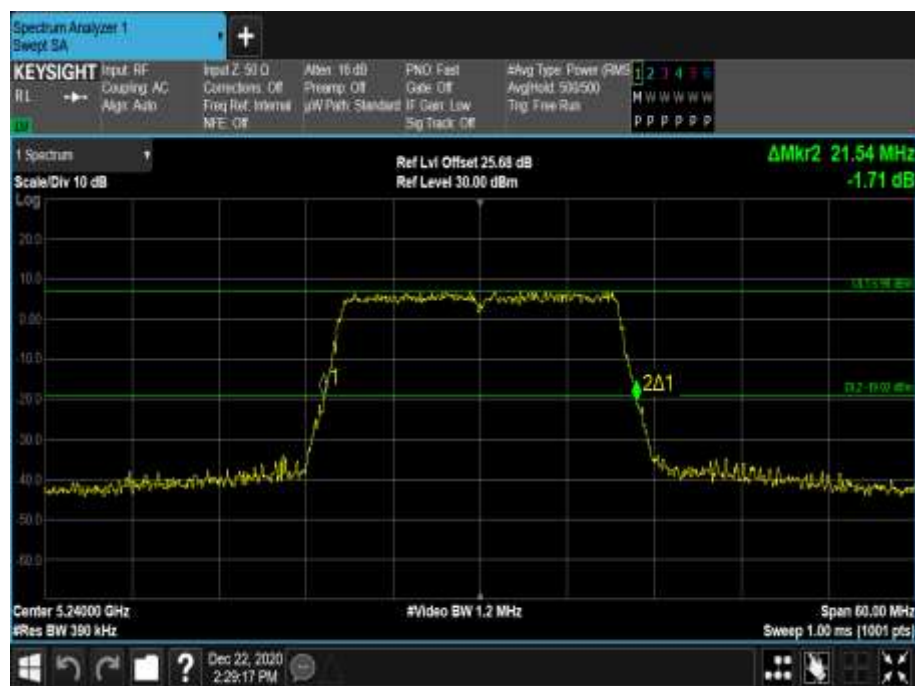
Figure 147 - 5240 MHz - 26 dB Emission Bandwidth
