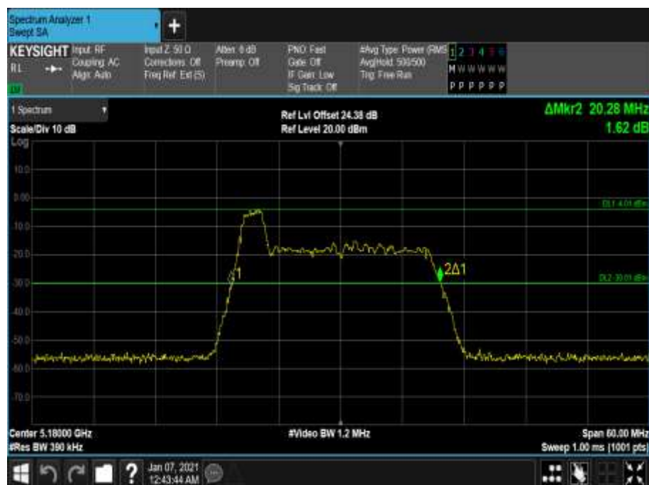
Figure 81 - 5180 MHz - 26 dB Emission Bandwidth
