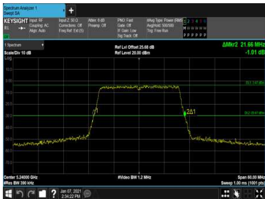
Figure 103 - 5240 MHz - 26 dB Emission Bandwidth
