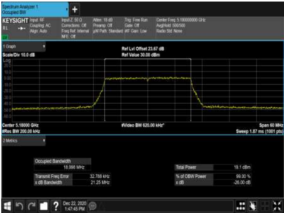
Figure 144 - 5180 MHz - 99% Occupied Bandwidth
