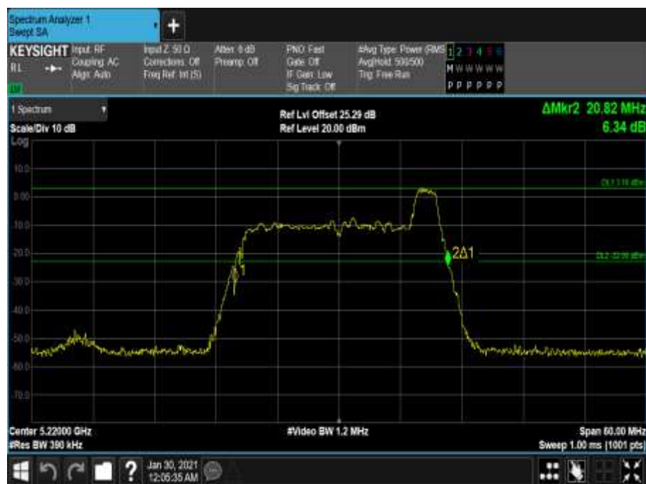
Figure 183 - 5220 MHz - 26 dB Emission Bandwidth
