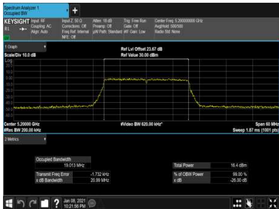
Figure 152 - 5200 MHz - 99% Occupied Bandwidth
