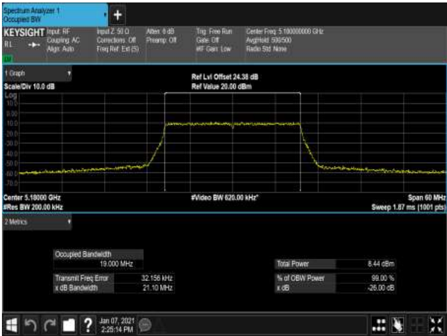
Figure 100 - 5180 MHz - 99% Occupied Bandwidth
