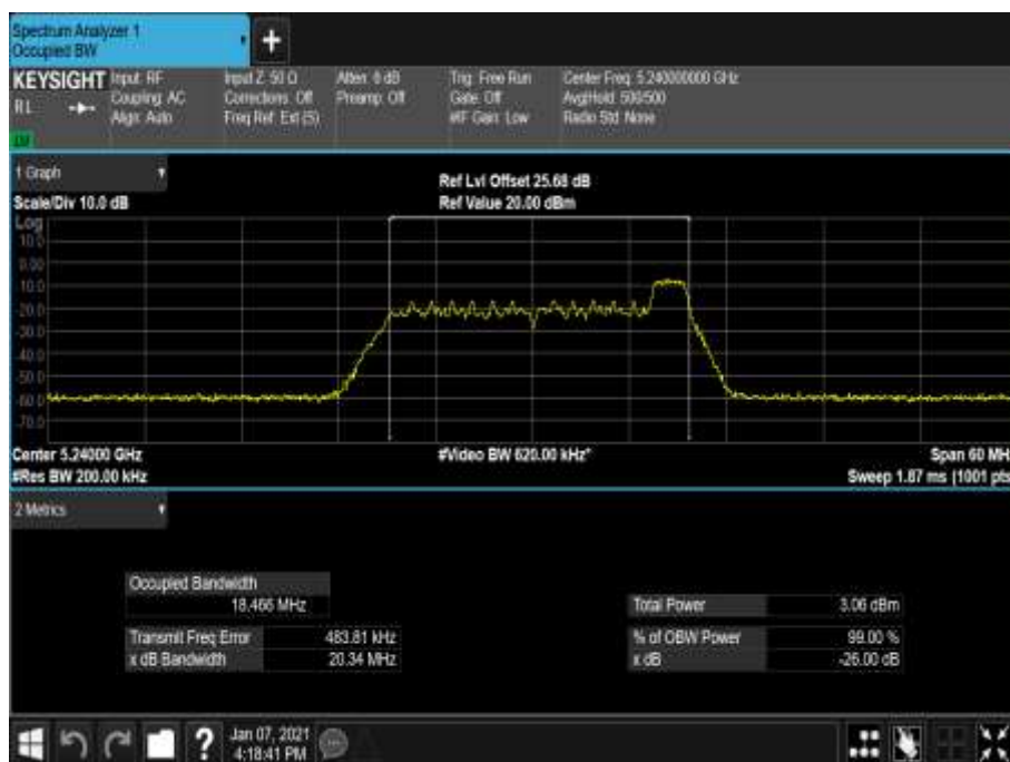
Figure 142 - 5240 MHz - 99% Occupied Bandwidth
