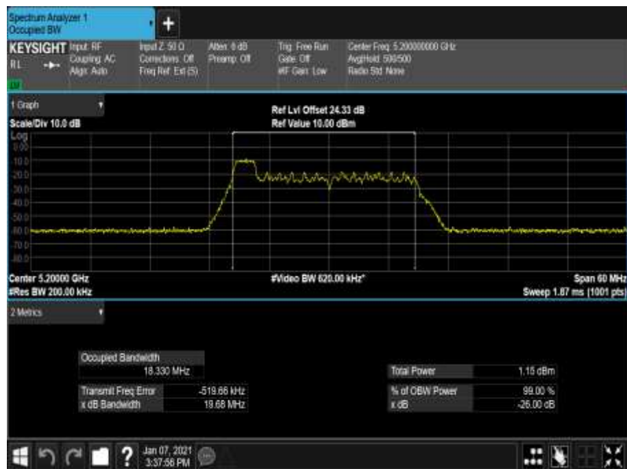
Figure 122 - 5200 MHz - 99% Occupied Bandwidth
