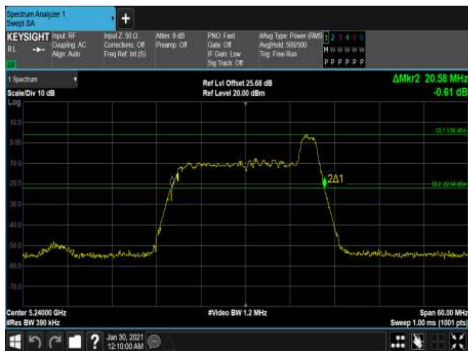
Figure 185 - 5240 MHz - 26 dB Emission Bandwidth
