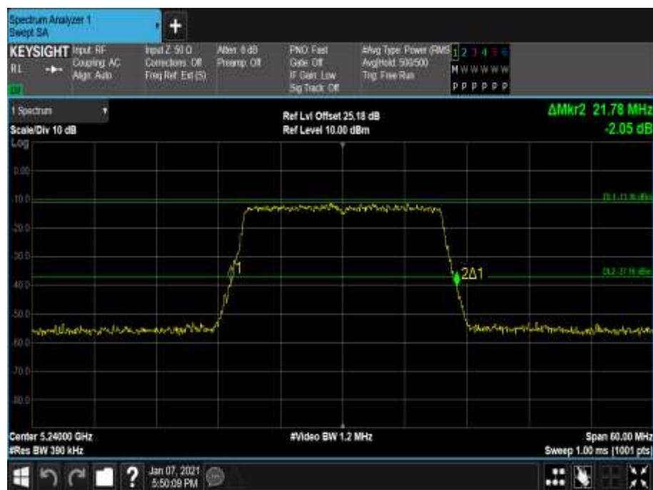
Figure 109 - 5240 MHz - 26 dB Emission Bandwidth
