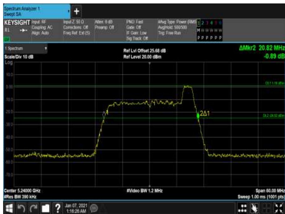
Figure 91 - 5240 MHz - 26 dB Emission Bandwidth
