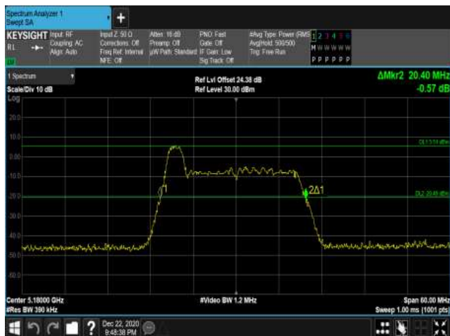
Figure 111 - 5180 MHz - 26 dB Emission Bandwidth
