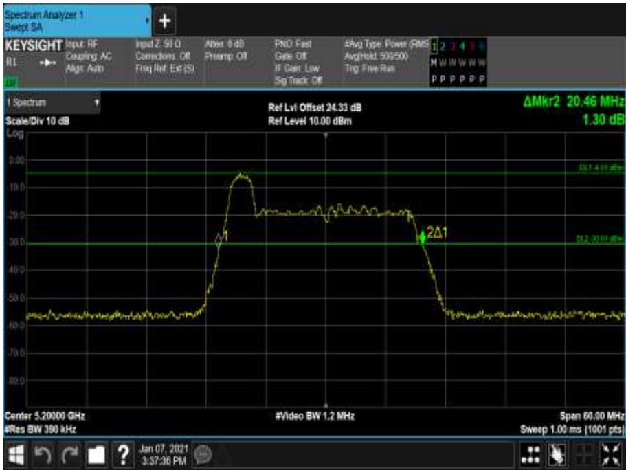
Figure 121 - 5200 MHz - 26 dB Emission Bandwidth
