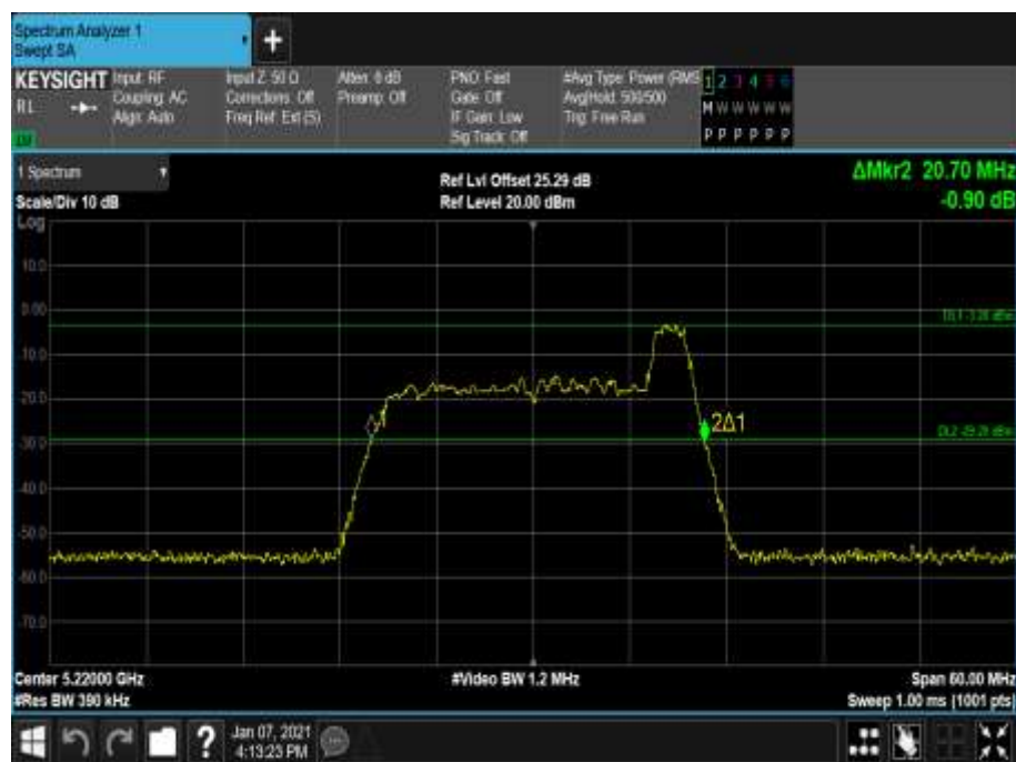
Figure 139 - 5220 MHz - 26 dB Emission Bandwidth
