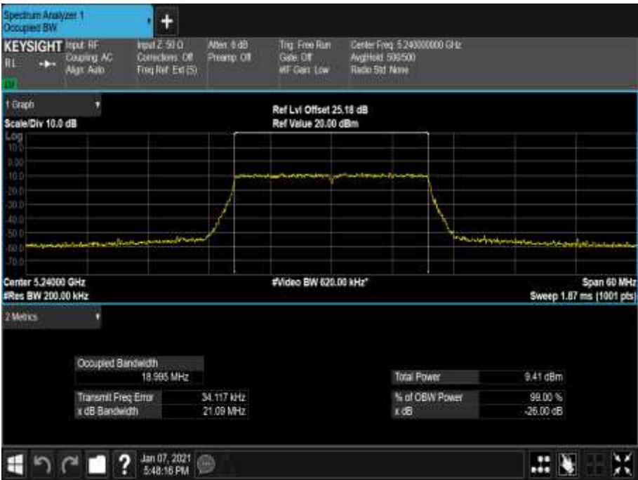
Figure 104 - 5240 MHz - 99% Occupied Bandwidth
