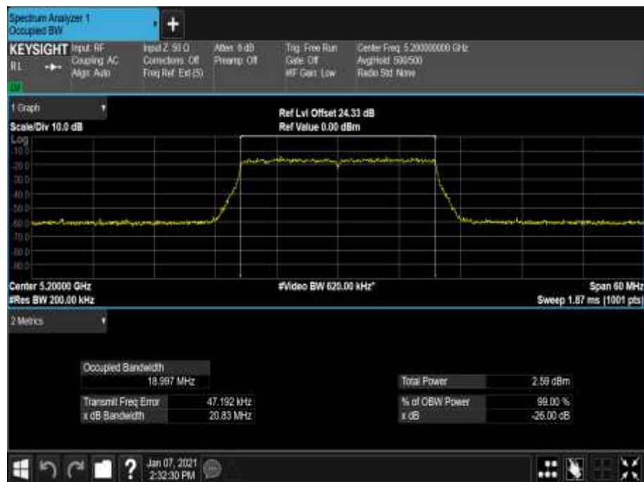
Figure 108 - 5200 MHz - 99% Occupied Bandwidth
