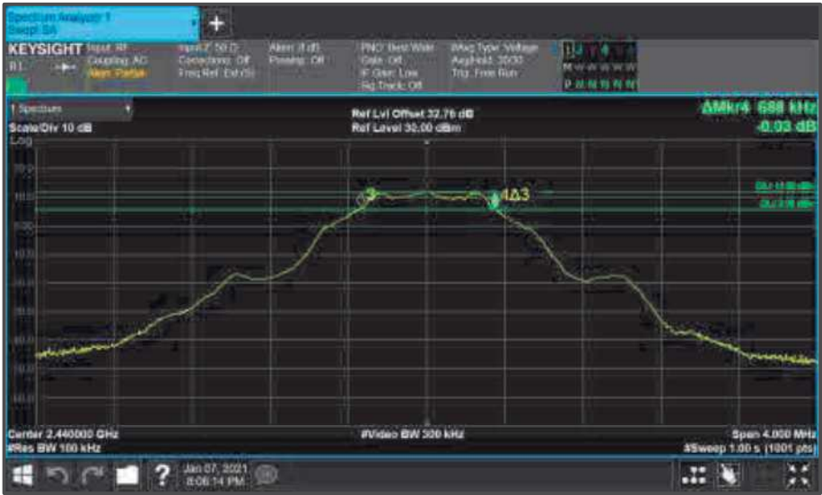
Figure 54 - Core1 (B) 2440 MHz (CH19) 6 dB Bandwidth
