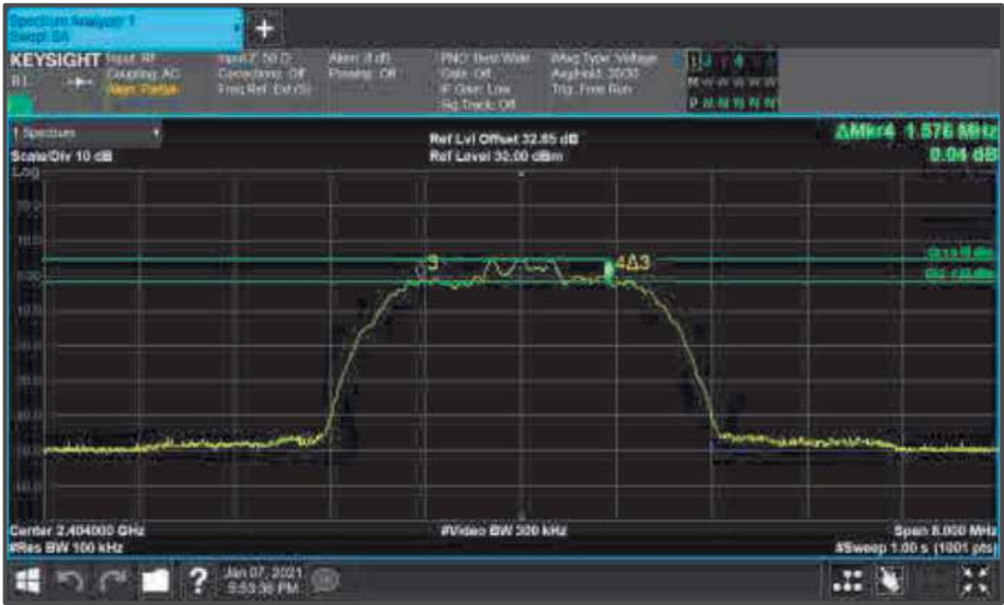
Figure 100 - Core0 (C) 2404 MHz (CH2) 6 dB Bandwidth
