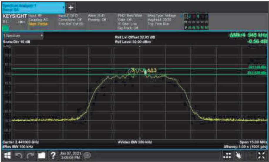
Figure 82 - Core2 (A) 2441 MHz (CH39) 6 dB Bandwidth
