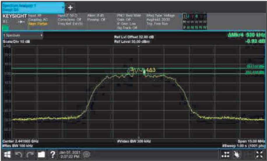
Figure 94 - Core0 (C) 2441 MHz (CH39) 6 dB Bandwidth
