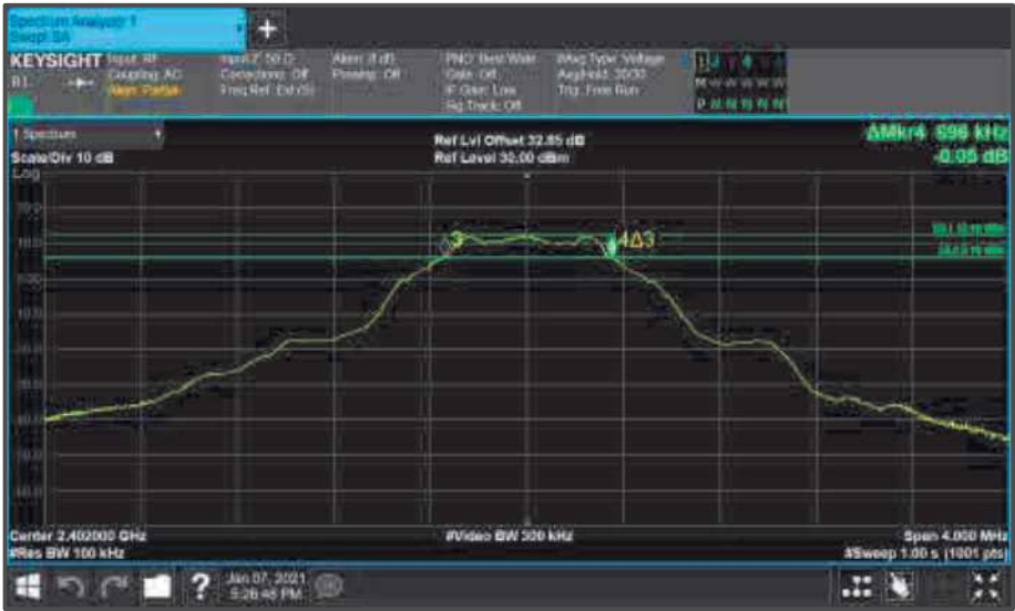
Figure 38 - Core0 (C) 2402 MHz (CH0) 6 dB Bandwidth
