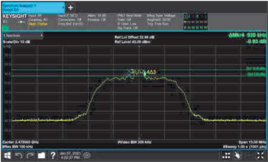
Figure 12 - Core0 (C) 2478 MHz (CH76) 6 dB Bandwidth
