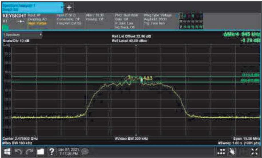
Figure 36 - Core0 (C) 2478 MHz (CH76) 6 dB Bandwidth
