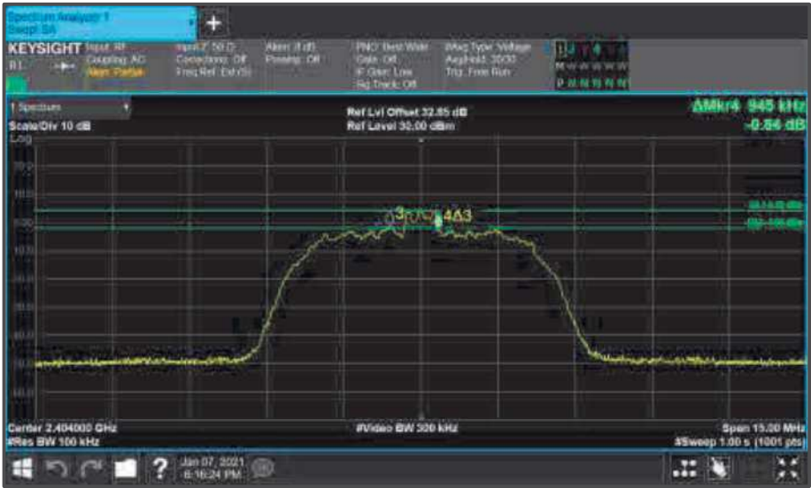
Figure 112 - Core0 (C) 2404 MHz (CH2) 6 dB Bandwidth
