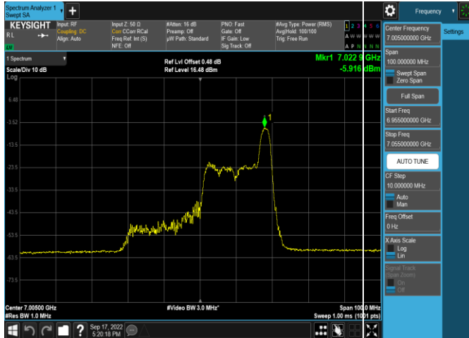
Plot 7-365. Power Spectral Density Plot SDM Antenna 5b (40MHz 802.11ax RU26 (UNII Band 8) – Ch. 211)
