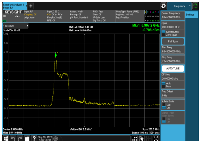
Plot 7-370. Power Spectral Density Plot SDM Antenna 4a (80MHz 802.11ax RU26 (UNII Band 8) – Ch. 199)
