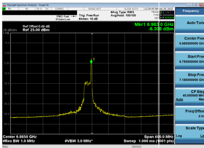
Plot 7-379. Power Spectral Density Plot SDM Antenna 5b (160MHz 802.11ax RU26 (UNII Band 8) – Ch. 207)
