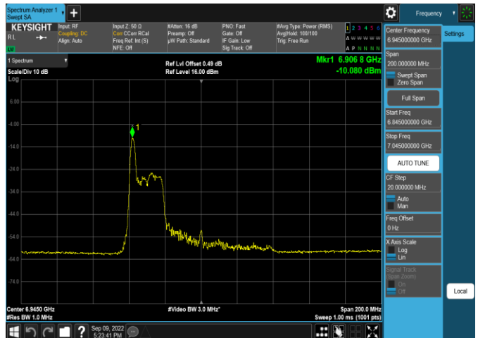
Plot 7-369. Power Spectral Density Plot SDM Antenna 5b (80MHz 802.11ax RU26 (UNII Band 8) – Ch. 199)
