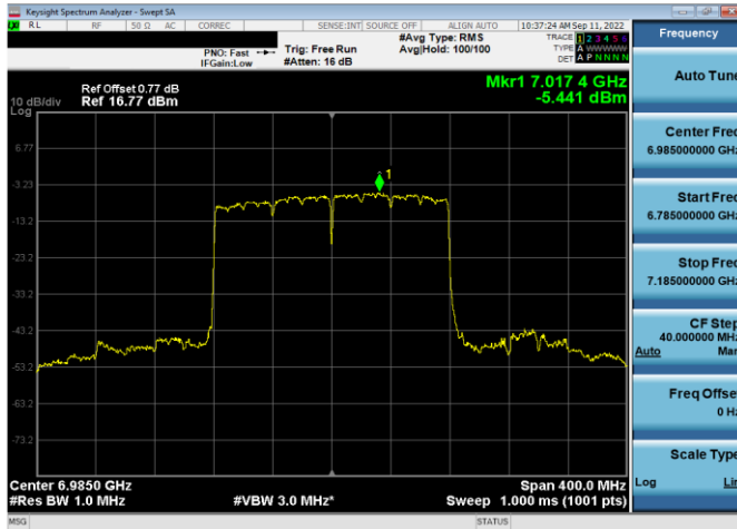
Plot 7-383. Power Spectral Density Plot SDM Antenna 5b (160MHz 802.11ax RU996x2 (UNII Band 8) – Ch. 207)
