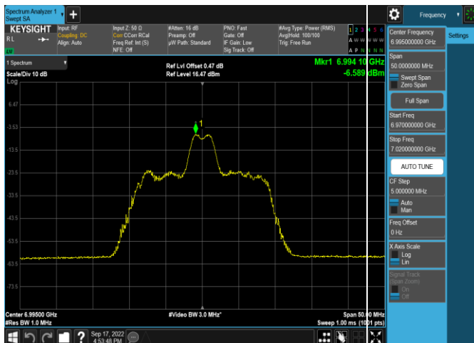
Plot 7-355. Power Spectral Density Plot SDM Antenna 5b (20MHz 802.11ax RU26 (UNII Band 8) – Ch. 209)
