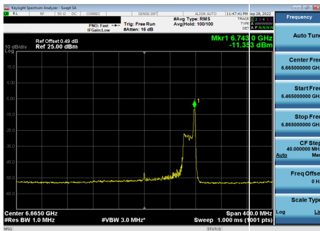
Plot 7-349. Power Spectral Density Plot SDM Antenna 5b (160MHz 802.11ax RU26 (UNII Band 7) – Ch. 143)
