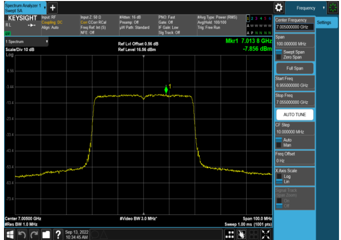
Plot 7-368. Power Spectral Density Plot SDM Antenna 4a (40MHz 802.11ax RU484 (UNII Band 8) – Ch. 211)
