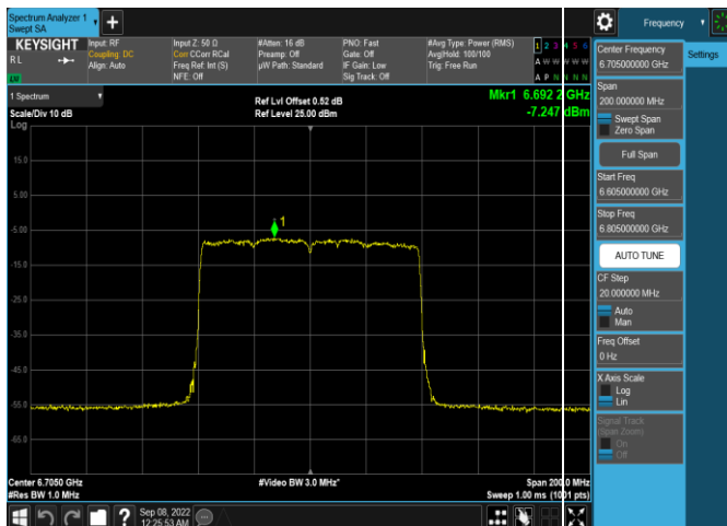
Plot 7-343. Power Spectral Density Plot SDM Antenna 5b (80MHz 802.11ax RU996 (UNII Band 7) – Ch. 151)
