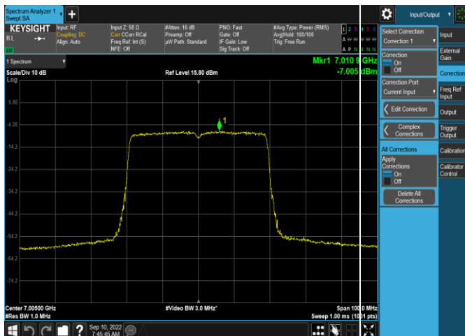
Plot 7-367. Power Spectral Density Plot SDM Antenna 5b (40MHz 802.11ax RU484 (UNII Band 8) – Ch. 211)
