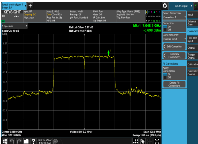
Plot 7-384. Power Spectral Density Plot SDM Antenna 4a (160MHz 802.11ax RU996x2 (UNII Band 8) – Ch. 207)
