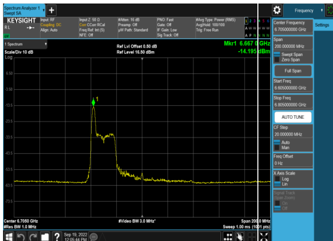
Plot 7-337. Power Spectral Density Plot SDM Antenna 5b (80MHz 802.11ax RU26 (UNII Band 7) – Ch. 151)
