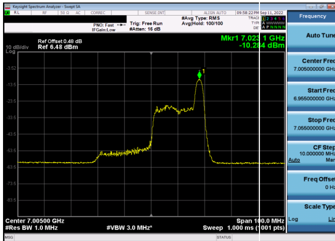
Plot 7-366. Power Spectral Density Plot SDM Antenna 4a (40MHz 802.11ax RU26 (UNII Band 8) – Ch. 211)
