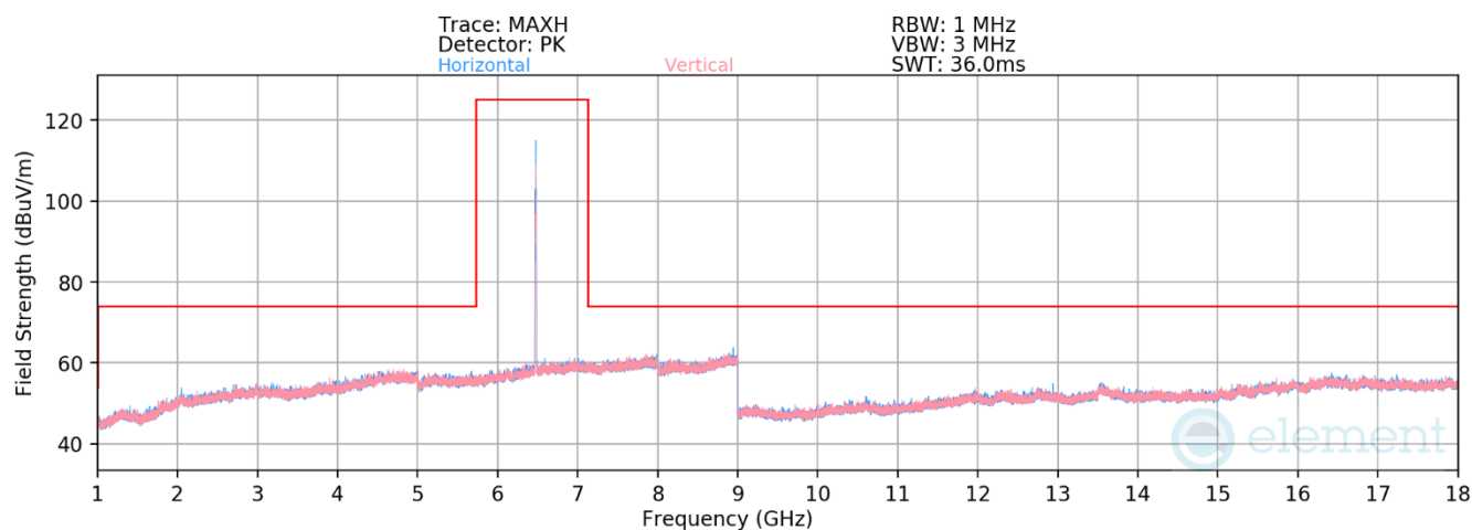
Plot 7-2. Radiated Spurious Emissions above 1GHz SDM (802.11ax – Ch. 105 – RU26)
