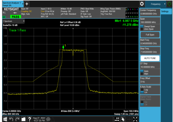
Plot 7-456. In-Band Emission Plot Antenna 4a (20MHz 802.11ax (UNII Band 8) – Ch. 209, MCS11)
