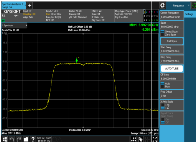
Plot 7-338. Power Spectral Density Plot SDM Antenna 4a (20MHz 802.11ax (UNII Band 8) – Ch. 209, MCS11)
