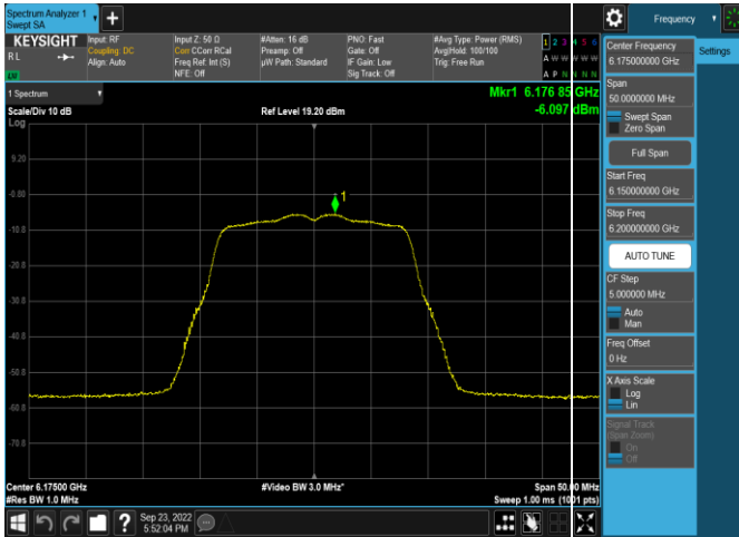
Plot 7-185. Power Spectral Density Plot Antenna 4a (20MHz 802.11a (UNII Band 5) – Ch. 45, MCS2)
