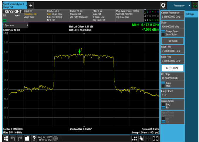
Plot 7-229. Power Spectral Density Plot Antenna 4a (160MHz 802.11ax (UNII Band 5) – Ch. 47, MCS11)
