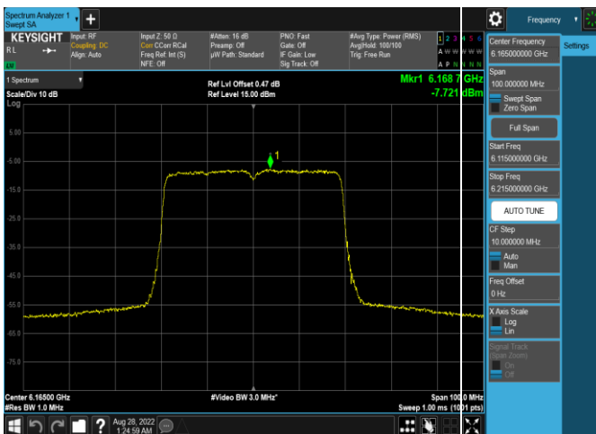
Plot 7-207. Power Spectral Density Plot Antenna 4a (40MHz 802.11ax (UNII Band 5) – Ch. 43, MCS4)
