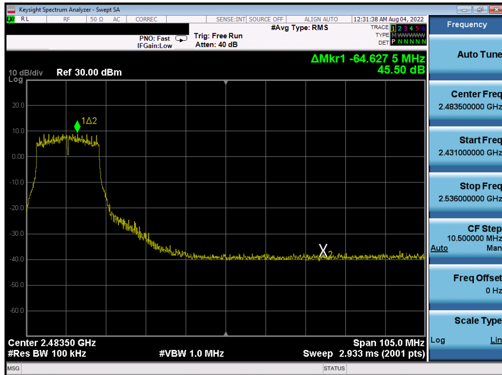
Plot 7-389. Band Edge Plot Antenna 2a (802.11g- Ch. 7) – 36Mbps
