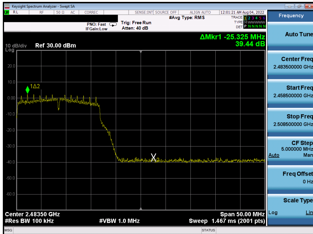
Plot 7-345. Band Edge Plot Antenna 2a (802.11g – Ch. 12) – 18Mbps
