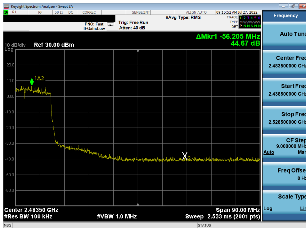
Plot 7-328. Band Edge Plot Antenna 2a (802.11ax (SU - 2.4GHz) – Ch. 7) – MCS2
