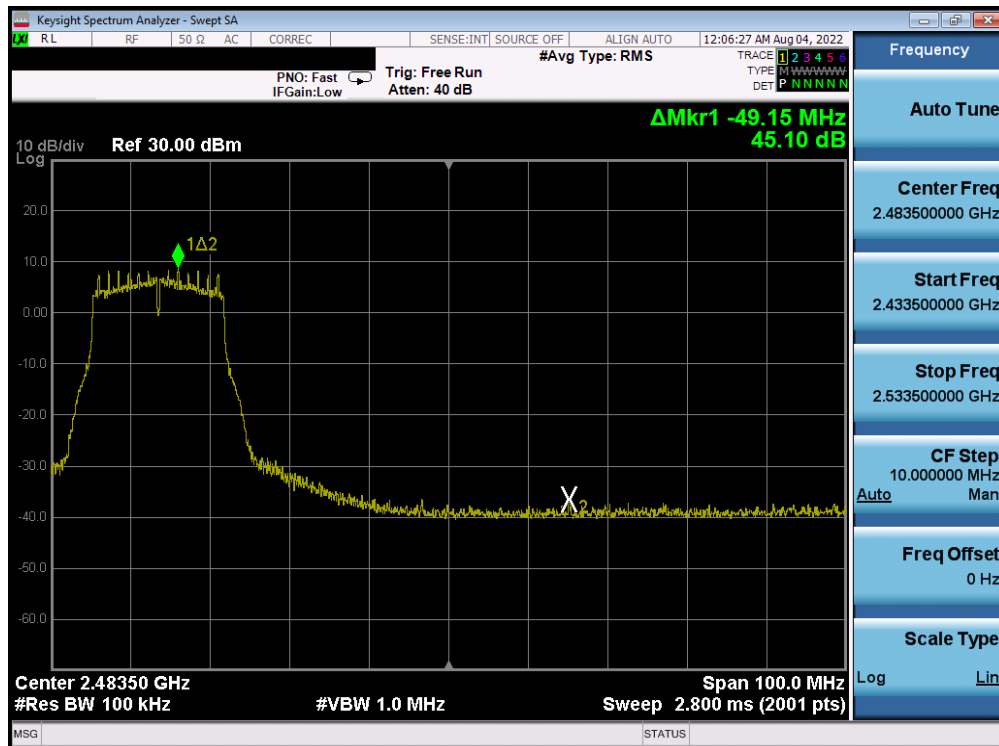
Plot 7-341. Band Edge Plot Antenna 2a (802.11g- Ch. 8) – 18Mbps
