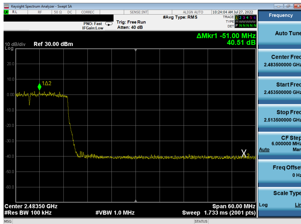
Plot 7-420. Band Edge Plot Antenna 2a (802.11ax (SU - 2.4GHz) – Ch. 10) – MCS5
