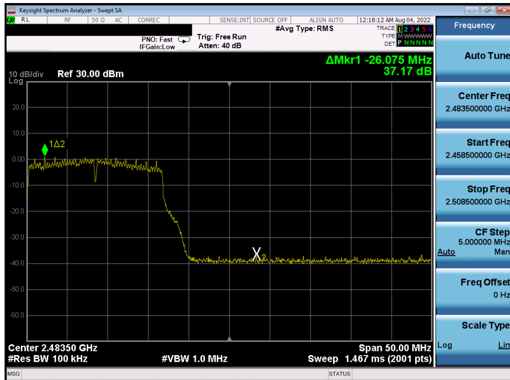
Plot 7-394. Band Edge Plot Antenna 2a (802.11g - Ch. 12) - 36Mbps
