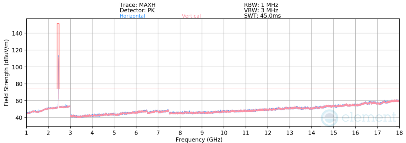
Plot 7-437. Radiated Spurious Emissions above 1GHz Antenna 4a (802.11b – Ch. 11)
