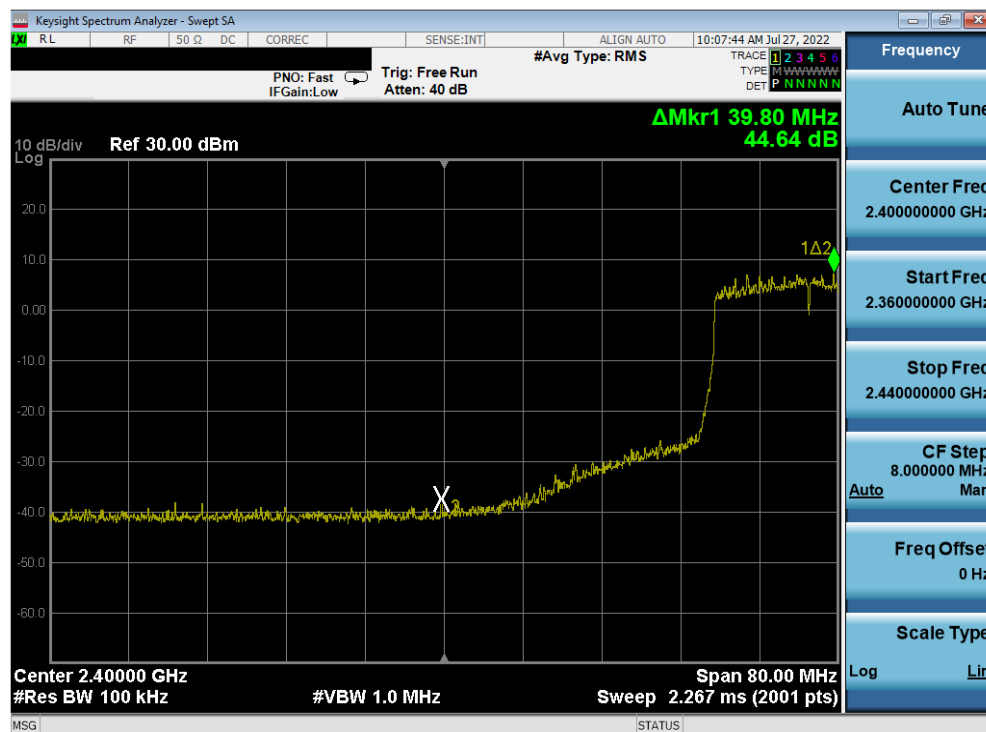
Plot 7-365. Band Edge Plot Antenna 2a (802.11ax (SU - 2.4GHz) – Ch. 6 (low)) – MCS3
