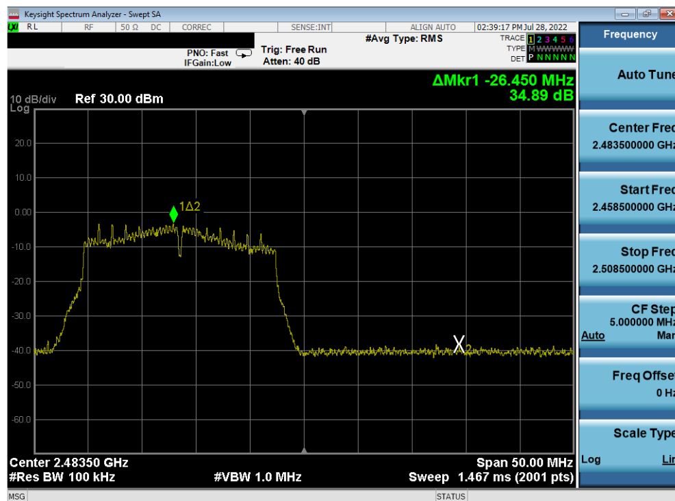
Plot 7-359. Band Edge Plot Antenna 2a (802.11n (2.4GHz) - Ch. 13) - MCS3
