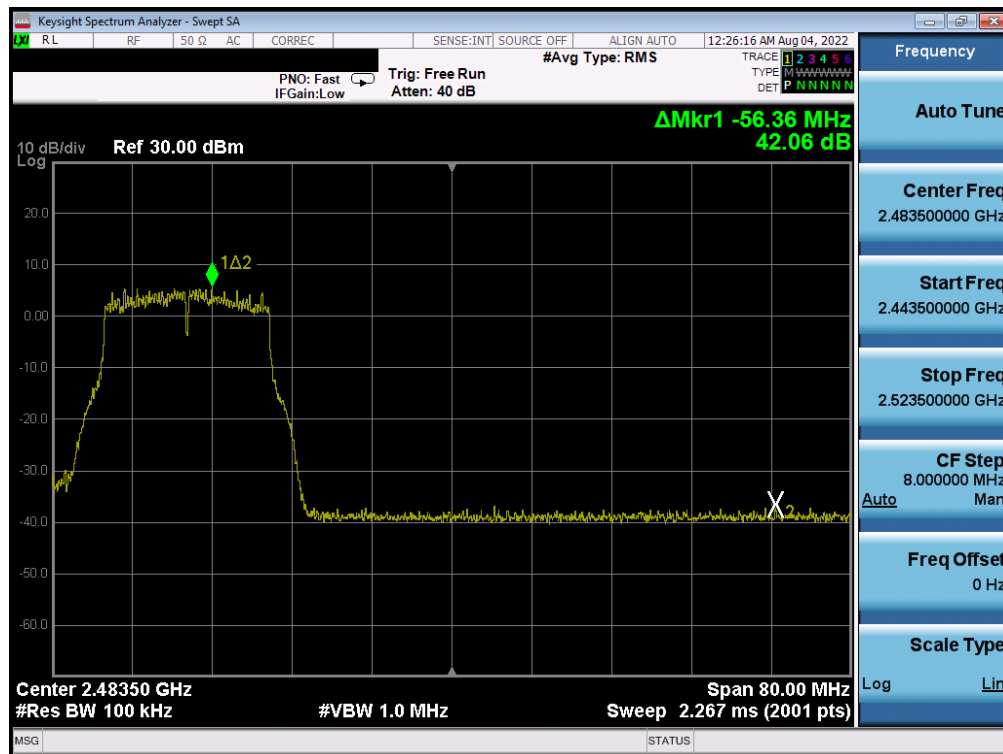
Plot 7-392. Band Edge Plot Antenna 2a (802.11g – Ch. 10) – 36Mbps
