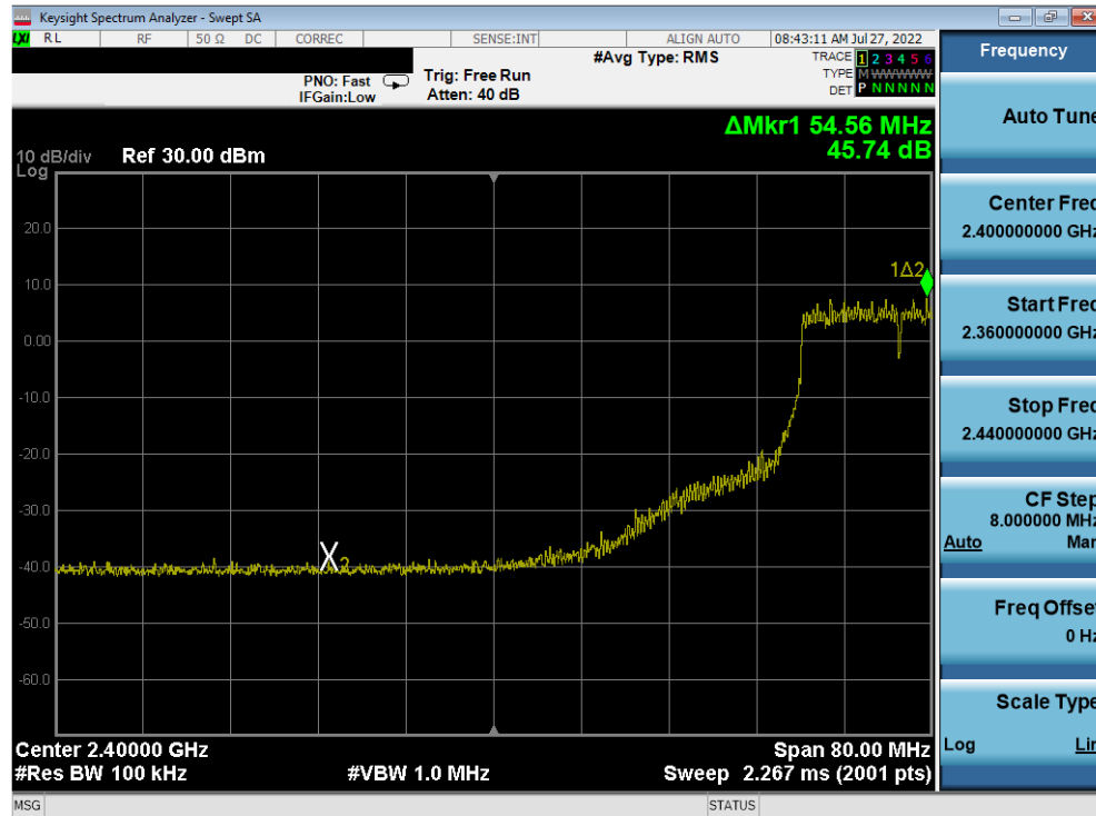
Plot 7-401. Band Edge Plot Antenna 2a (802.11n (2.4GHz) – Ch. 6 (low)) – MCS5
