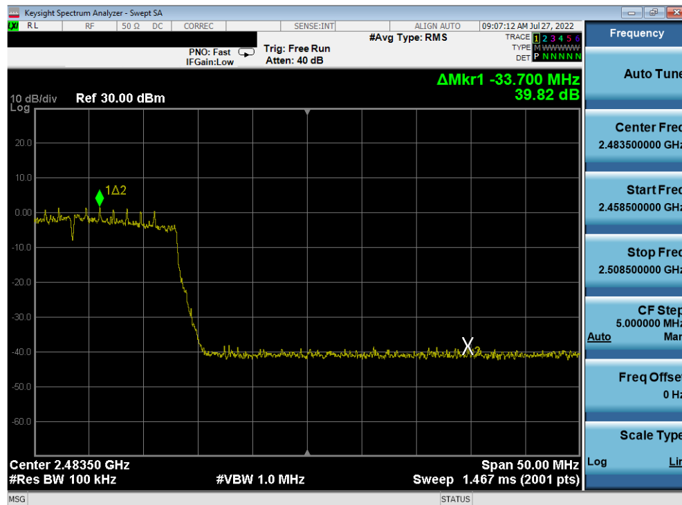
Plot 7-332. Band Edge Plot Antenna 2a (802.11ax (SU - 2.4GHz) – Ch. 11) – MCS2
