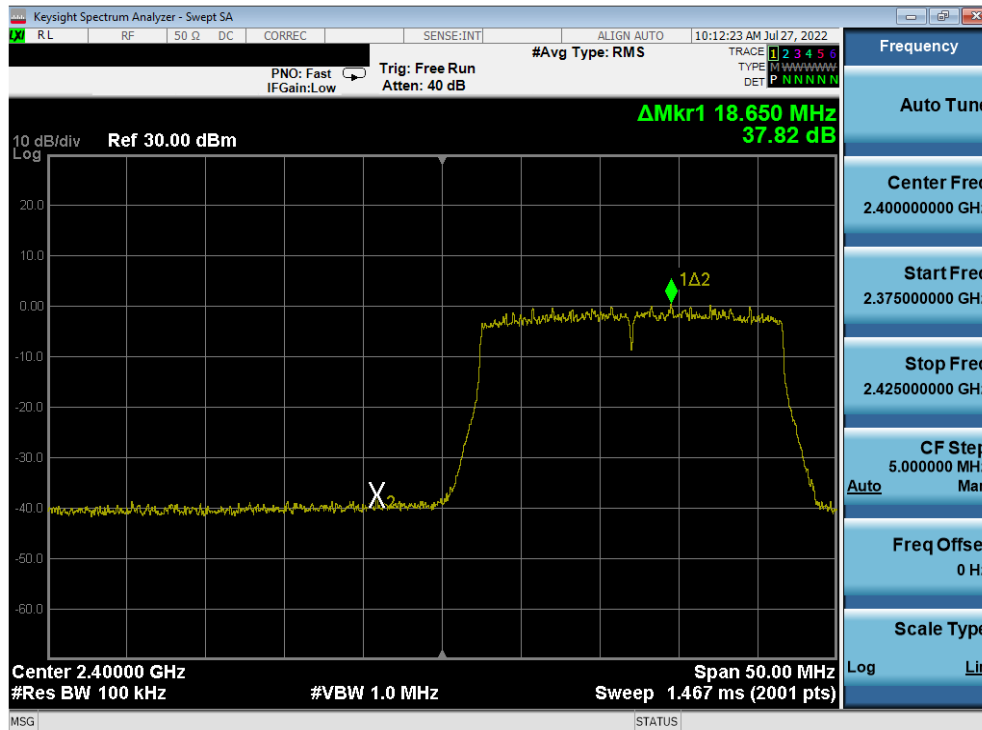
Plot 7-410. Band Edge Plot Antenna 2a (802.11ax (SU - 2.4GHz) – Ch. 1) – MCS5
