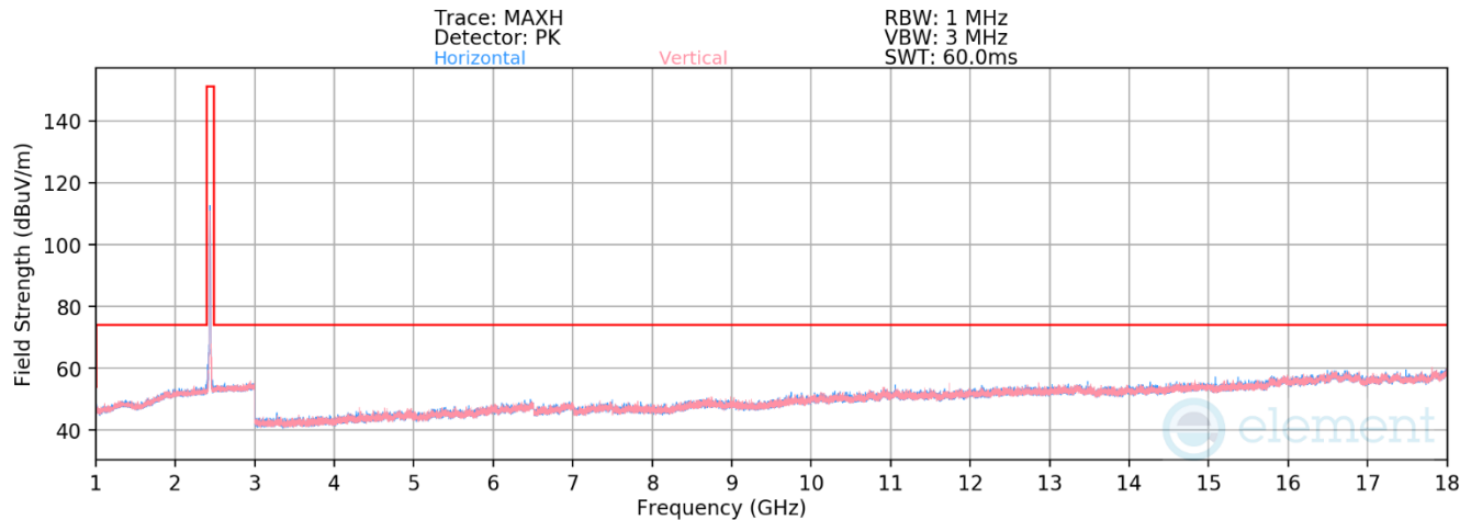
Plot 7-436. Radiated Spurious Emissions above 1GHz Antenna 4a (802.11b – Ch. 6)
