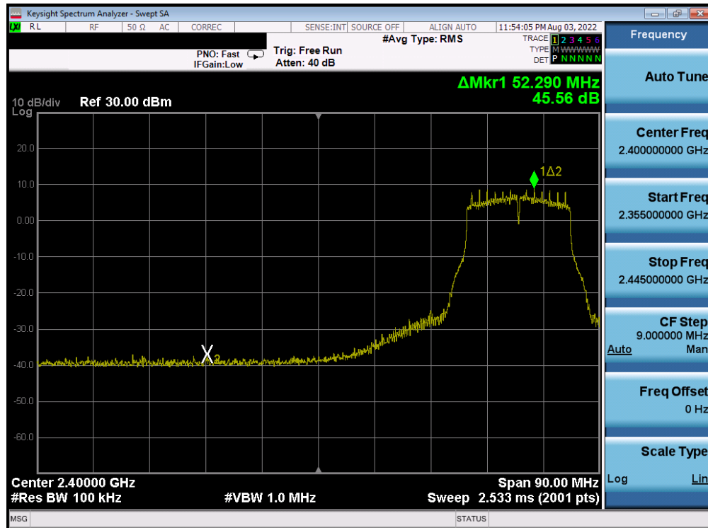
Plot 7-338. Band Edge Plot Antenna 2a (802.11g– Ch. 5) – 18Mbps
