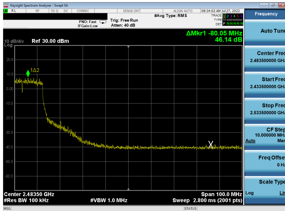
Plot 7-402. Band Edge Plot Antenna 2a (802.11n (2.4GHz) – Ch. 6 (high)) – MCS5
