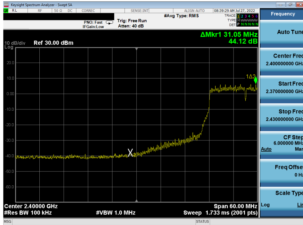
Plot 7-399. Band Edge Plot Antenna 2a (802.11n (2.4GHz) – Ch. 4) – MCS5
