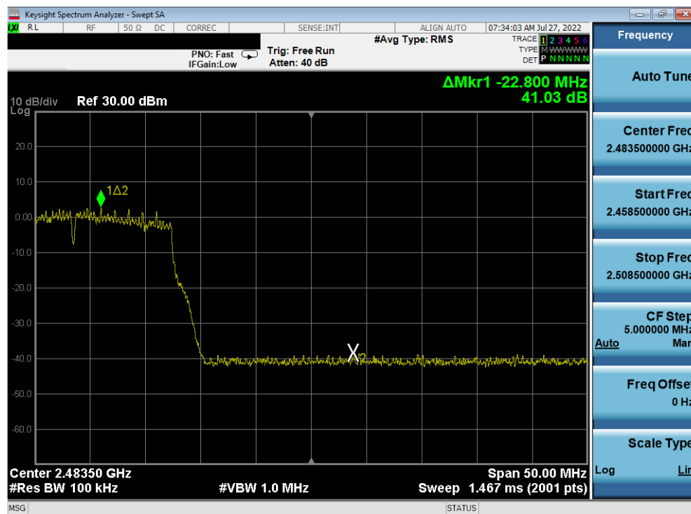
Plot 7-357. Band Edge Plot Antenna 2a (802.11n (2.4GHz) - Ch. 11) - MCS3
