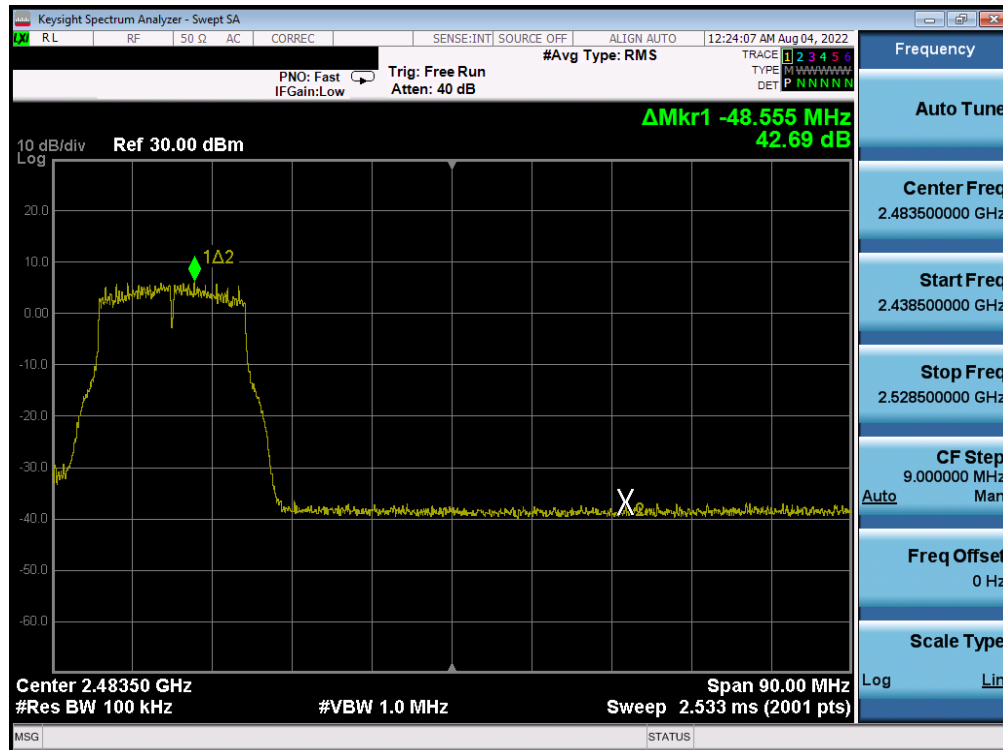
Plot 7-391. Band Edge Plot Antenna 2a (802.11g – Ch. 9) – 36Mbps
