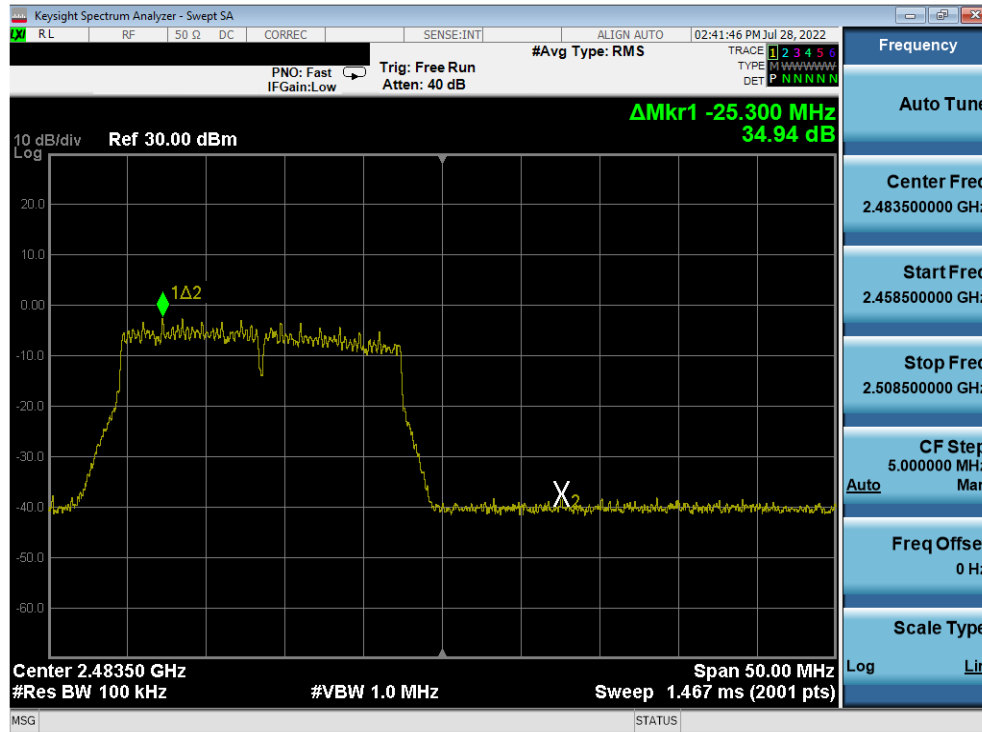
Plot 7-409. Band Edge Plot Antenna 2a (802.11n (2.4GHz) – Ch. 13) – MCS5
