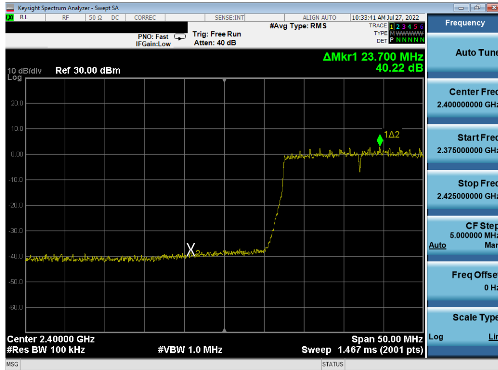
Plot 7-411. Band Edge Plot Antenna 2a (802.11ax (SU - 2.4GHz) – Ch. 2) – MCS5
