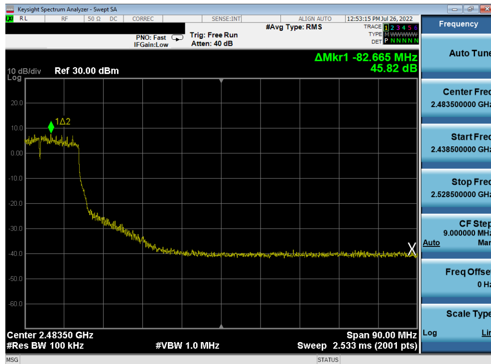
Plot 7-353. Band Edge Plot Antenna 2a (802.11n (2.4GHz) – Ch. 7) – MCS3
