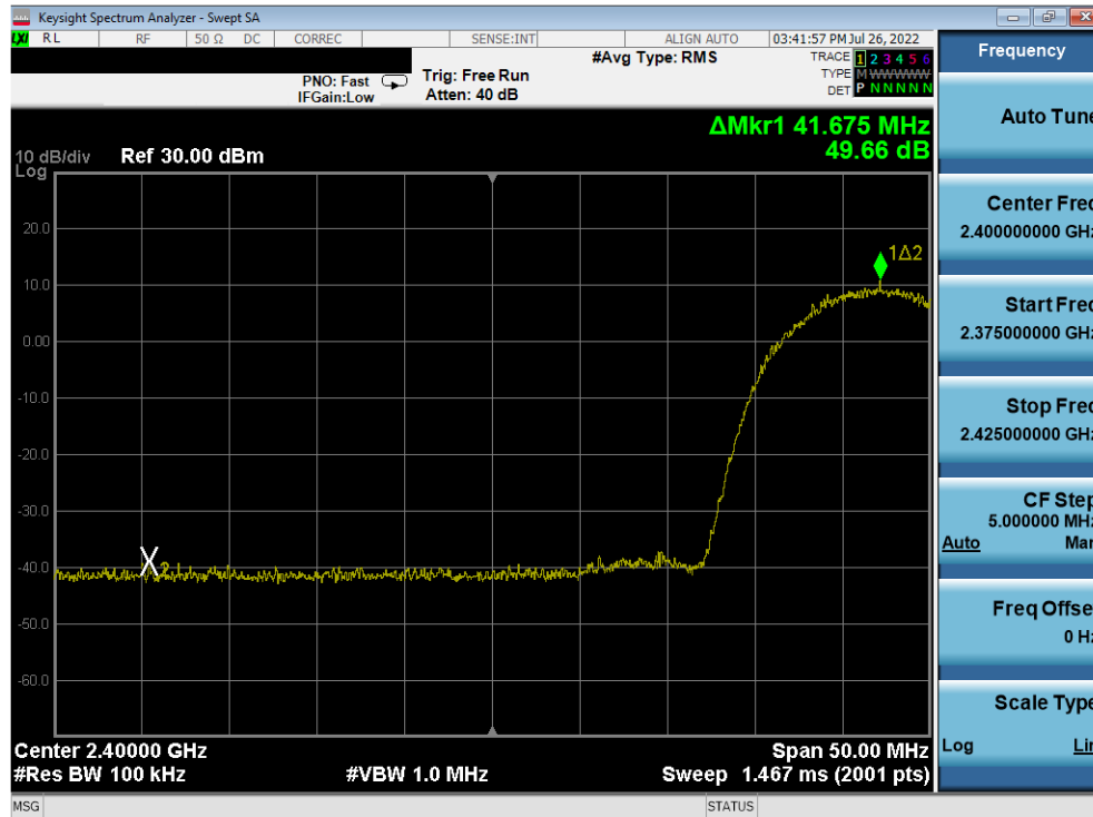
Plot 7-375. Band Edge Plot Antenna 2a (802.11b – Ch. 3) – 11Mbps
