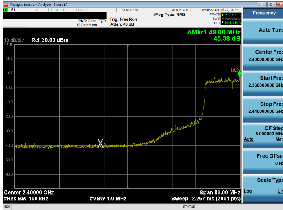
Plot 7-415. Band Edge Plot Antenna 2a (802.11ax (SU - 2.4GHz) – Ch. 6 (low)) – MCS5
