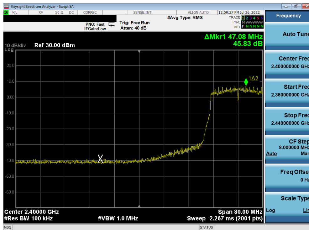
Plot 7-351. Band Edge Plot Antenna 2a (802.11n (2.4GHz) - Ch. 5) - MCS3
