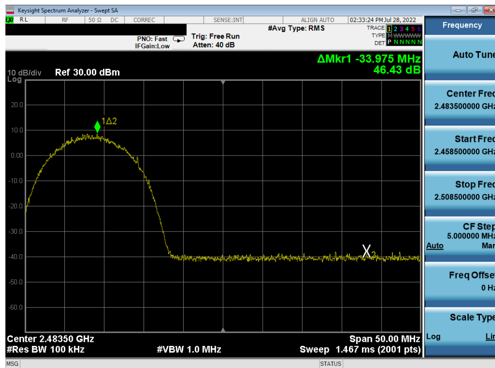
Plot 7-380. Band Edge Plot Antenna 2a (802.11b – Ch. 12) – 11Mbps
