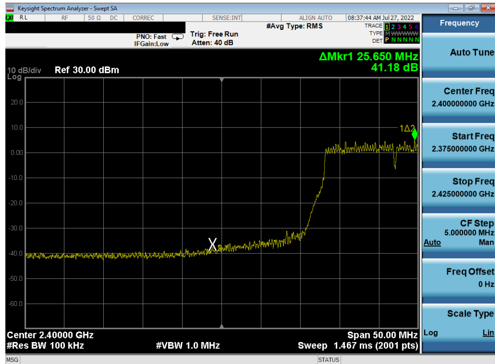
Plot 7-398. Band Edge Plot Antenna 2a (802.11n (2.4GHz) – Ch. 3) – MCS5
