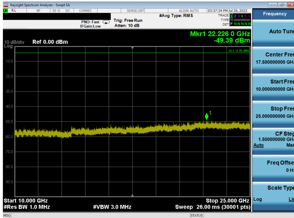
Plot 7-434. Conducted Spurious Plot Antenna 2a (802.11b – Ch. 11)
