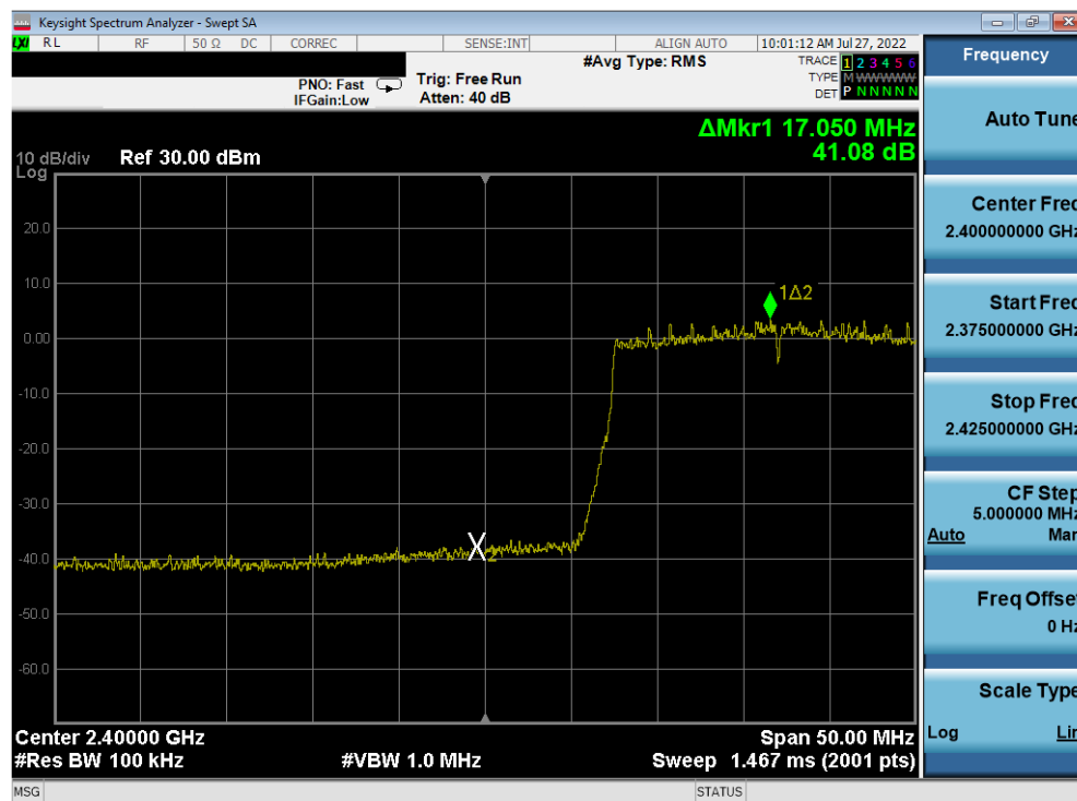
Plot 7-361. Band Edge Plot Antenna 2a (802.11ax (SU - 2.4GHz) – Ch. 2) – MCS3
