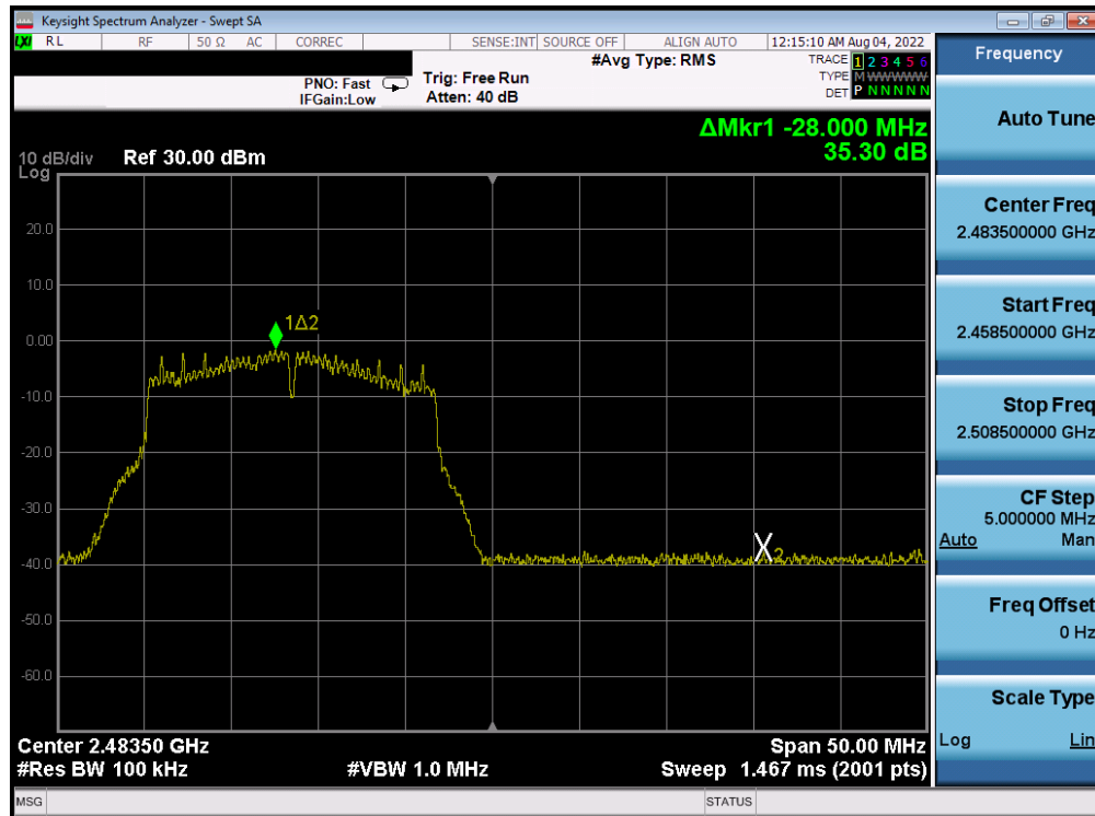
Plot 7-395. Band Edge Plot Antenna 2a (802.11g – Ch. 13) – 36Mbps
