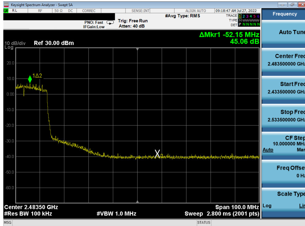
Plot 7-327. Band Edge Plot Antenna 2a (802.11ax (SU - 2.4GHz) – Ch. 6 (high)) – MCS2
