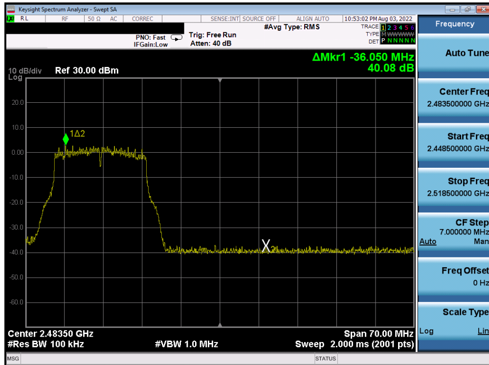
Plot 7-393. Band Edge Plot Antenna 2a (802.11g - Ch. 11) - 36Mbps
