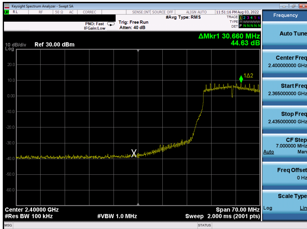
Plot 7-337. Band Edge Plot Antenna 2a (802.11g- Ch. 4) – 18Mbps
