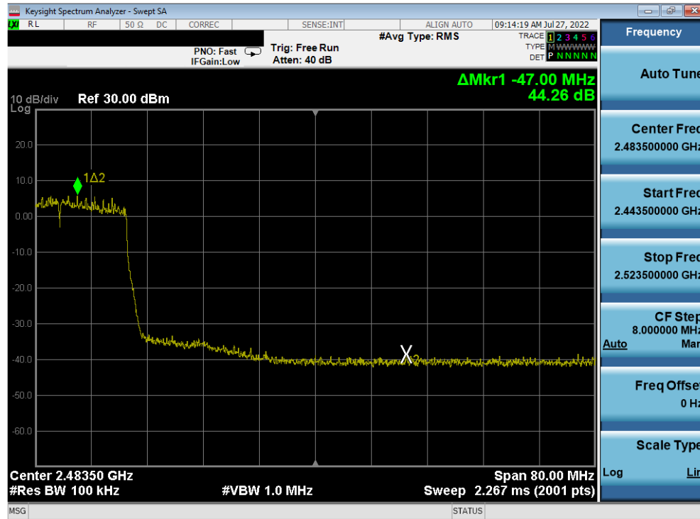
Plot 7-329. Band Edge Plot Antenna 2a (802.11ax (SU - 2.4GHz) – Ch. 8) – MCS2
