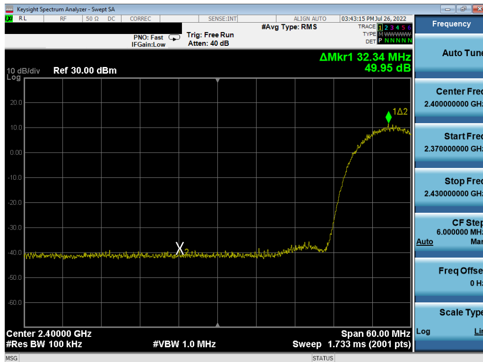
Plot 7-376. Band Edge Plot Antenna 2a (802.11b – Ch. 4) – 11Mbps
