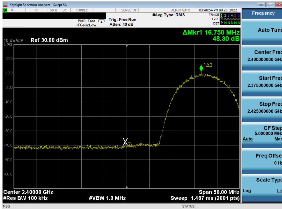
Plot 7-374. Band Edge Plot Antenna 2a (802.11b – Ch. 2) – 11Mbps
