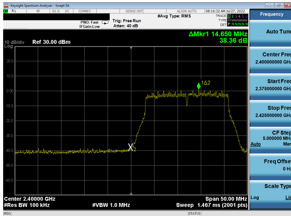
Plot 7-396. Band Edge Plot Antenna 2a (802.11n (2.4GHz) – Ch. 1) – MCS5
