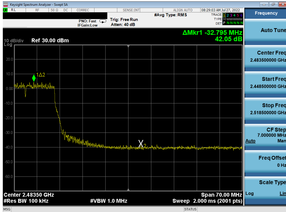
Plot 7-405. Band Edge Plot Antenna 2a (802.11n (2.4GHz) - Ch. 9) - MCS5
