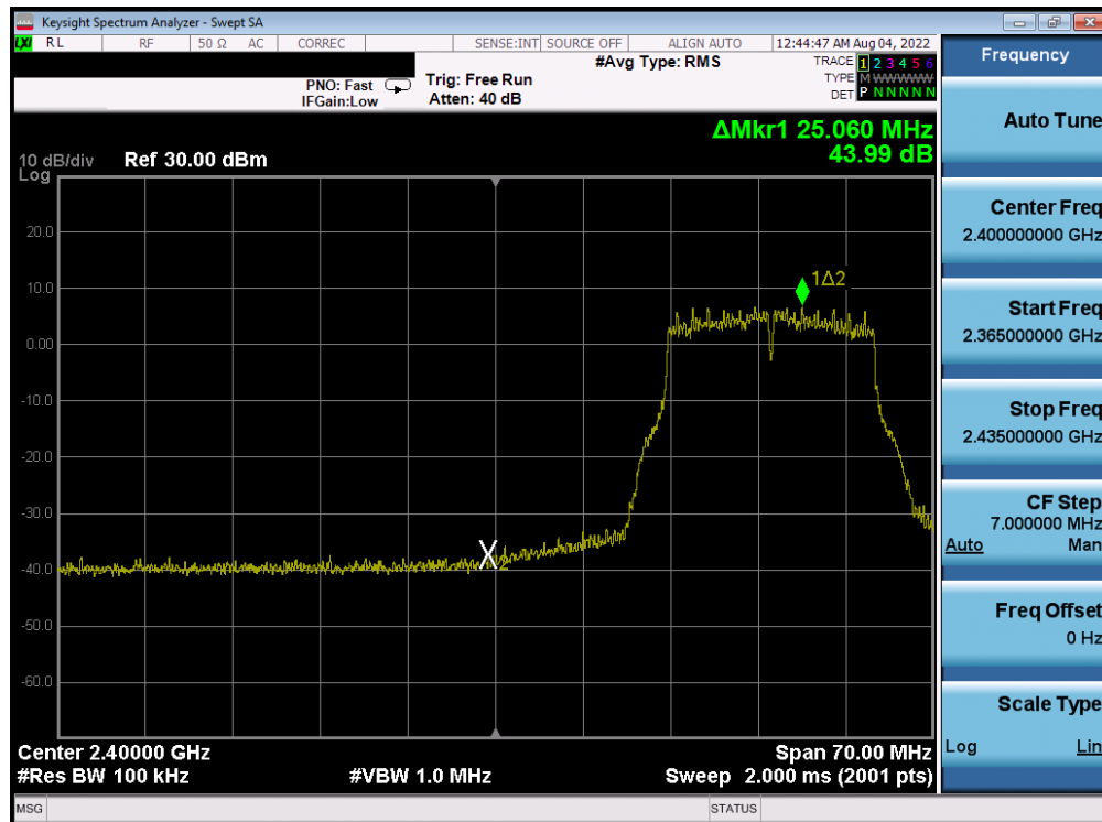
Plot 7-384. Band Edge Plot Antenna 2a (802.11g- Ch. 3) – 36Mbps
