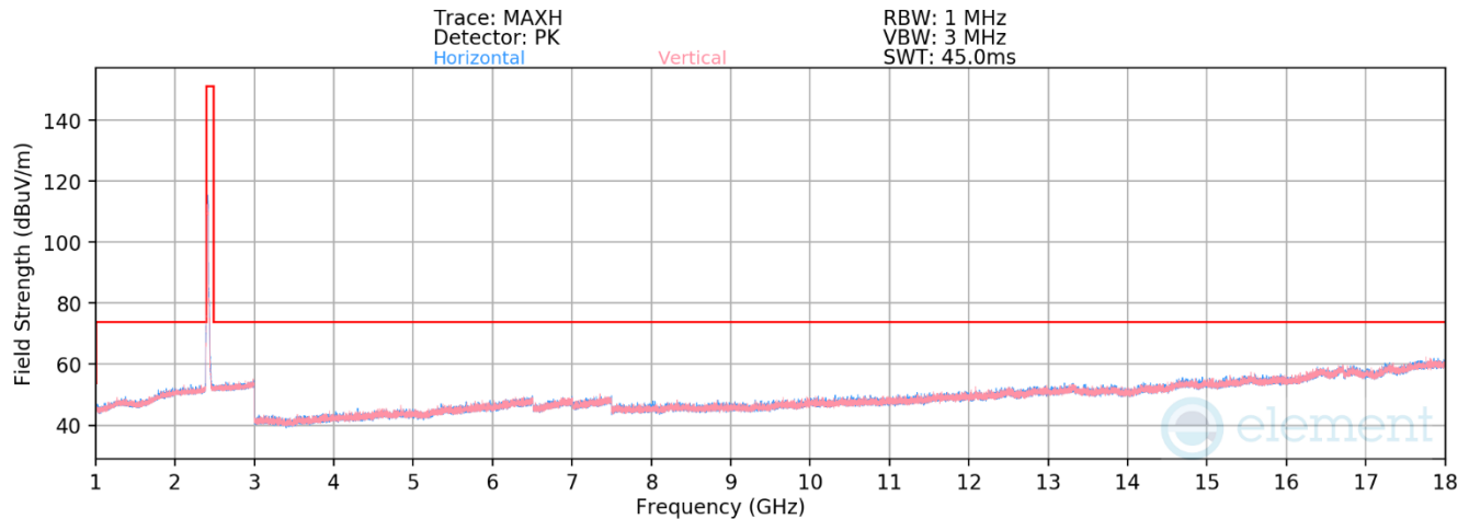
Plot 7-438. Radiated Spurious Emissions above 1GHz Antenna 4a (802.11ax(SU) – Ch. 1)
