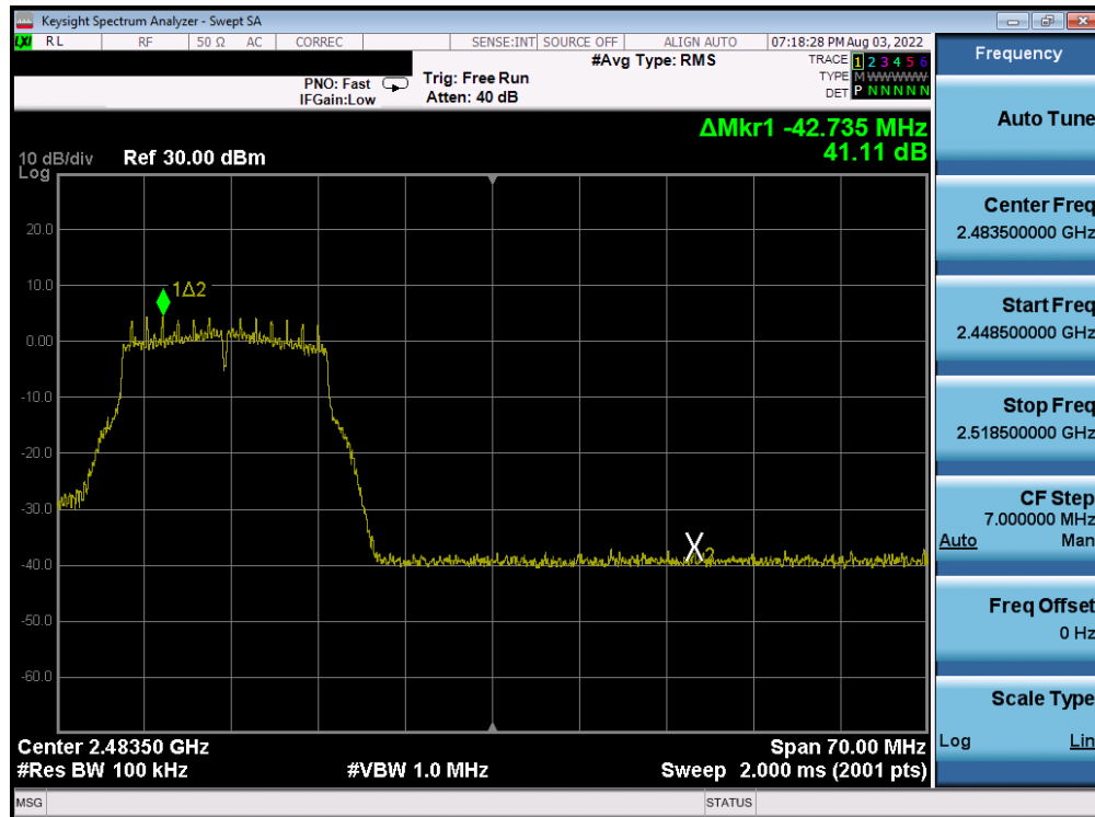
Plot 7-344. Band Edge Plot Antenna 2a (802.11g – Ch. 11) – 18Mbps
