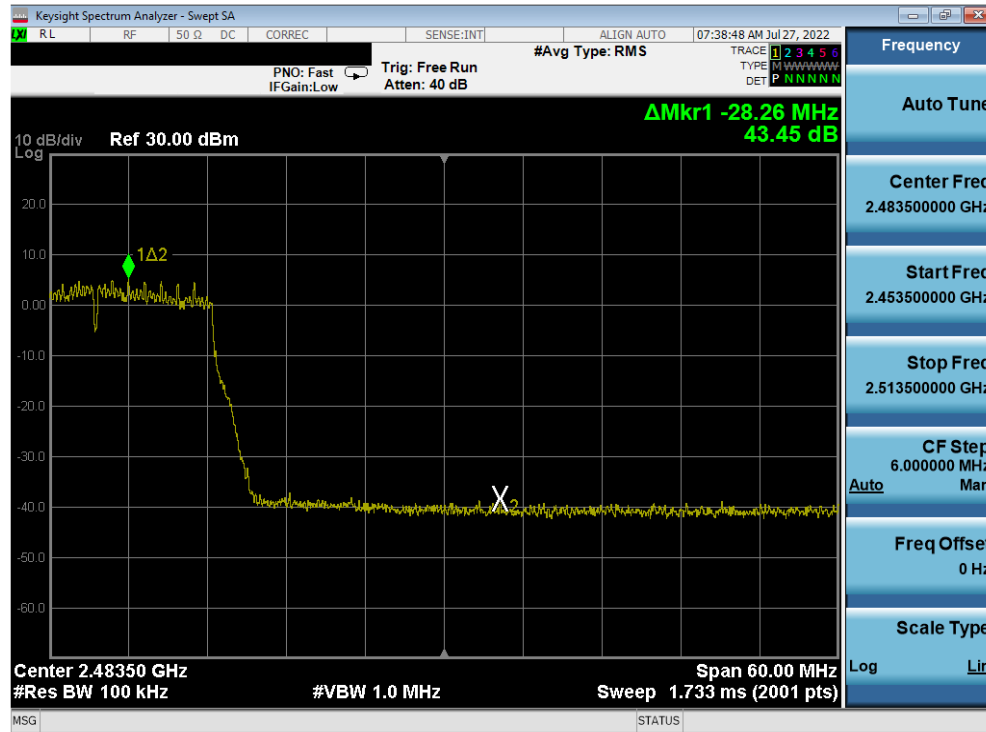
Plot 7-356. Band Edge Plot Antenna 2a (802.11n (2.4GHz) - Ch. 10) - MCS3
