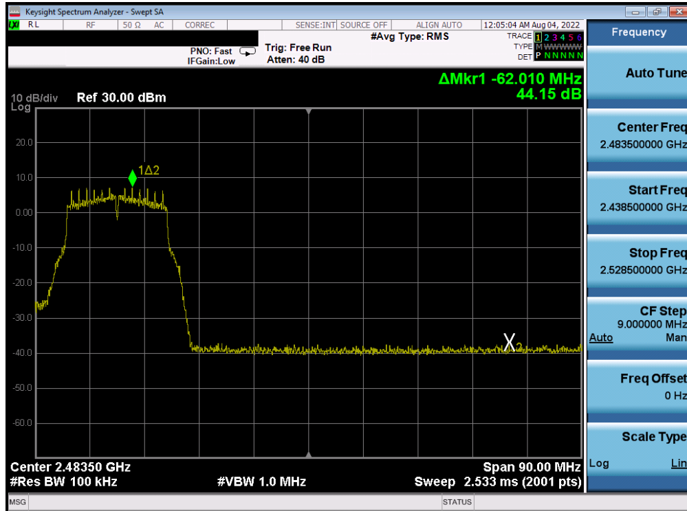
Plot 7-342. Band Edge Plot Antenna 2a (802.11g – Ch. 9) – 18Mbps
