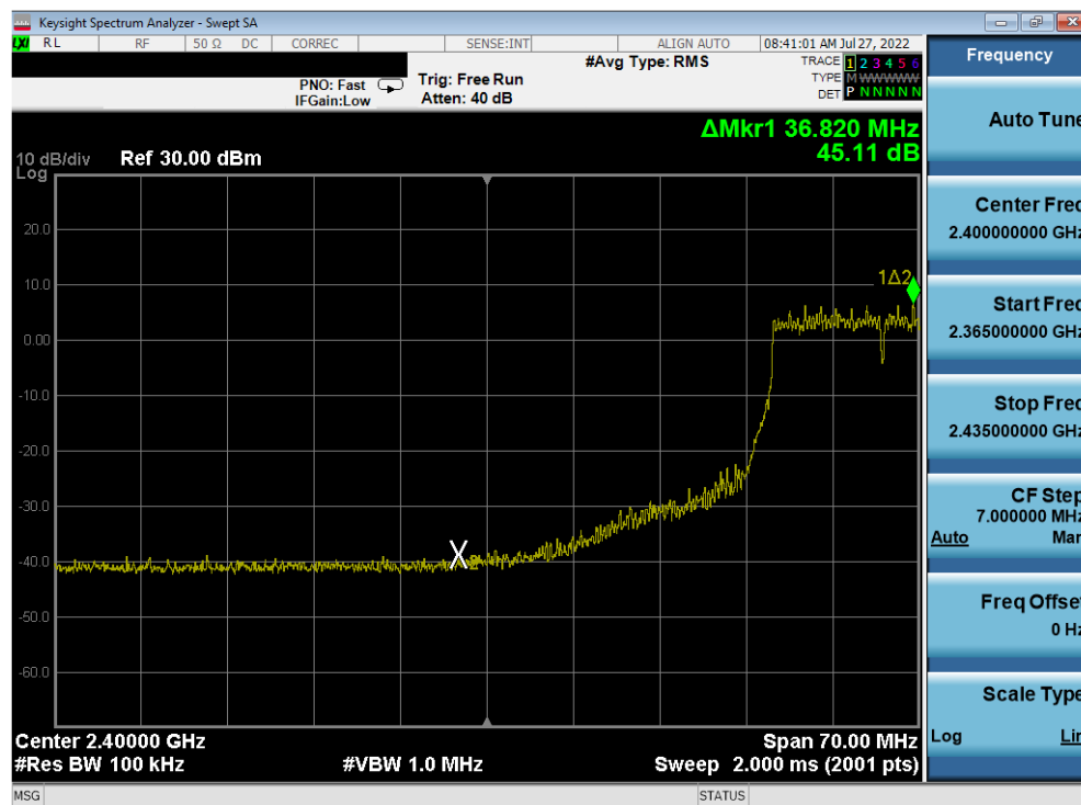
Plot 7-400. Band Edge Plot Antenna 2a (802.11n (2.4GHz) – Ch. 5) – MCS5
