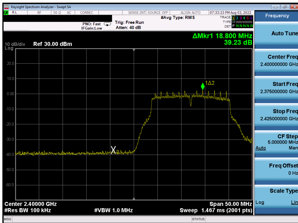
Plot 7-334. Band Edge Plot Antenna 2a (802.11g- Ch. 1) - 18Mbps
