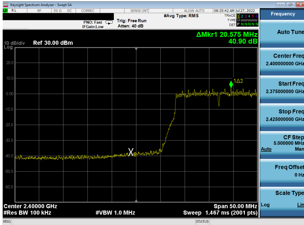
Plot 7-397. Band Edge Plot Antenna 2a (802.11n (2.4GHz) – Ch. 2) – MCS5
