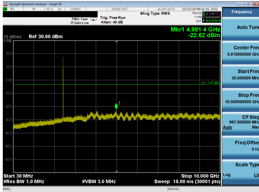
Plot 7-431. Conducted Spurious Plot Antenna 2a (802.11b – Ch. 6)
