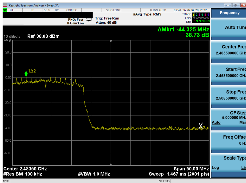
Plot 7-333. Band Edge Plot Antenna 2a (802.11ax (SU - 2.4GHz) – Ch. 12) – MCS2
