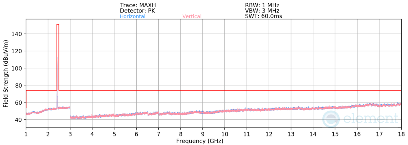
Plot 7-435. Radiated Spurious Emissions above 1GHz Antenna 4a (802.11b – Ch. 1)
