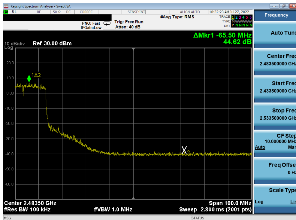
Plot 7-416. Band Edge Plot Antenna 2a (802.11ax (SU - 2.4GHz) – Ch. 6 (high)) – MCS5
