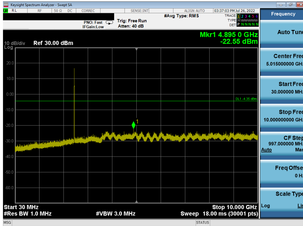
Plot 7-433. Conducted Spurious Plot Antenna 2a (802.11b – Ch. 11)
