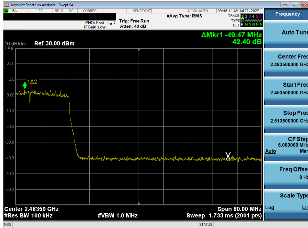
Plot 7-370. Band Edge Plot Antenna 2a (802.11ax (SU - 2.4GHz) - Ch. 10) - MCS3
