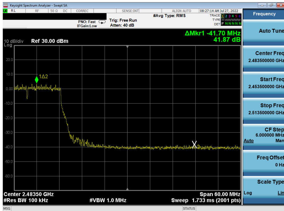
Plot 7-406. Band Edge Plot Antenna 2a (802.11n (2.4GHz) - Ch. 10) - MCS5
