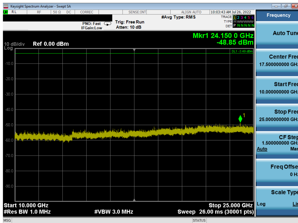
Plot 7-426. Conducted Spurious Plot Antenna 4a (802.11b – Ch. 6)
