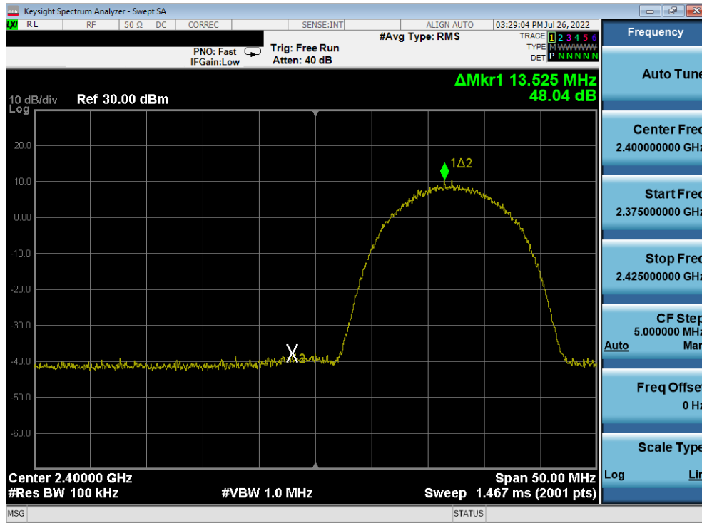
Plot 7-373. Band Edge Plot Antenna 2a (802.11b – Ch. 1) – 11Mbps
