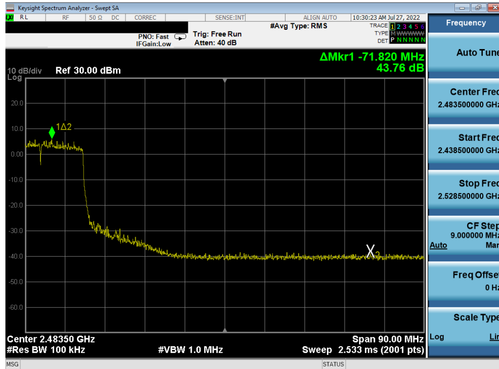
Plot 7-417. Band Edge Plot Antenna 2a (802.11ax (SU - 2.4GHz) – Ch. 7) – MCS5
