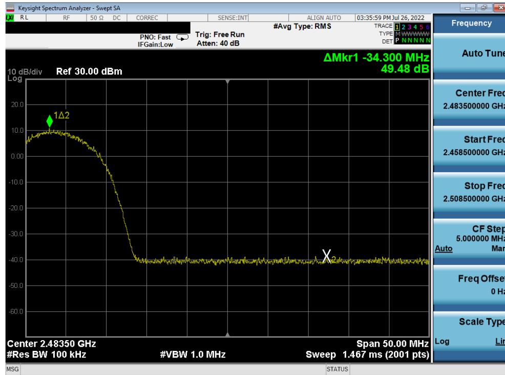
Plot 7-379. Band Edge Plot Antenna 2a (802.11b – Ch. 11) – 11Mbps
