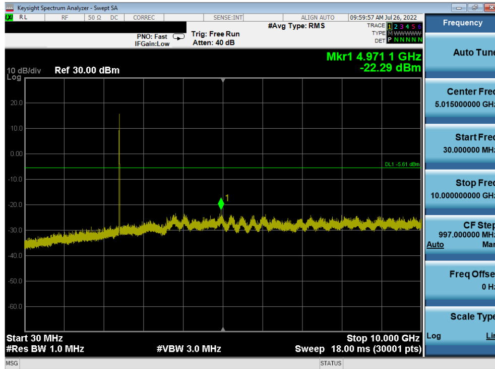
Plot 7-423. Conducted Spurious Plot Antenna 4a (802.11b – Ch. 1)
