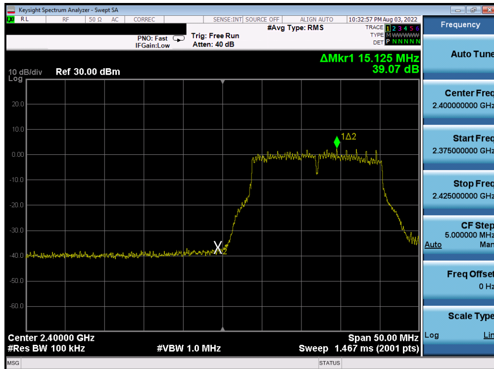
Plot 7-382. Band Edge Plot Antenna 2a (802.11g– Ch. 1) – 36Mbps
