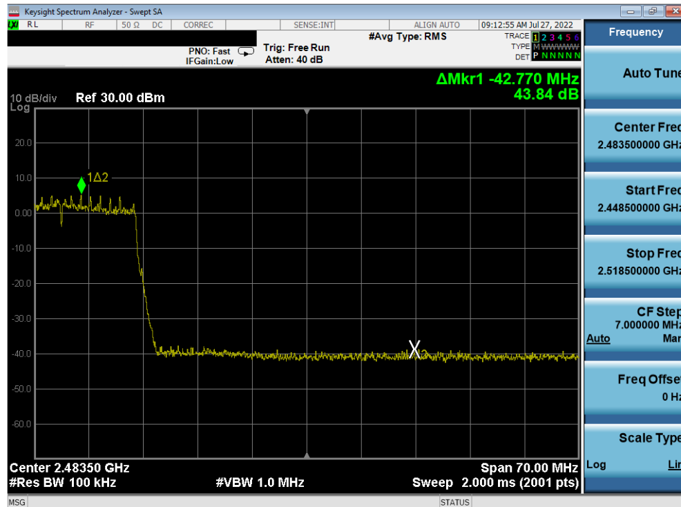
Plot 7-330. Band Edge Plot Antenna 2a (802.11ax (SU - 2.4GHz) – Ch. 9) – MCS2
