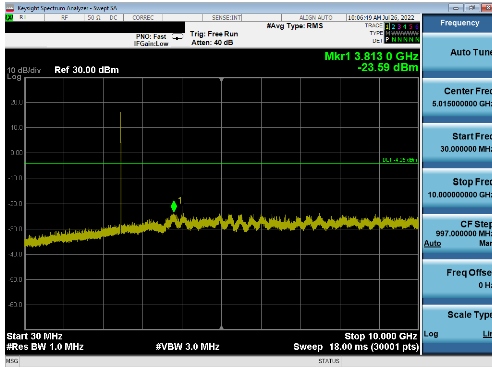
Plot 7-427. Conducted Spurious Plot Antenna 4a (802.11b – Ch. 11)
