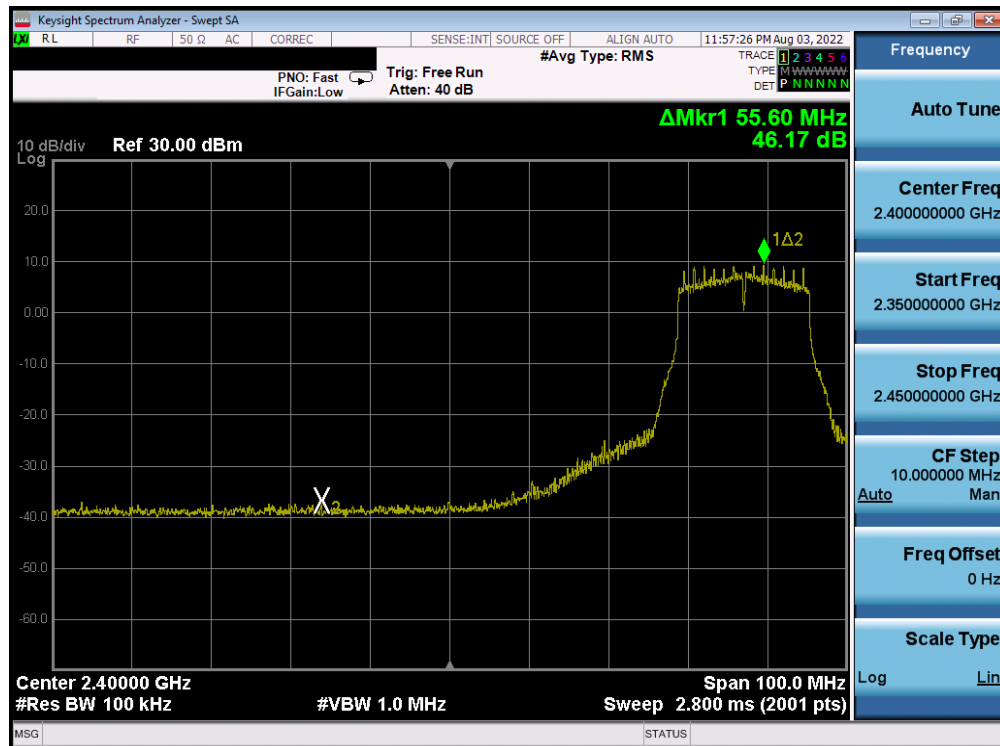
Plot 7-339. Band Edge Plot Antenna 2a (802.11g– Ch. 6 (low)) – 18Mbps
