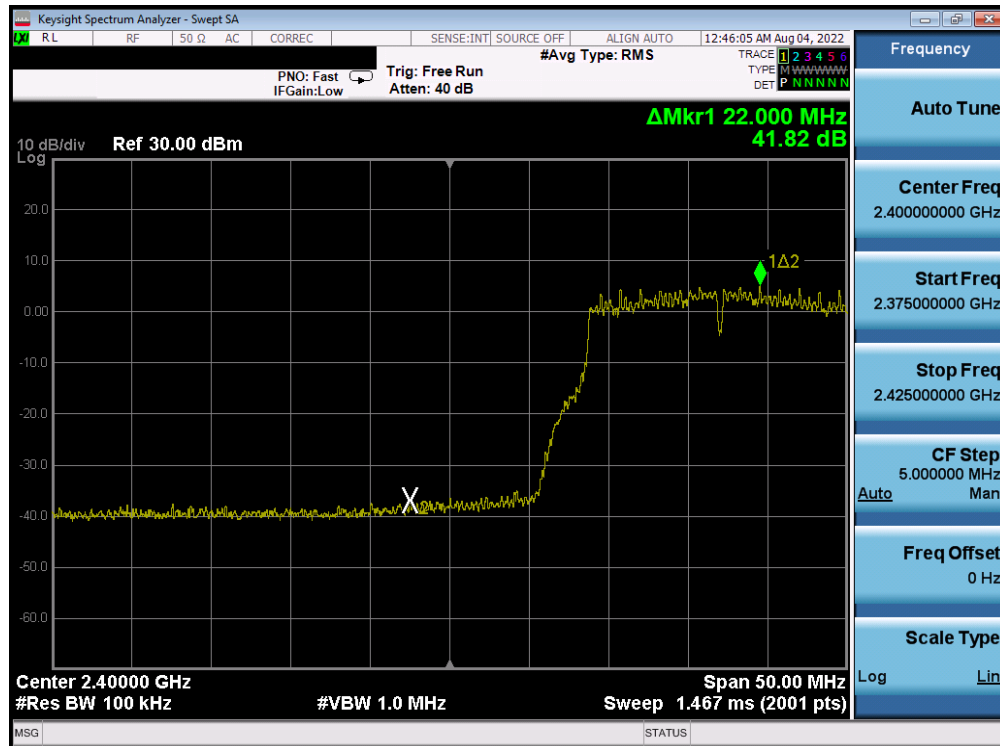
Plot 7-383. Band Edge Plot Antenna 2a (802.11g- Ch. 2) – 36Mbps
