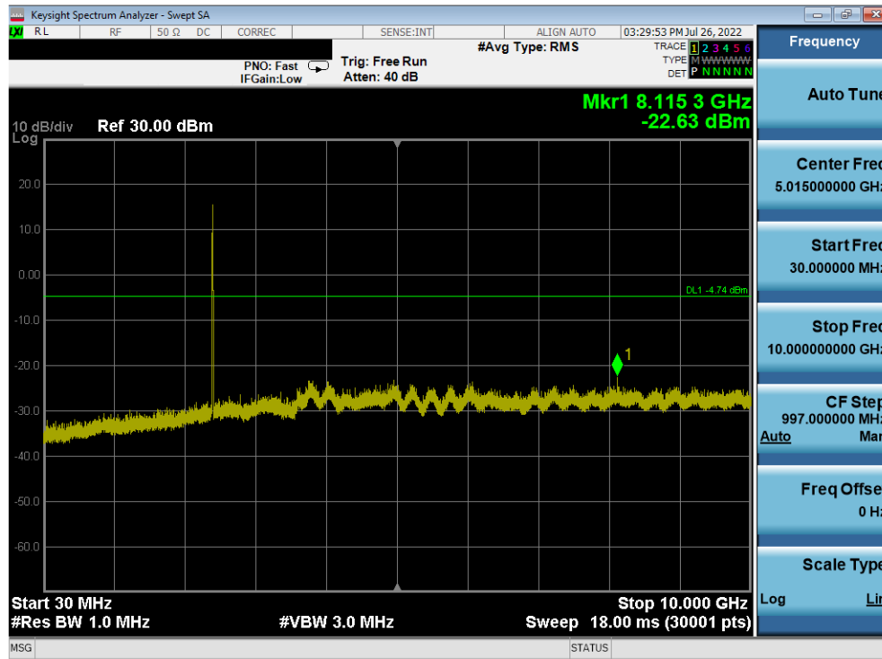
Plot 7-429. Conducted Spurious Plot Antenna 2a (802.11b – Ch. 1)
