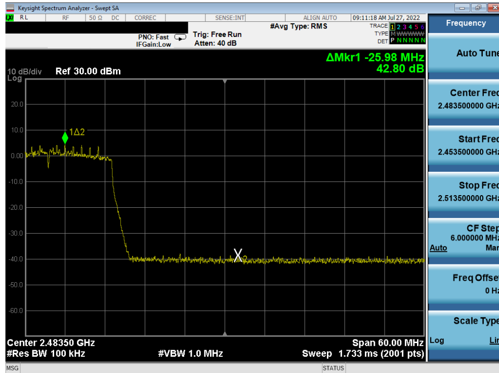
Plot 7-331. Band Edge Plot Antenna 2a (802.11ax (SU - 2.4GHz) – Ch. 10) – MCS2
