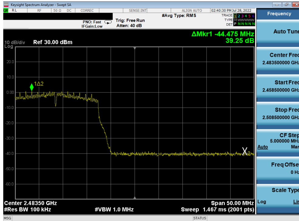
Plot 7-358. Band Edge Plot Antenna 2a (802.11n (2.4GHz) - Ch. 12) - MCS3
