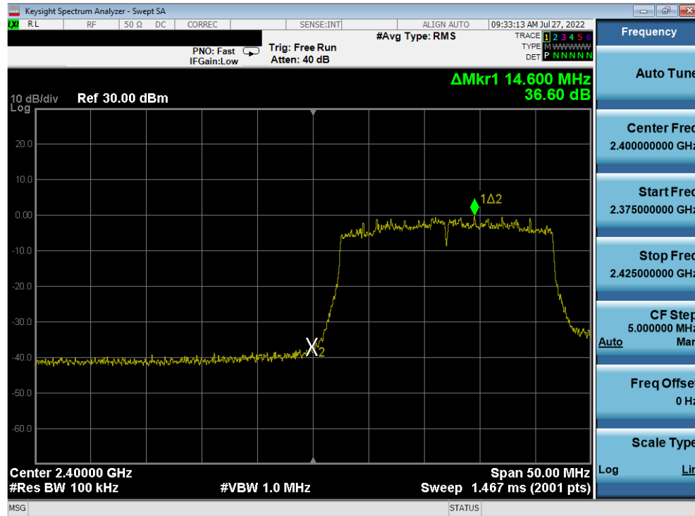
Plot 7-360. Band Edge Plot Antenna 2a (802.11ax (SU - 2.4GHz) – Ch. 1) – MCS3
