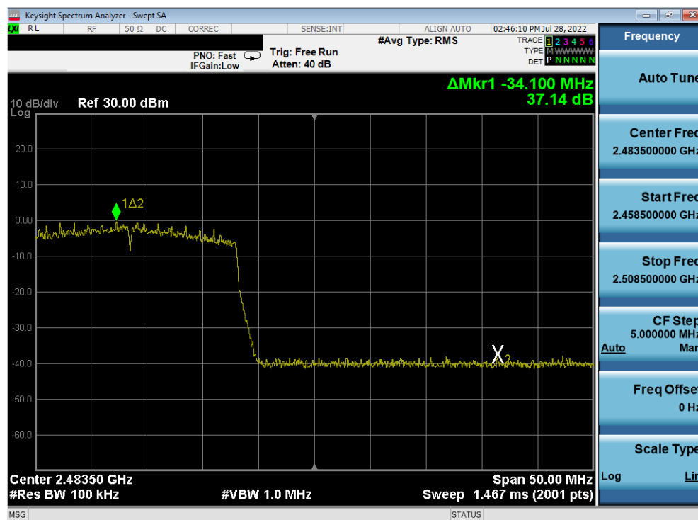
Plot 7-372. Band Edge Plot Antenna 2a (802.11ax (SU - 2.4GHz) – Ch. 12) – MCS3
