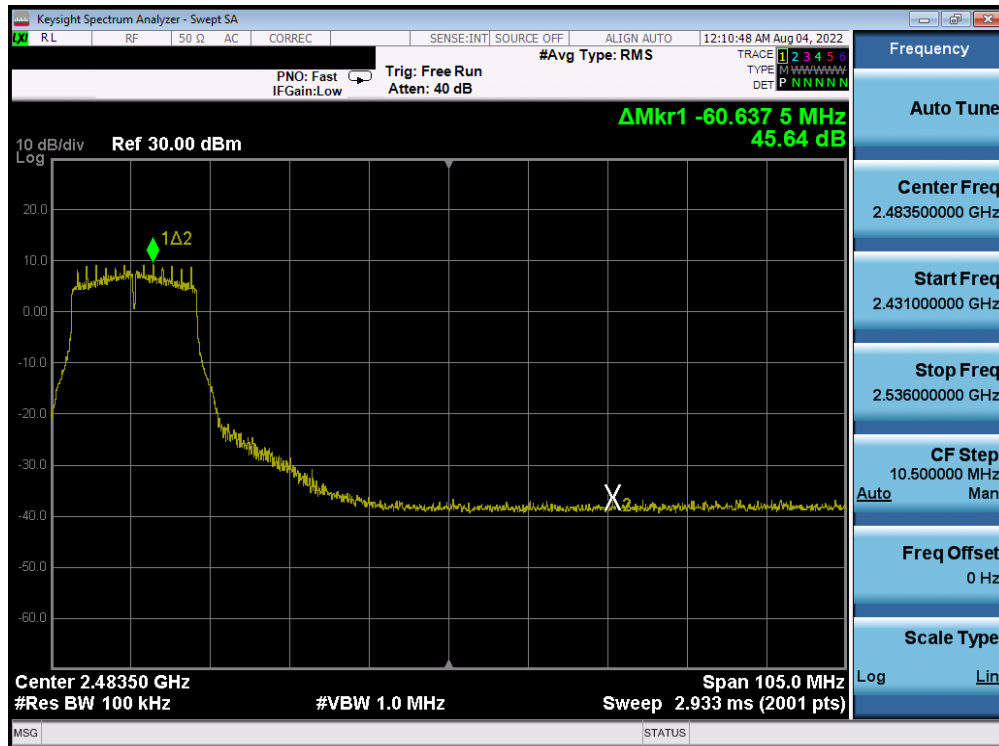
Plot 7-340. Band Edge Plot Antenna 2a (802.11g- Ch. 7) – 18Mbps
