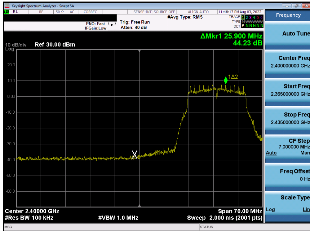
Plot 7-336. Band Edge Plot Antenna 2a (802.11g- Ch. 3) – 18Mbps
