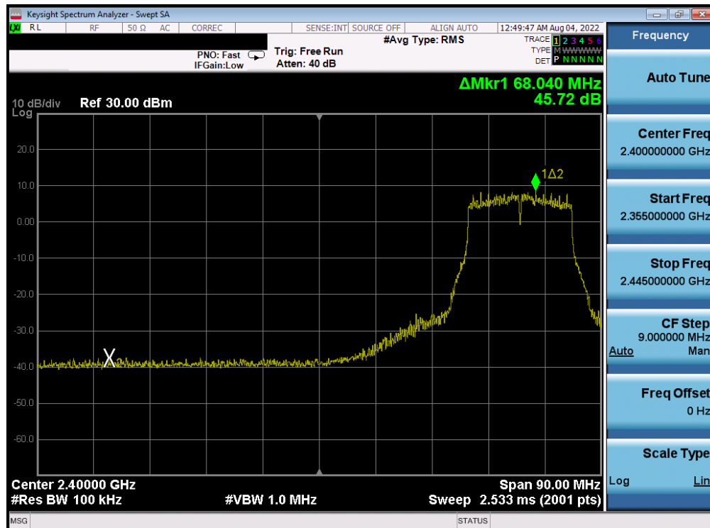
Plot 7-386. Band Edge Plot Antenna 2a (802.11g- Ch. 5) – 36Mbps
