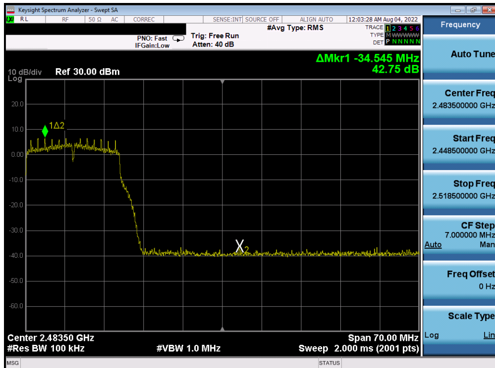
Plot 7-343. Band Edge Plot Antenna 2a (802.11g – Ch. 10) – 18Mbps
