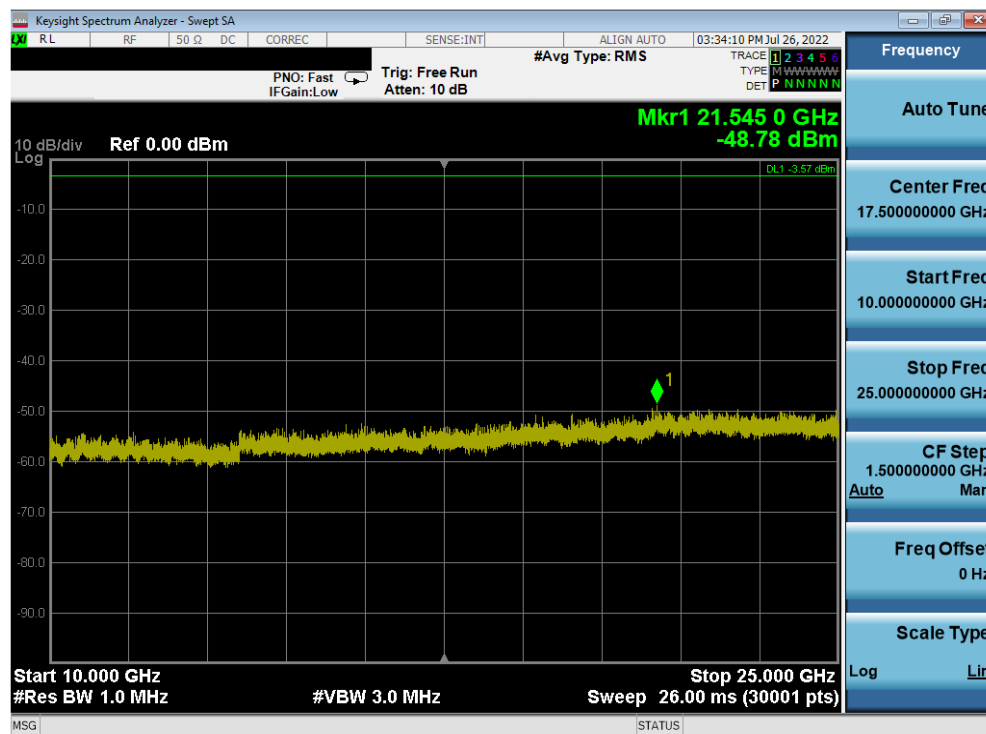
Plot 7-432. Conducted Spurious Plot Antenna 2a (802.11b – Ch. 6)
