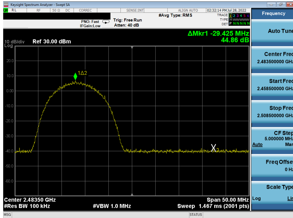
Plot 7-381. Band Edge Plot Antenna 2a (802.11b – Ch. 13) – 11Mbps
