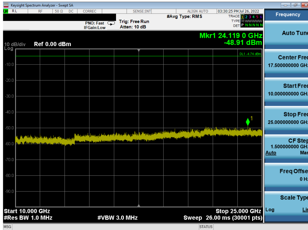
Plot 7-430. Conducted Spurious Plot Antenna 2a (802.11b – Ch. 1)
