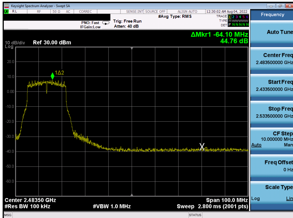
Plot 7-390. Band Edge Plot Antenna 2a (802.11g- Ch. 8) – 36Mbps
