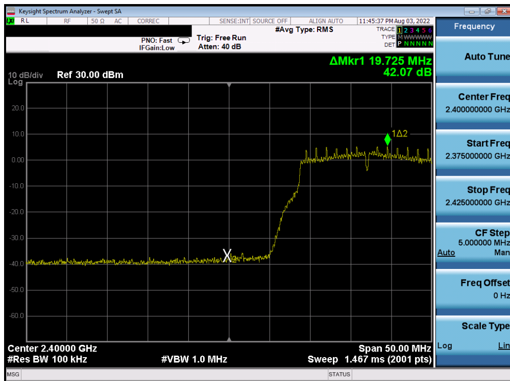
Plot 7-335. Band Edge Plot Antenna 2a (802.11g- Ch. 2) - 18Mbps
