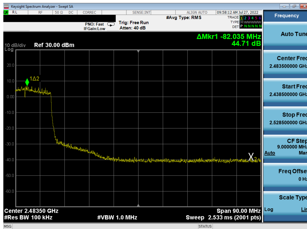
Plot 7-367. Band Edge Plot Antenna 2a (802.11ax (SU - 2.4GHz) – Ch. 7) – MCS3
