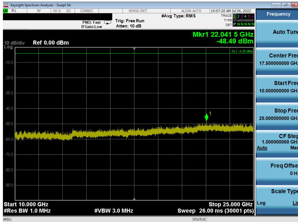
Plot 7-428. Conducted Spurious Plot Antenna 4a (802.11b – Ch. 11)
