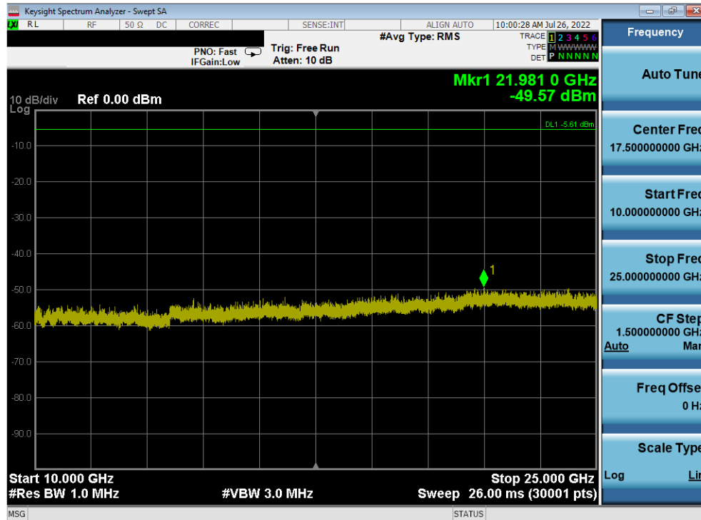
Plot 7-424. Conducted Spurious Plot Antenna 4a (802.11b – Ch. 1)
