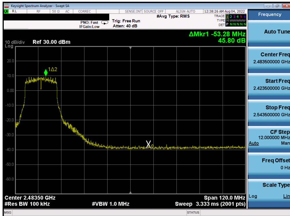
Plot 7-388. Band Edge Plot Antenna 2a (802.11g- Ch. 6 (high)) – 36Mbps
