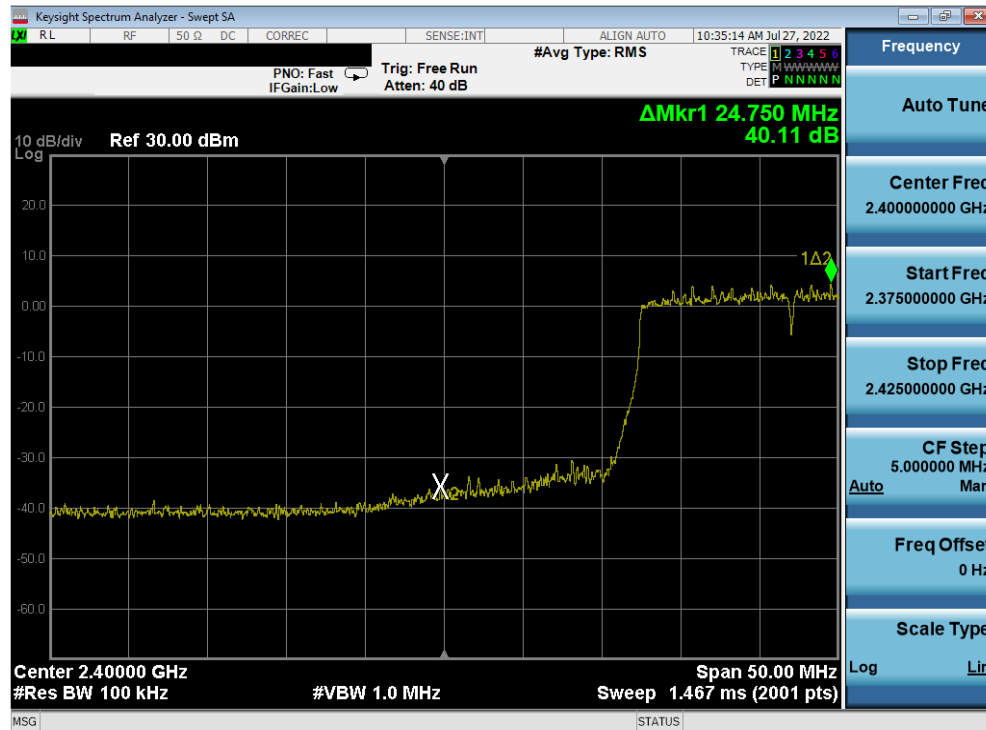
Plot 7-412. Band Edge Plot Antenna 2a (802.11ax (SU - 2.4GHz) – Ch. 3) – MCS5
