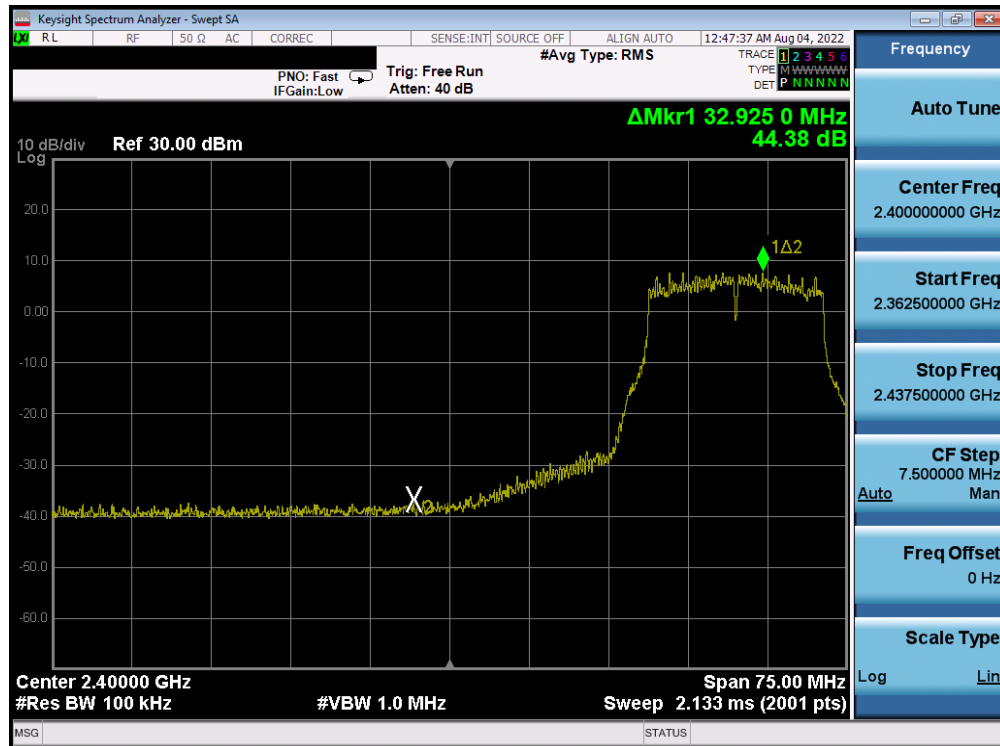
Plot 7-385. Band Edge Plot Antenna 2a (802.11g- Ch. 4) – 36Mbps
