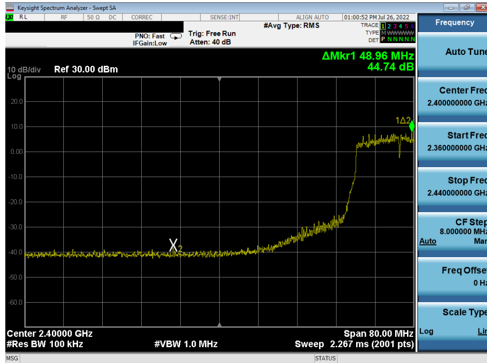
Plot 7-352. Band Edge Plot Antenna 2a (802.11n (2.4GHz) – Ch. 6 (low)) – MCS3
