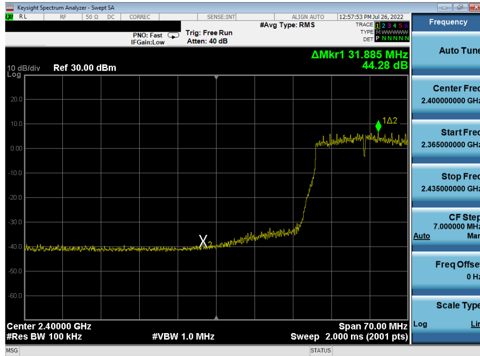
Plot 7-350. Band Edge Plot Antenna 2a (802.11n (2.4GHz) - Ch. 4) - MCS3
