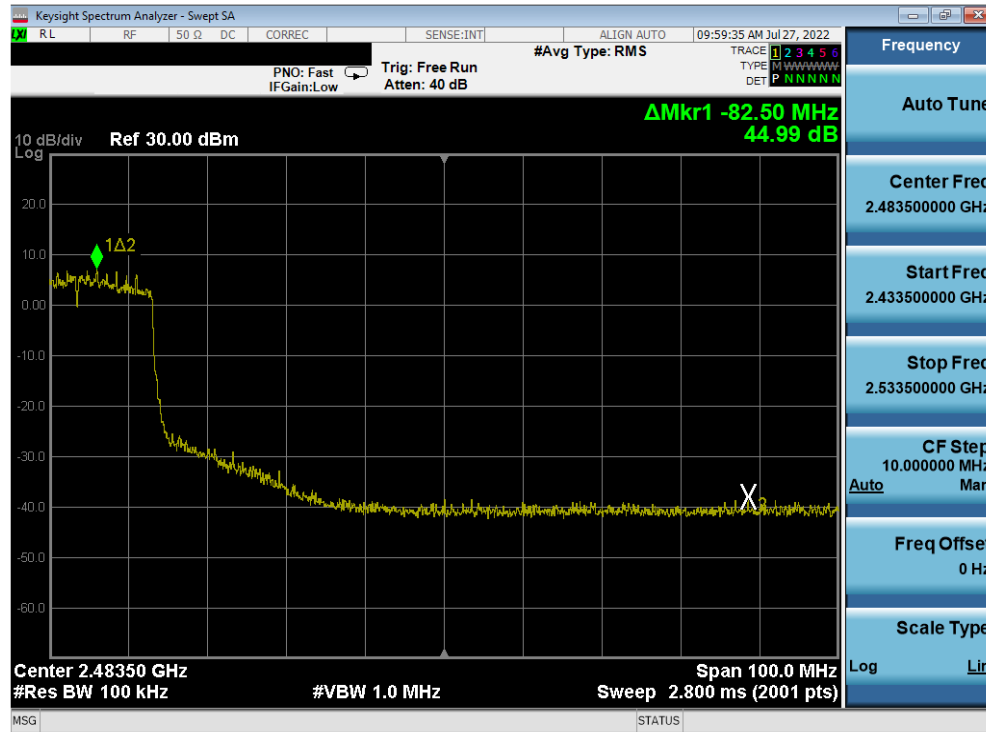
Plot 7-366. Band Edge Plot Antenna 2a (802.11ax (SU - 2.4GHz) – Ch. 6 (High)) – MCS3
