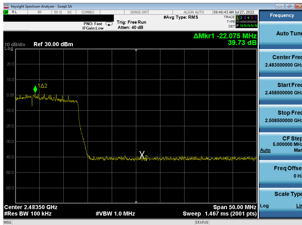
Plot 7-371. Band Edge Plot Antenna 2a (802.11ax (SU - 2.4GHz) - Ch. 11) - MCS3
