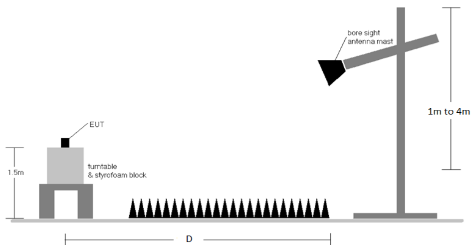
Figure 7-6. Radiated Measurement Setup
