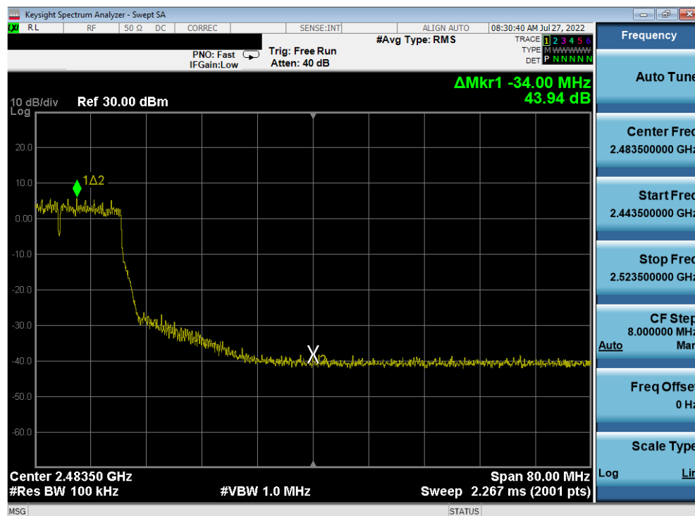
Plot 7-404. Band Edge Plot Antenna 2a (802.11n (2.4GHz) – Ch. 8) – MCS5
