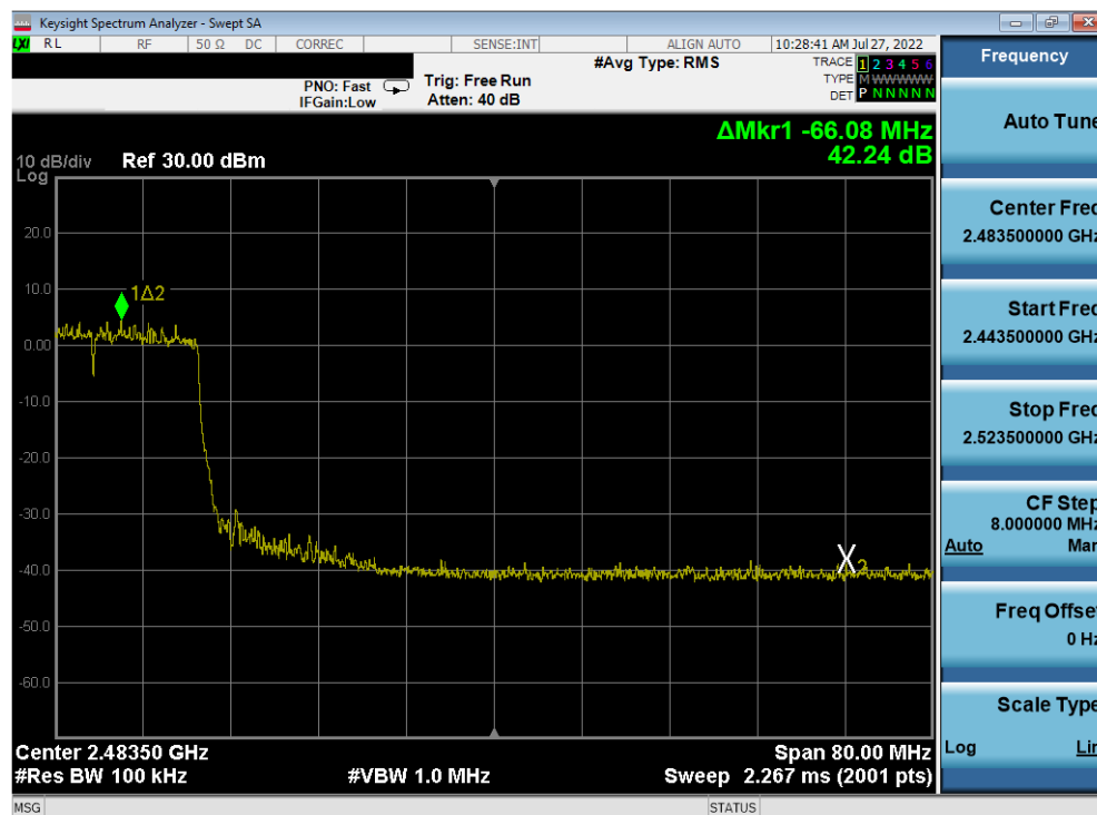
Plot 7-418. Band Edge Plot Antenna 2a (802.11ax (SU - 2.4GHz) – Ch. 8) – MCS5
