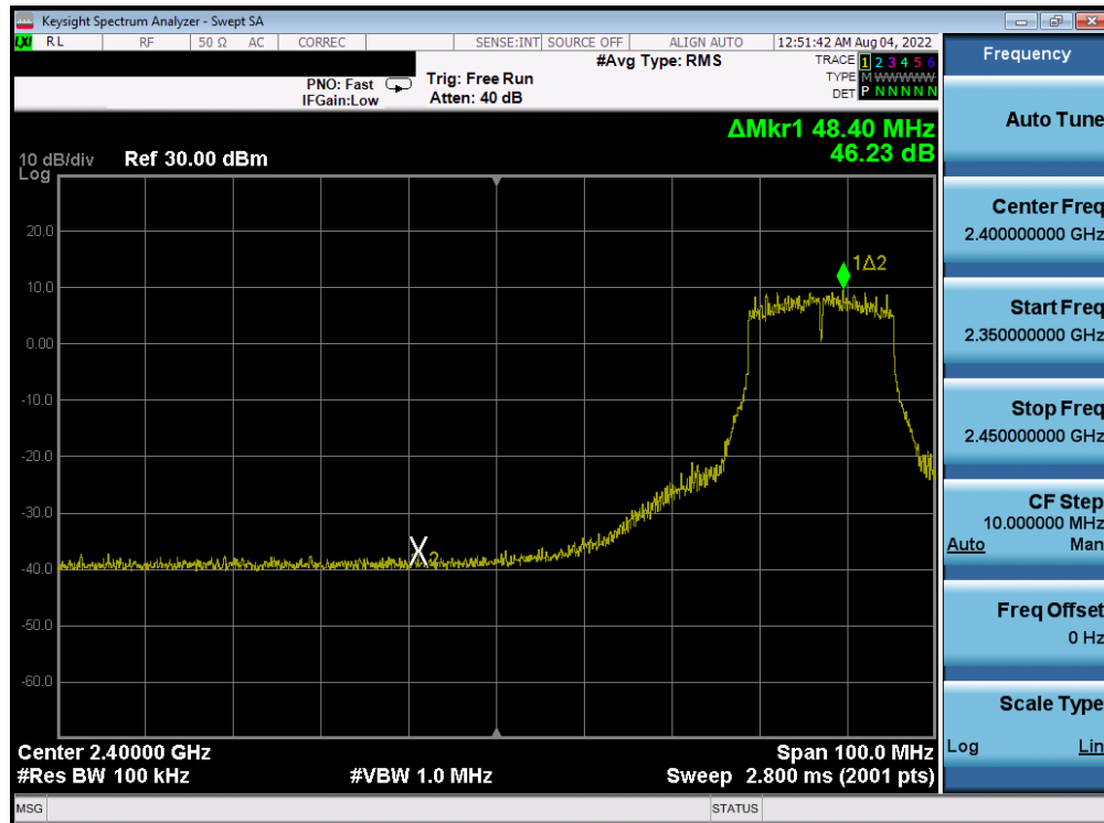
Plot 7-387. Band Edge Plot Antenna 2a (802.11g- Ch. 6 (low)) – 36Mbps
