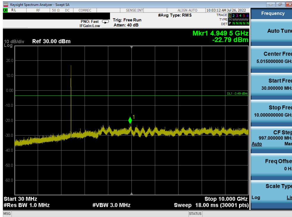
Plot 7-425. Conducted Spurious Plot Antenna 4a (802.11b – Ch. 6)
