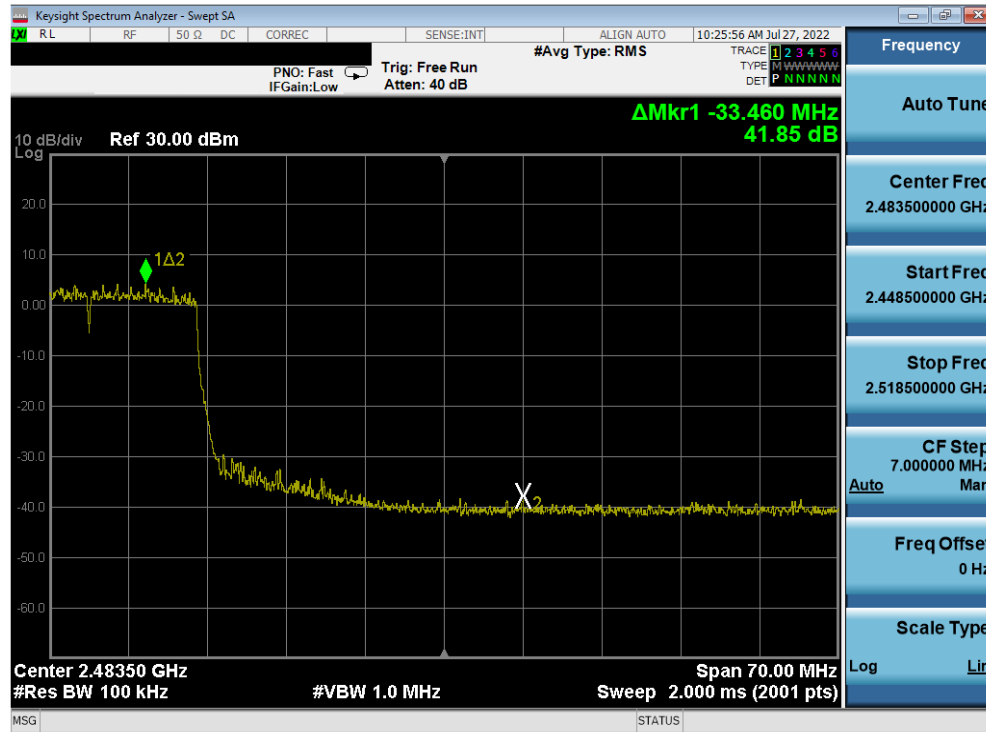
Plot 7-419. Band Edge Plot Antenna 2a (802.11ax (SU - 2.4GHz) – Ch. 9) – MCS5
