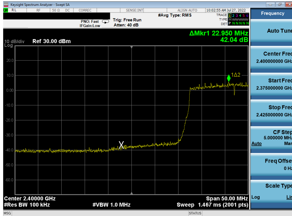
Plot 7-362. Band Edge Plot Antenna 2a (802.11ax (SU - 2.4GHz) – Ch. 3) – MCS3
