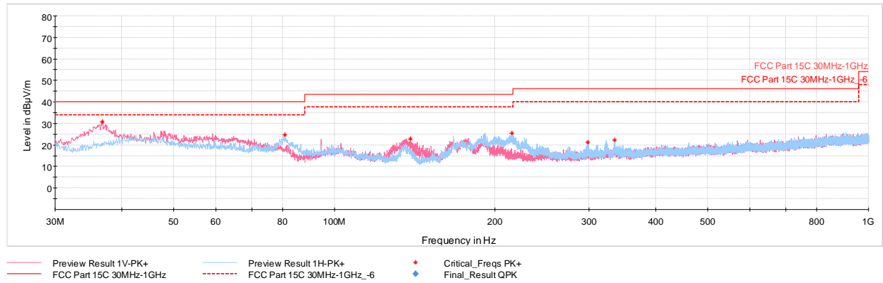
Plot 7-195. Radiated Spurious Emissions below 1GHz CDD Ch.6 (RU242), with AC/DC Adapter
