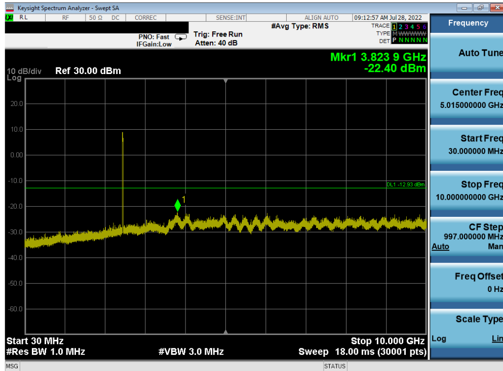
Plot 7-113. Conducted Spurious Plot Antenna 4a (802.11ax OFDMA – RU242 – Ch. 11)
