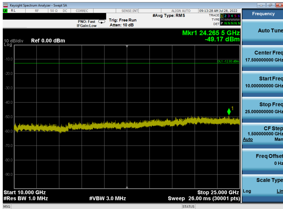
Plot 7-114. Conducted Spurious Plot Antenna 4a (802.11ax OFDMA – RU242 – Ch. 11)
