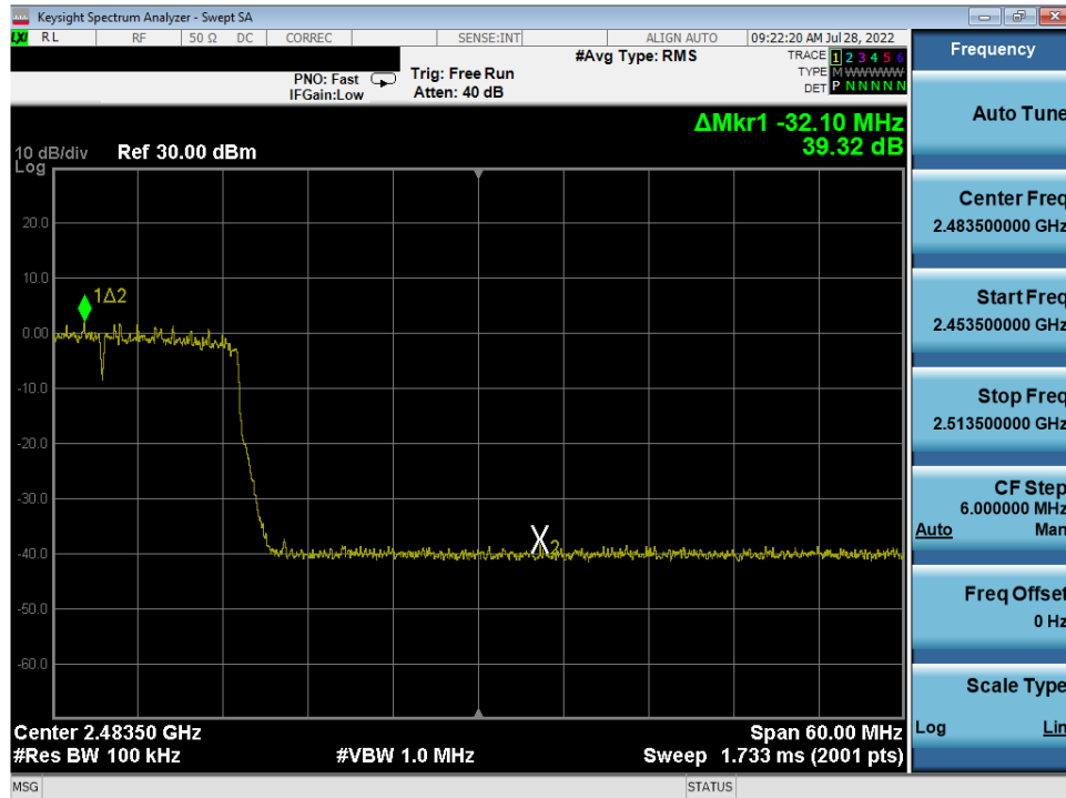
Plot 7-85. Band Edge Antenna 4a (802.11ax OFDMA – RU242 – Ch. 10)
