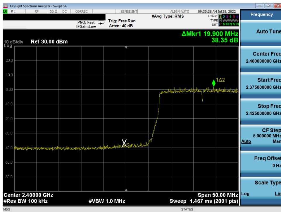
Plot 7-76. Band Edge Antenna 4a (802.11ax OFDMA – RU242 – Ch. 2)
