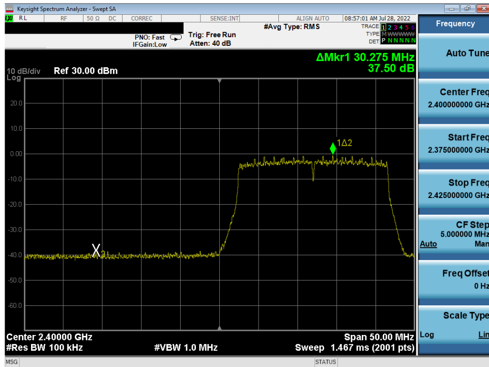
Plot 7-75. Band Edge Antenna 4a (802.11ax OFDMA – RU242 – Ch. 1)
