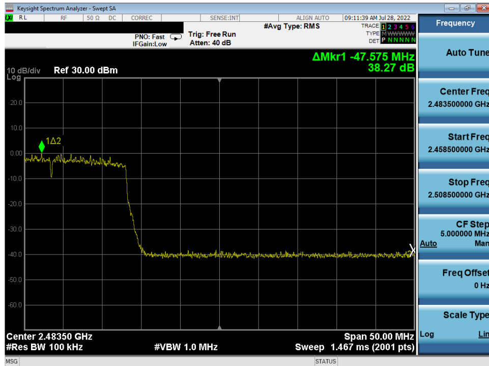
Plot 7-86. Band Edge Antenna 4a (802.11ax OFDMA – RU242 – Ch. 11)
