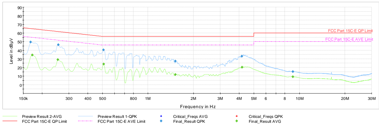
Plot 7-106. AC Line Conducted Plot with Bluetooth HDR (N, 4Mbps ePA - Ch.38 with AC/DC Adapter)
