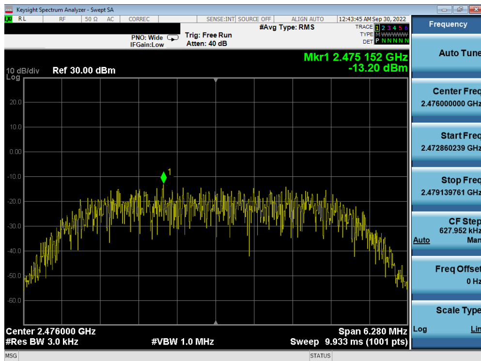
Plot 7-60. Power Spectral Density Plot TxBF Antenna 2a (Bluetooth (HDR8), 8Mbps, iPA – Ch. 7)
