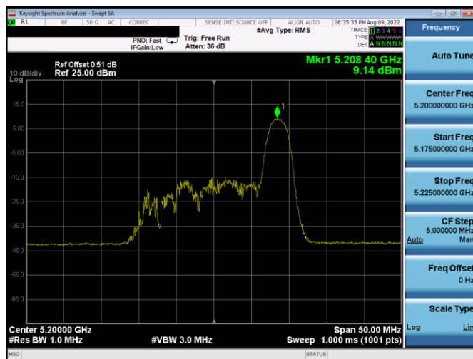
Plot 7-186. PSD Antenna WF4a (20MHz BW 11ax Index 8 - RU26 - Ch.40)
