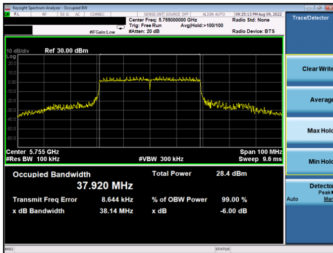
Plot 7-108. 6dB BW & 99% OBW Antenna WF4a (40MHz BW 11ax – RU484 – Ch.151)
