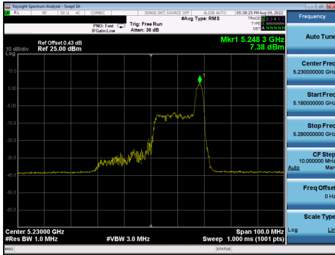
Plot 7-119. PSD Antenna WF5b (40MHz BW 11ax Index 17 – RU26 – Ch.46)
