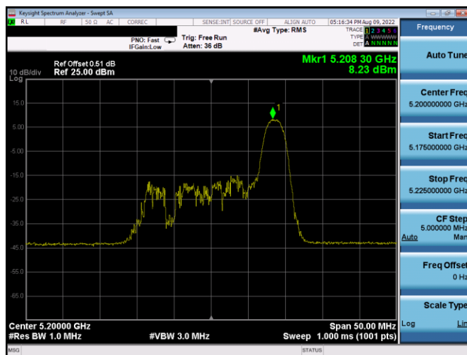
Plot 7-115. PSD Antenna WF5b (20MHz BW 11ax Index 8 - RU26 - Ch.40)
