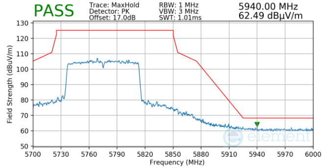
Plot 7-1196. Antenna 4a (Pk, Ch.155, 802.11ac, MCS9)
