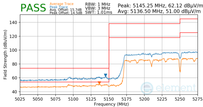
Plot 7-1219. Antenna 4a (Pk & Avg, Ch.50, 802.11ac, MCS4)
