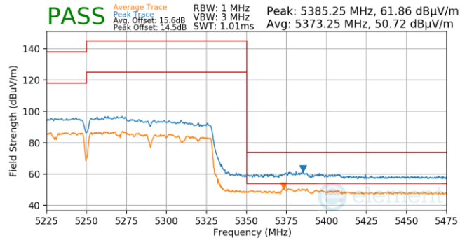
Plot 7-1222. Antenna 4a (Pk & Avg, Ch.50, 802.11ac, MCS4)
