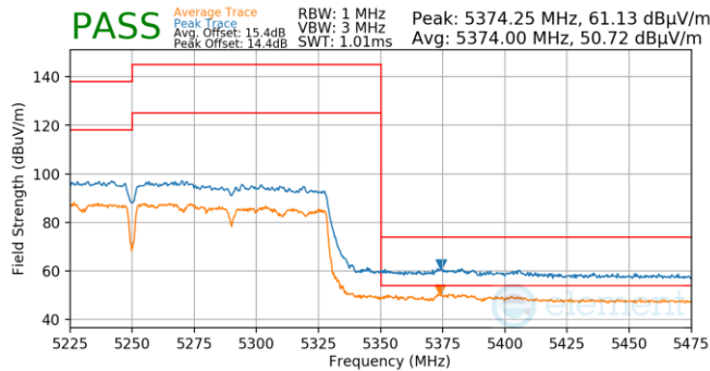
Plot 7-1221. Antenna 4a (Pk & Avg, Ch.50, 802.11ac, MCS2)
