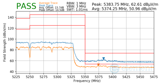
Plot 7-1223. Antenna 4a (Pk & Avg, Ch.50, 802.11ac, MCS9)
