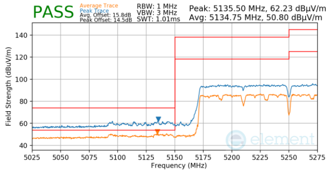
Plot 7-1220. Antenna 4a (Pk & Avg, Ch.50, 802.11ac, MCS9)
