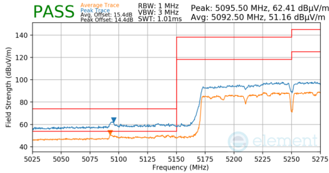
Plot 7-1218. Antenna 4a (Pk & Avg, Ch.50, 802.11ac, MCS2)
