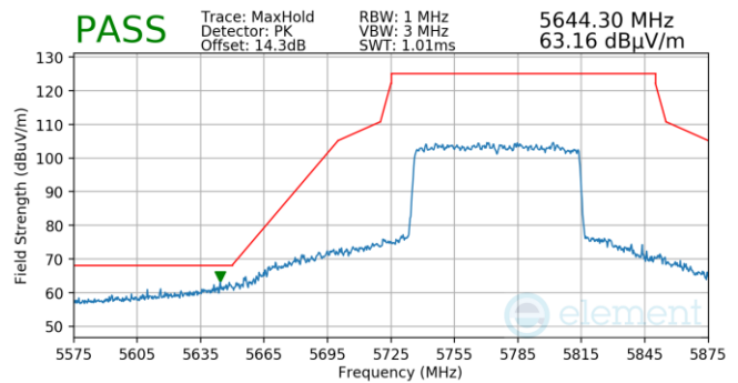
Plot 7-1214. Antenna 4a (Pk, Ch.155, 802.11ax(SU), MCS11)
