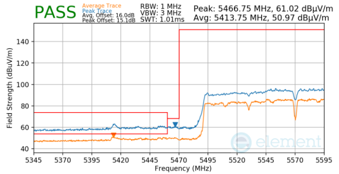
Plot 7-1224. (FCC Only) Antenna 4a (Pk & Avg, Ch.114, 802.11n, MCS2)
