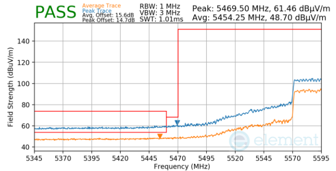
Plot 7-1207. (FCC Only) Antenna 4a (Pk & Avg, Ch.122, 802.11ax(SU), MCS3)
