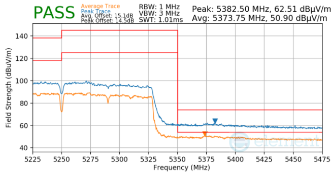
Plot 7-861. Antenna 5b (Pk & Avg, Ch.50, 802.11ac, MCS2)
