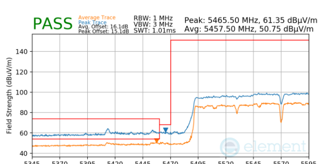
Plot 7-865. (FCC Only) Antenna 5b (Pk & Avg, Ch.114, 802.11n, MCS4)
