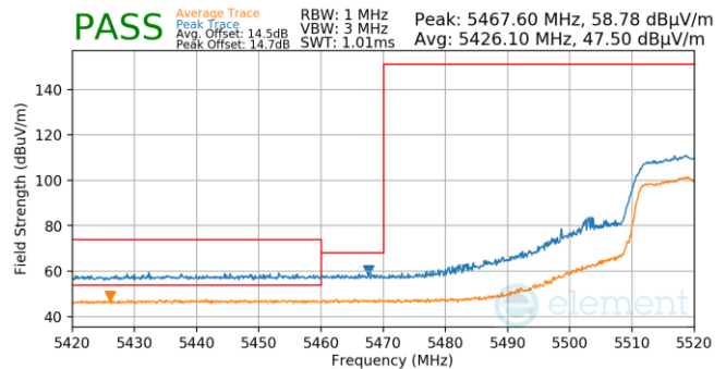
Plot 7-890. Antenna 4a (Pk & Avg, Ch.104, 802.11n, MCS4)
