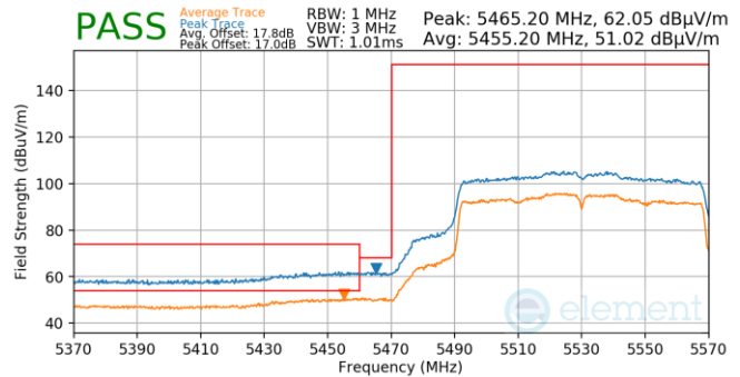
Plot 7-822. Antenna 5b (Pk & Avg, Ch.106, 802.11ac, MCS2)
