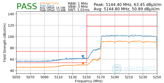
Plot 7-838. Antenna 5b (Pk & Avg, Ch.42, 802.11ax(SU), MCS4)
