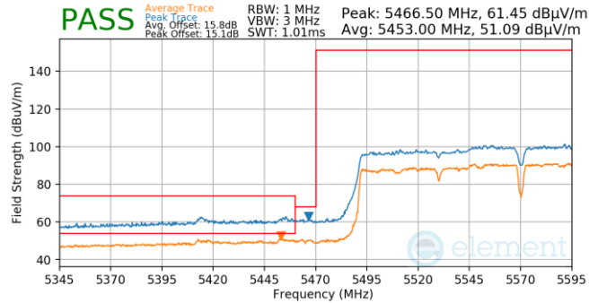
Plot 7-864. (FCC Only) Antenna 5b (Pk & Avg, Ch.114, 802.11n, MCS2)
