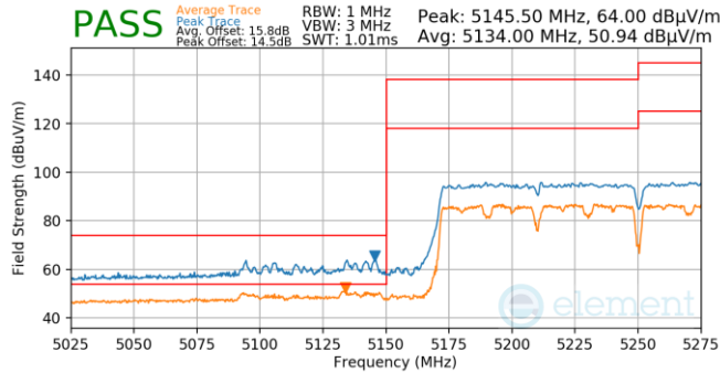
Plot 7-860. Antenna 5b (Pk & Avg, Ch.50, 802.11ac, MCS9)
