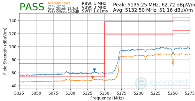
Plot 7-858. Antenna 5b (Pk & Avg, Ch.50, 802.11ac, MCS2)
