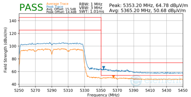
Plot 7-821. Antenna 5b (Pk & Avg, Ch.58, 802.11ac, MCS9)
