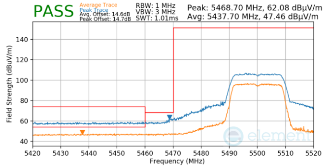
Plot 7-889. Antenna 4a (Pk & Avg, Ch.100, 802.11n, MCS7)
