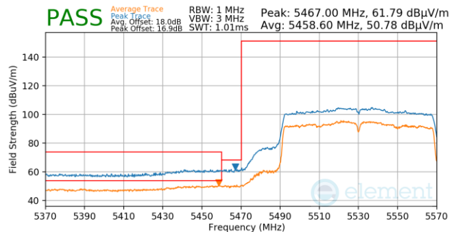
Plot 7-823. Antenna 5b (Pk & Avg, Ch.106, 802.11ac, MCS4)
