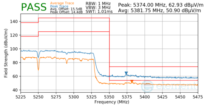
Plot 7-862. Antenna 5b (Pk & Avg, Ch.50, 802.11ac, MCS4)
