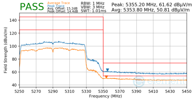
Plot 7-820. Antenna 5b (Pk & Avg, Ch.58, 802.11ac, MCS4)
