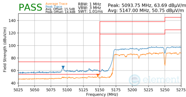
Plot 7-859. Antenna 5b (Pk & Avg, Ch.50, 802.11ac, MCS4)
