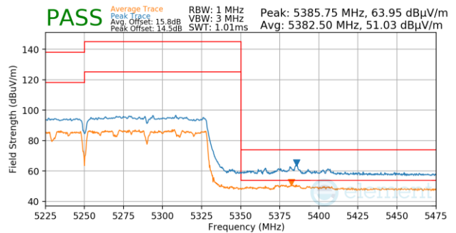
Plot 7-863. Antenna 5b (Pk & Avg, Ch.50, 802.11ac, MCS9)
