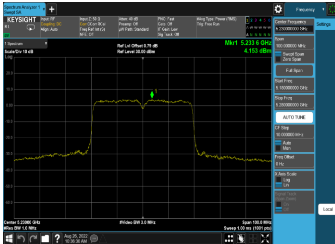
Plot 7-591. ISED PSD SDM Antenna 5b (40MHz BW 11ax(SU) – Ch.46, MCS11)
