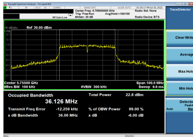
Plot 7-159. 6dB BW & 99% OBW Antenna 4a (40MHz BW 802.11n – Ch. 151, MCS4)
