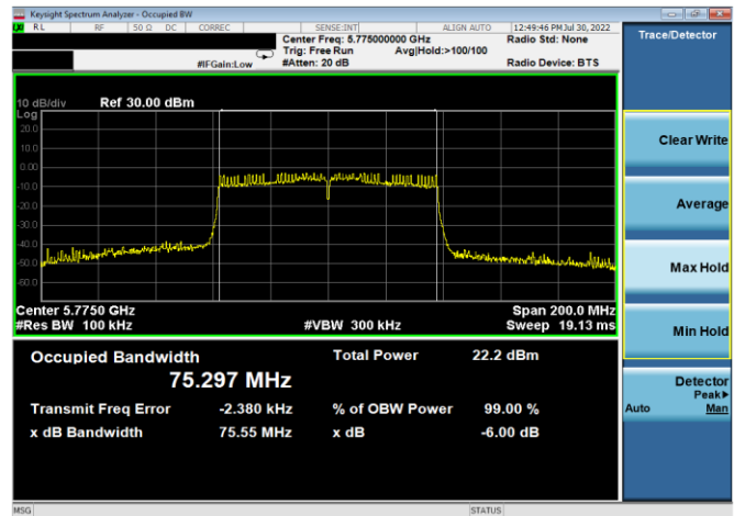
Plot 7-155. 6dB BW & 99% OBW Antenna 4a (80MHz BW 802.11ac – Ch. 155, MCS2)
