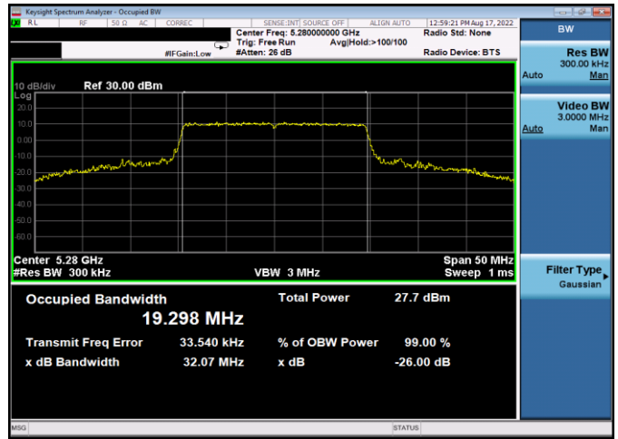
Plot 7-120. 26dB BW & 99% OBW Antenna 4a (20MHz BW 802.11ax(SU) – Ch. 56, MCS11)
