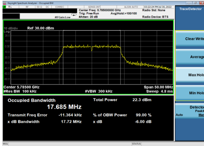
Plot 7-163. 6dB BW & 99% OBW Antenna 4a (20MHz BW 802.11n – Ch. 157, MCS7)
