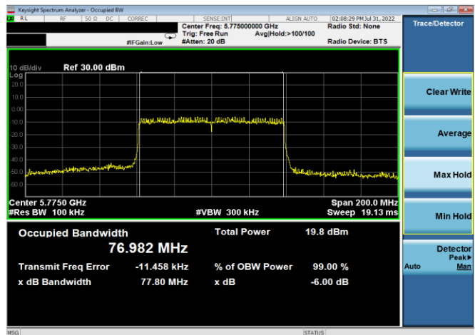
Plot 7-162. 6dB BW & 99% OBW Antenna 4a (80MHz BW 802.11ax(SU) – Ch. 155, MCS4)
