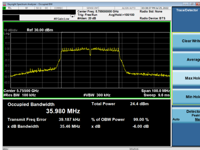
Plot 7-135. 6dB BW & 99% OBW Antenna 5b (40MHz BW 802.11n – Ch. 151, MCS2)
