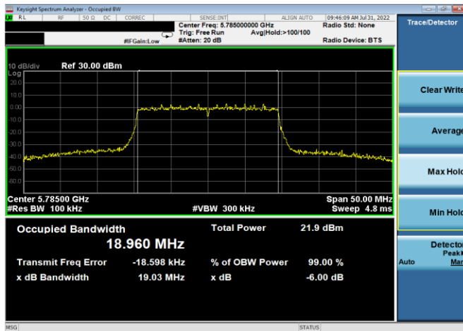
Plot 7-152. 6dB BW & 99% OBW Antenna 4a (20MHz BW 802.11ax(SU) – Ch. 157, MCS2)
