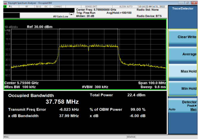
Plot 7-154. 6dB BW & 99% OBW Antenna 4a (40MHz BW 802.11ax(SU) – Ch. 151, MCS2)
