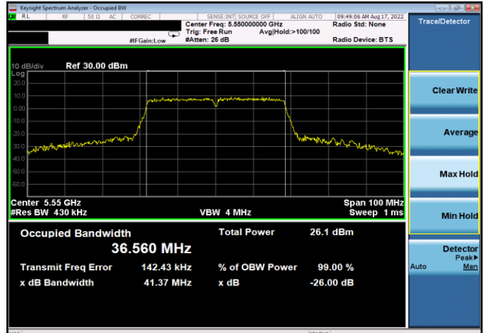
Plot 7-127. 26dB BW & 99% OBW Antenna 4a (40MHz BW 802.11n – Ch. 110, MCS9)
