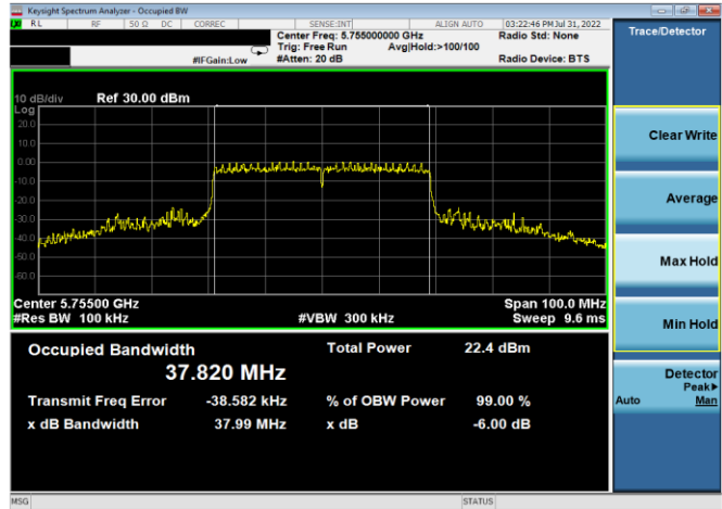
Plot 7-166. 6dB BW & 99% OBW Antenna 4a (40MHz BW 802.11ax(SU) – Ch. 151, MCS11)
