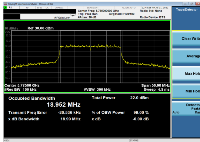
Plot 7-158. 6dB BW & 99% OBW Antenna 4a (20MHz BW 802.11ax(SU) – Ch. 157, MCS4)
