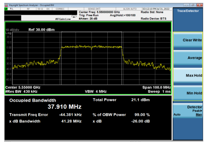
Plot 7-128. 26dB BW & 99% OBW Antenna 4a (40MHz BW 802.11ax(SU) – Ch. 110, MCS11)
