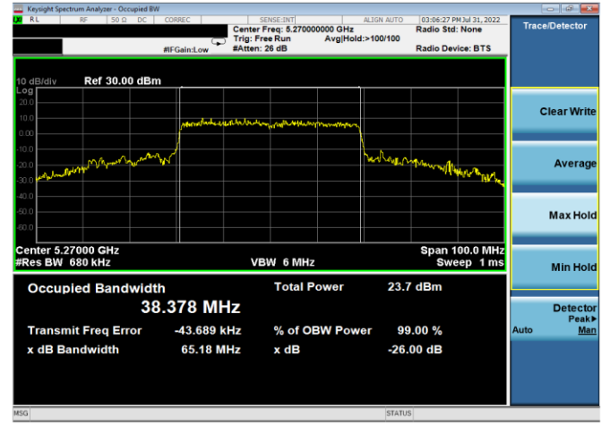
Plot 7-122. 26dB BW & 99% OBW Antenna 4a (40MHz BW 802.11ax(SU) – Ch. 54, MCS11)
