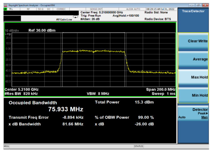
Plot 7-115. 26dB BW & 99% OBW Antenna 4a (80MHz BW 802.11ac – Ch. 42, MC9)
