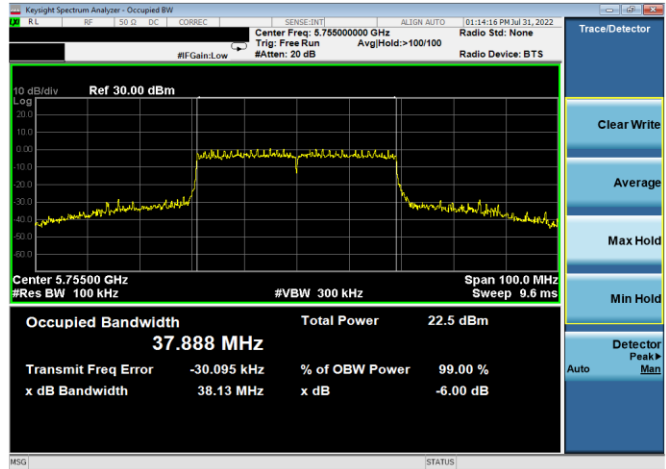
Plot 7-160. 6dB BW & 99% OBW Antenna 4a (40MHz BW 802.11ax (SU) – Ch. 151, MCS4)
