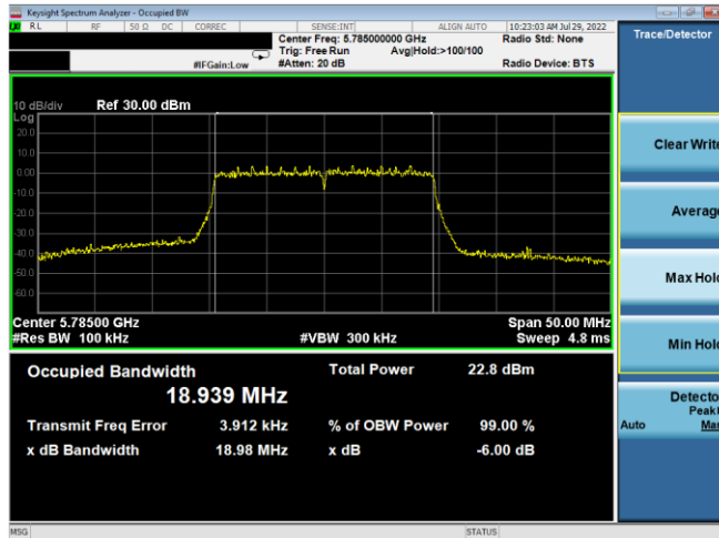
Plot 7-134. 6dB BW & 99% OBW Antenna 5b (20MHz BW 802.11ax(SU) – Ch. 157, MCS2)
