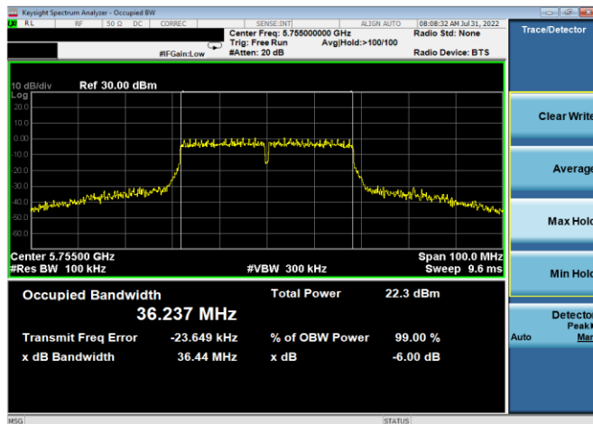
Plot 7-165. 6dB BW & 99% OBW Antenna 4a (40MHz BW 802.11n – Ch. 151, MCS9)
