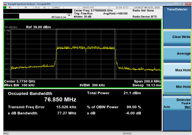
Plot 7-156. 6dB BW & 99% OBW Antenna 4a (80MHz BW 802.11ax(SU) – Ch. 155, MCS2)
