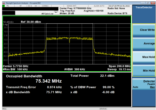
Plot 7-161. 6dB BW & 99% OBW Antenna 4a (80MHz BW 802.11ac – Ch. 155, MCS4)
