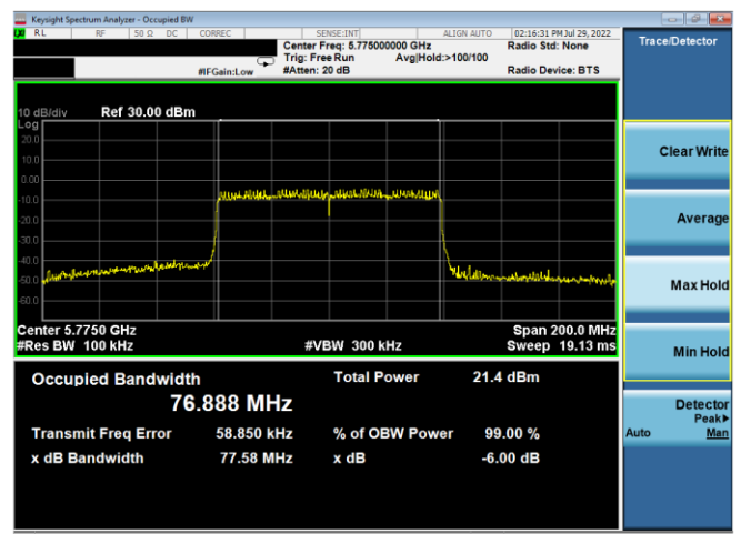
Plot 7-144. 6dB BW & 99% OBW Antenna 5b (80MHz BW 802.11ax(SU) – Ch. 155, MCS4)
