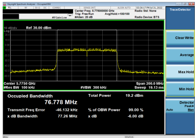
Plot 7-168. 6dB BW & 99% OBW Antenna 4a (80MHz BW 802.11ax(SU) – Ch. 155, MCS11)
