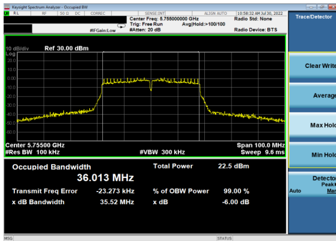
Plot 7-153. 6dB BW & 99% OBW Antenna 4a (40MHz BW 802.11n – Ch. 151, MCS2)
