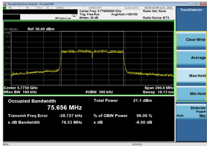
Plot 7-167. 6dB BW & 99% OBW Antenna 4a (80MHz BW 802.11ac – Ch. 155, MCS9)
