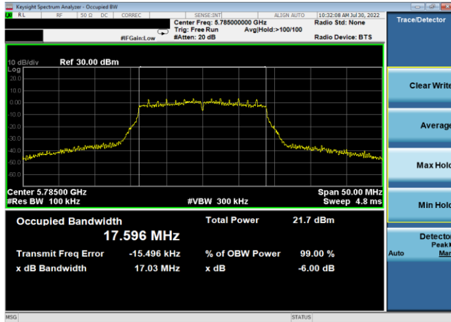
Plot 7-151. 6dB BW & 99% OBW Antenna 4a (20MHz BW 802.11n – Ch. 157, MCS2)
