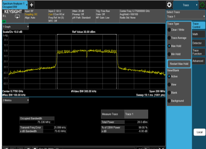
Plot 7-143. 6dB BW & 99% OBW Antenna 5b (80MHz BW 802.11ac – Ch. 155, MCS4)
