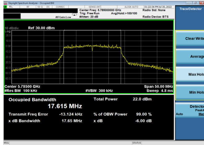
Plot 7-157. 6dB BW & 99% OBW Antenna 4a (20MHz BW 802.11n – Ch. 157, MCS4)
