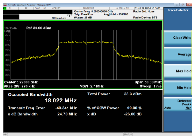
Plot 7-119. 26dB BW & 99% OBW Antenna 4a (20MHz BW 802.11n – Ch. 56, MCS7)
