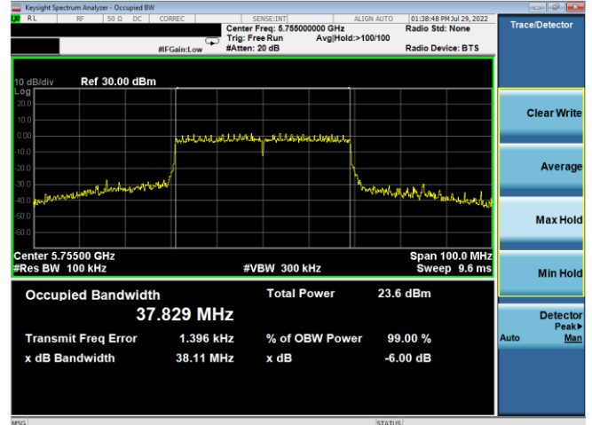
Plot 7-142. 6dB BW & 99% OBW Antenna 5b (40MHz BW 802.11ax(SU) – Ch. 151, MCS4)
