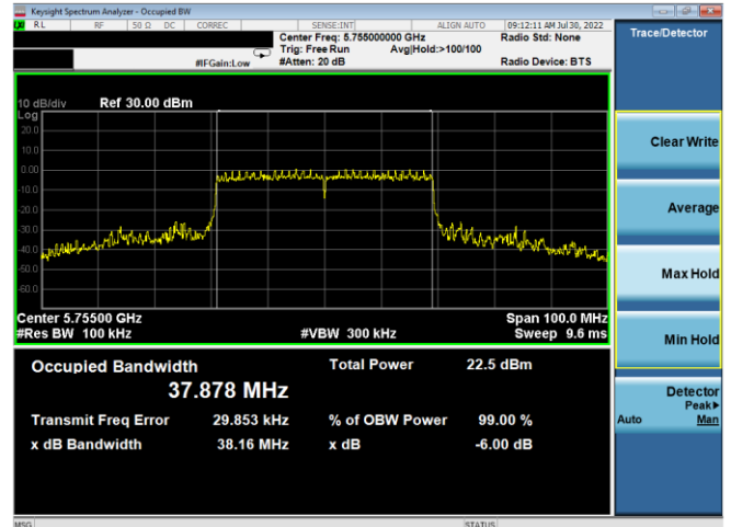
Plot 7-148. 6dB BW & 99% OBW Antenna 5b (40MHz BW 802.11ax(SU) – Ch. 151, MCS11)
