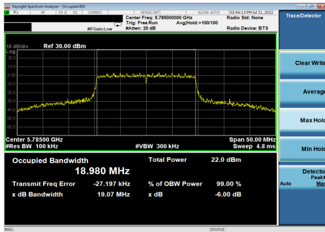
Plot 7-164. 6dB BW & 99% OBW Antenna 4a (20MHz BW 802.11ax(SU) – Ch. 157, MCS11)
