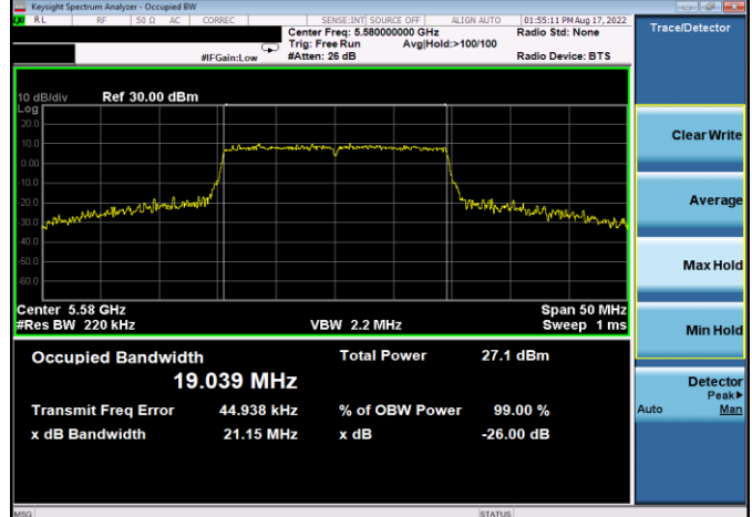
Plot 7-126. 26dB BW & 99% OBW Antenna 4a (20MHz BW 802.11ax(SU) – Ch. 116, MCS11)
