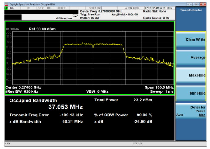
Plot 7-121. 26dB BW & 99% OBW Antenna 4a (40MHz BW 802.11n – Ch. 54, MCS9)
