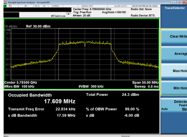
Plot 7-139. 6dB BW & 99% OBW Antenna 5b (20MHz BW 802.11n – Ch. 157, MCS4)
