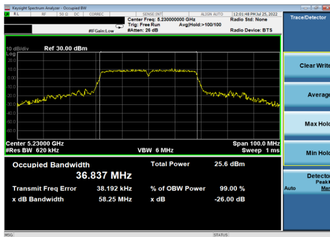
Plot 7-47. 26dB BW & 99% OBW Antenna 5b (40MHz BW 802.11n – Ch. 46, MCS7)
