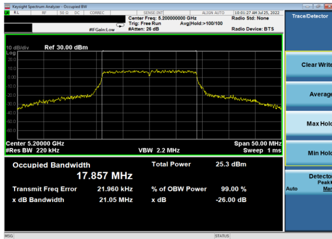
Plot 7-45. 26dB BW & 99% OBW Antenna 5b (20MHz BW 802.11n – Ch. 40, MCS7)
