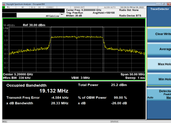
Plot 7-46. 26dB BW & 99% OBW Antenna 5b (20MHz BW 802.11ax(SU) – Ch. 40, MCS11)
