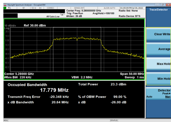
Plot 7-97. 26dB BW & 99% OBW Antenna 4a (20MHz BW 802.11n – Ch. 56, MCS4)
