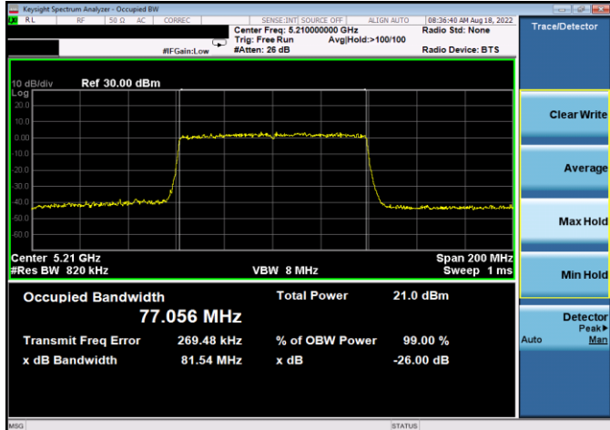
Plot 7-50. 26dB BW & 99% OBW Antenna 5b (80MHz BW 802.11ax(SU) – Ch. 42, MCS11)
