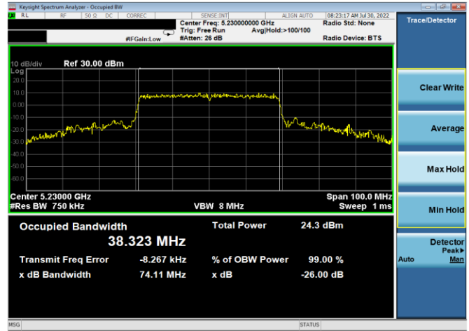
Plot 7-48. 26dB BW & 99% OBW Antenna 5b (40MHz BW 802.11ax(SU) – Ch. 46, MCS11)
