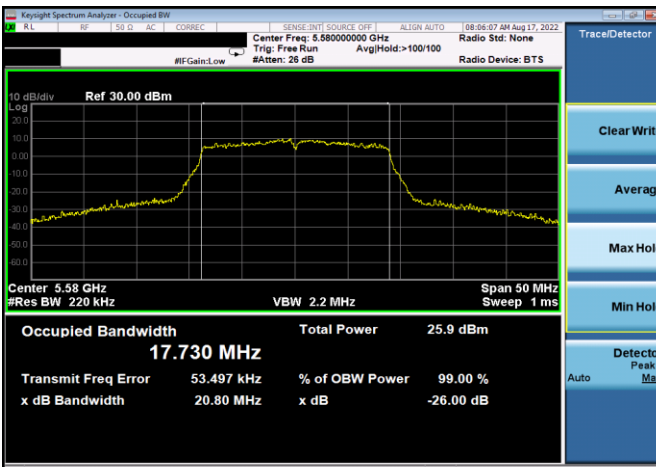
Plot 7-103. 26dB BW & 99% OBW Antenna 4a (20MHz BW 802.11n – Ch. 116, MCS4)
