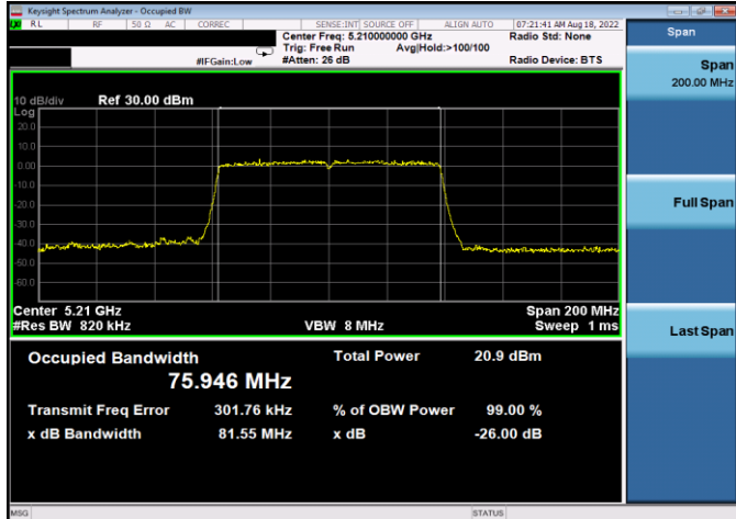
Plot 7-49. 26dB BW & 99% OBW Antenna 5b (80MHz BW 802.11ac – Ch. 42, MCS9)
