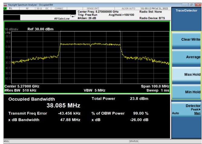
Plot 7-100. 26dB BW & 99% OBW Antenna 4a (40MHz BW 802.11ax(SU) – Ch. 54, MCS4)
