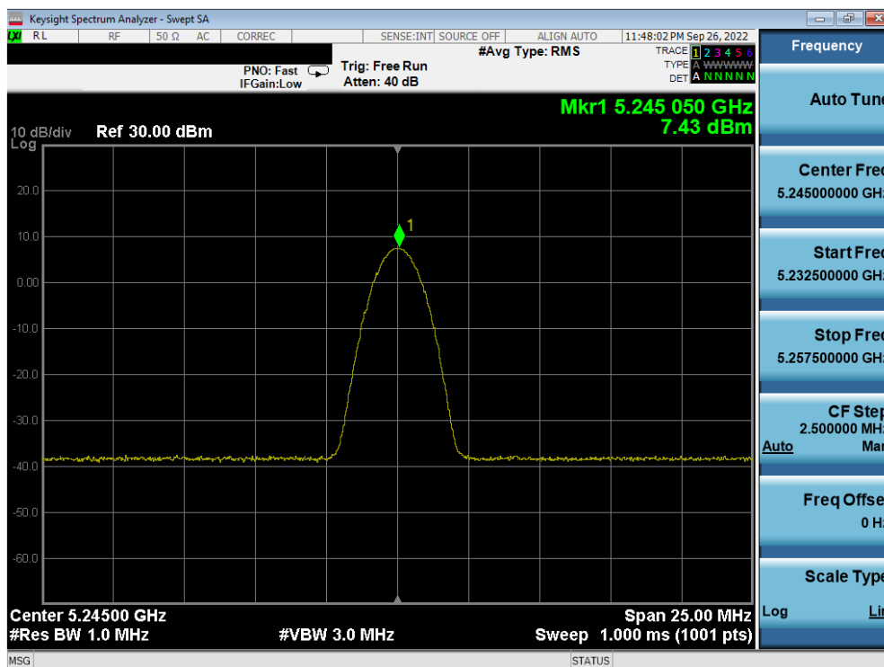
Plot 7-42. PSD TxBF Antenna 4a (BDR GFSK, ePA - 5245MHz)
