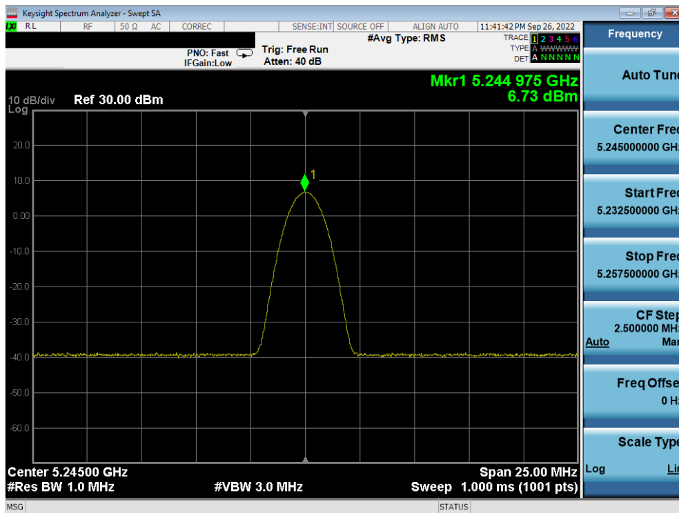
Plot 7-41. PSD TxBF Antenna 5b (BDR GFSK, ePA - 5245MHz)
