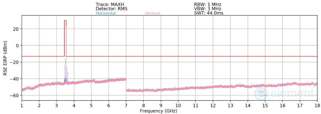
Plot 7-283. Antenna 3 Radiated Spurious Plot 1GHz – 18GHz (NR Band n77 DoD Band)
