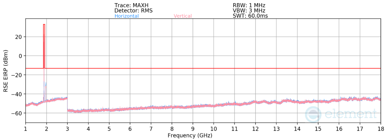
Plot 7-2. Antenna 4b Radiated Spurious Emission above 1GHz (LTE Band 2)
