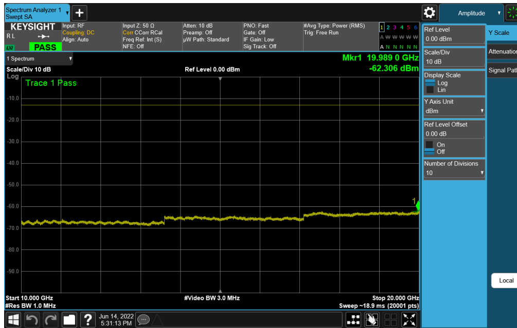
Plot 7-72. Conducted Spurious Plot (NR Band n25/n2 - 40.0MHz - RB Size 1, RB Offset 0 - Low Channel)
