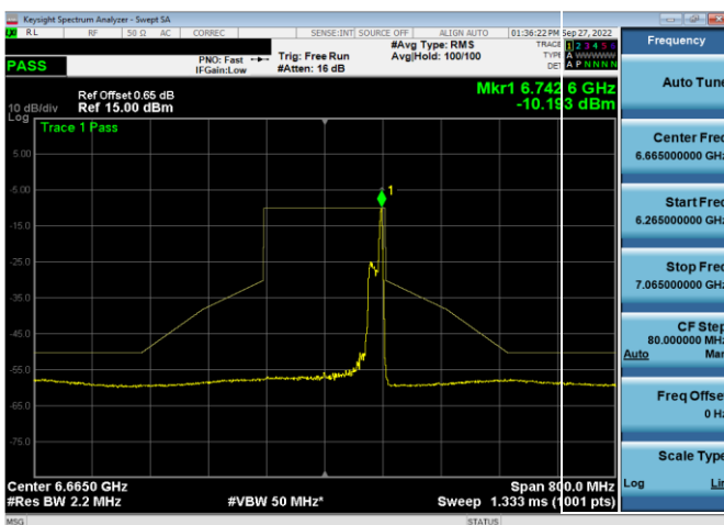
Plot 7-604. In-Band Emission Plot SDM Antenna WF5t (160MHz 802.11ax RU26 (UNII Band 7) – Ch. 143)
