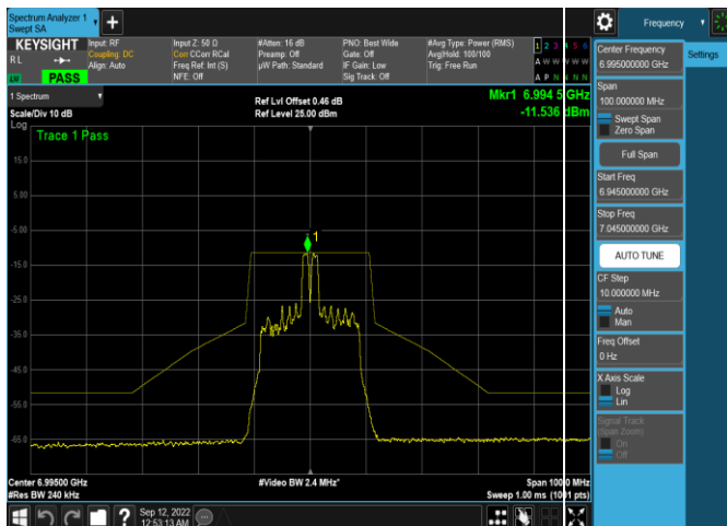
Plot 7-610. In-Band Emission Plot SDM Antenna WF5b (20MHz 802.11ax RU26 (UNII Band 8) – Ch. 209)
