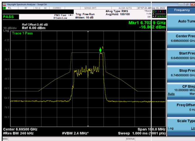
Plot 7-580. In-Band Emission Plot SDM Antenna WF5t (20MHz 802.11ax RU26 (UNII Band 7) – Ch. 149)
