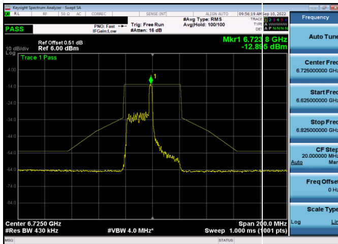
Plot 7-586. In-Band Emission Plot SDM Antenna WF5t (40MHz 802.11ax RU26 (UNII Band 7) – Ch. 155)
