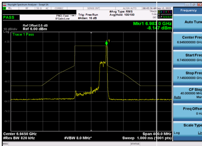
Plot 7-628. In-Band Emission Plot SDM Antenna WF5b (80MHz 802.11ax RU26 (UNII Band 8) – Ch. 199)
