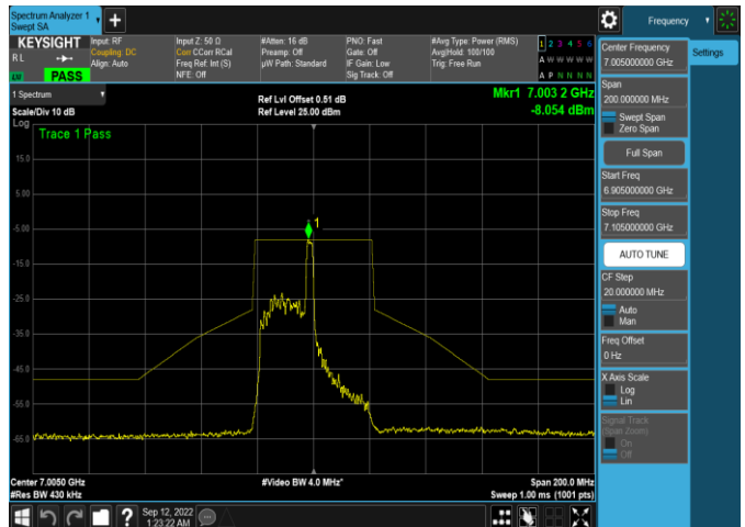
Plot 7-618. In-Band Emission Plot SDM Antenna WF5b (40MHz 802.11ax RU26 (UNII Band 8) - Ch. 211)
