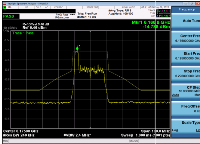
Plot 7-512. In-Band Emission Plot SDM Antenna WF5t (20MHz 802.11ax RU26 (UNII Band 5) – Ch. 45)
