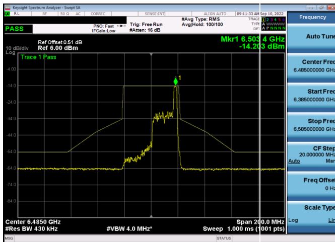
Plot 7-556. In-Band Emission Plot SDM Antenna WF5t (40MHz 802.11ax RU26 (UNII Band 6) – Ch. 107)
