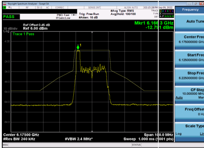
Plot 7-384. In-Band Emission Plot Antenna WF5t (20MHz 802.11ax RU26 (UNII Band 5) – Ch. 45)
