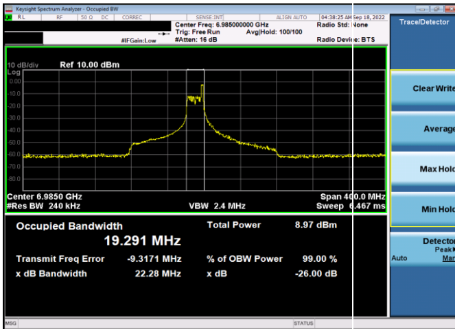
Plot 7-62. 26dB & 99% Bandwidth Plot Antenna WF5t (160MHz 802.11ax RU26 (UNII Band 8) – Ch. 207)
