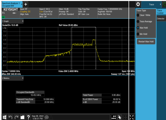
Plot 7-55. 26dB & 99% Bandwidth Plot Antenna WF5t (40MHz 802.11ax RU26 (UNII Band 8) - Ch. 211)
