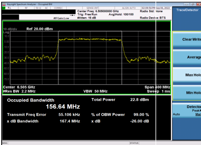
Plot 7-32. 26dB & 99% Bandwidth Plot Antenna WF5t (160MHz 802.11ax RU484 (UNII Band 6) – Ch. 111)
