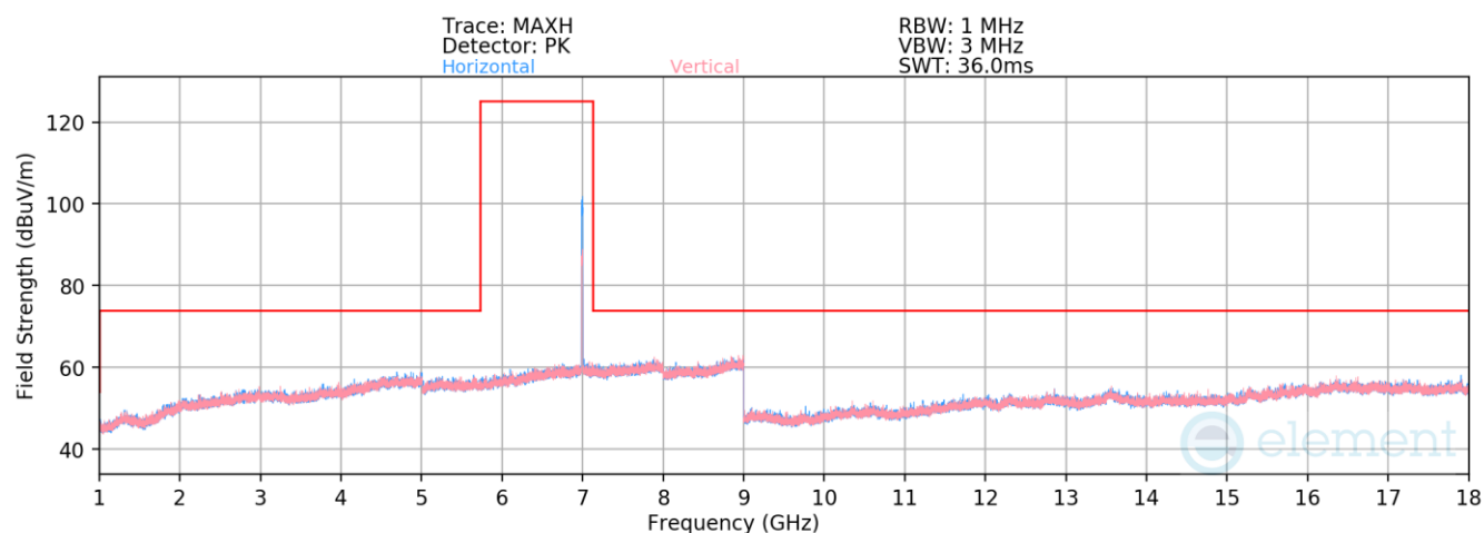
Plot 7-595. Radiated Spurious Emissions above 1GHz Antenna WF5t (802.11ax – Ch. 209, MCS2)
