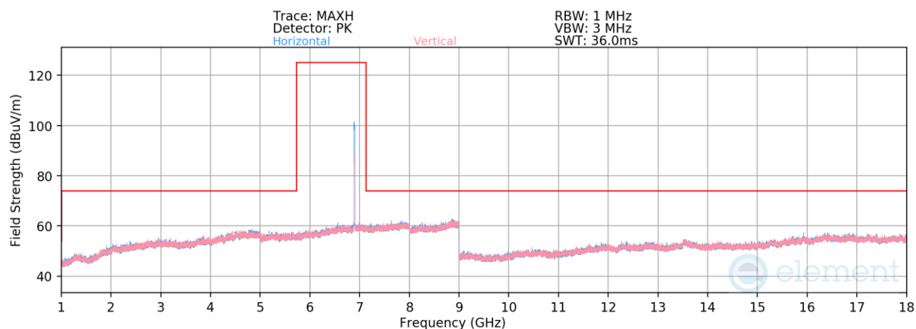
Plot 7-594. Radiated Spurious Emissions above 1GHz Antenna WF5t (802.11ax – Ch. 189, MCS2)
