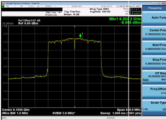
Plot 7-280. Power Spectral Density Plot SDM Antenna WF5b (160MHz 802.11ax (UNII Band 5) – Ch. 47, MCS4)
