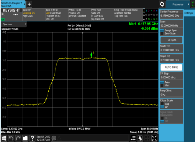
Plot 7-217. Power Spectral Density Plot Antenna WF5b (20MHz 802.11a (UNII Band 5) – Ch. 45, MCS11)
