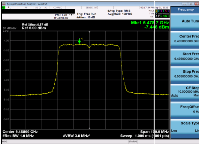
Plot 7-224. Power Spectral Density Plot Antenna WF5b (40MHz 802.11ax (UNII Band 6) – Ch. 107, MCS11)
