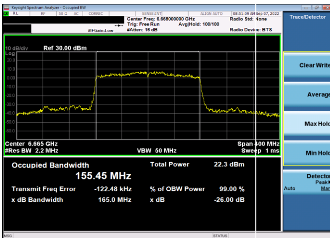
Plot 7-95. 26dB & 99% Bandwidth Plot Antenna WF5b (160MHz) 802.11ax (UNII Band 7) – Ch. 143, MCS4)
