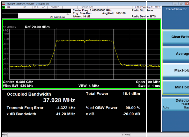
Plot 7-88. 26dB & 99% Bandwidth Plot Antenna WF5b (40MHz 802.11ax (UNII Band 6) – Ch. 107, MCS4)
