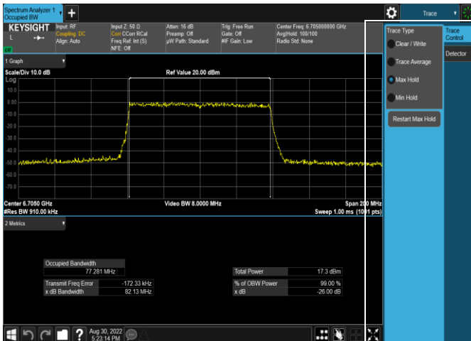
Plot 7-94. 26dB & 99% Bandwidth Plot Antenna WF5b (80MHz) 802.11ax (UNII Band 7) – Ch. 151, MCS4)
