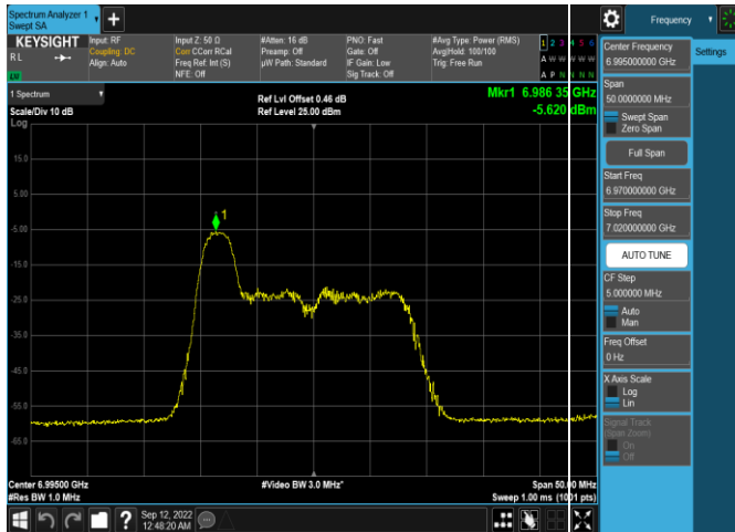
Plot 7-353. Power Spectral Density Plot SDM Antenna WF5b (20MHz 802.11ax RU26 (UNII Band 8) – Ch. 209)
