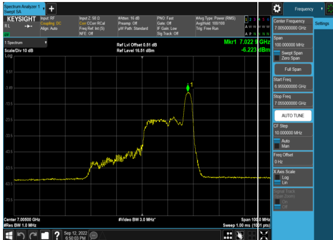
Plot 7-183. Power Spectral Density Plot Antenna WF5t (40MHz 802.11ax RU26 (UNII Band 8) – Ch. 211)
