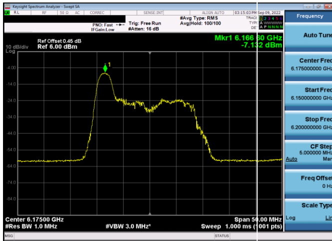
Plot 7-129. Power Spectral Density Plot Antenna WF5t (20MHz 802.11ax RU26 (UNII Band 5) – Ch. 45)
