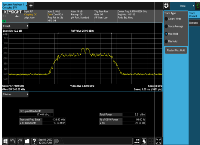
Plot 7-2. 26dB & 99% Bandwidth Plot Antenna WF5t (20MHz 802.11ax RU26 (UNII Band 5) – Ch. 45)
