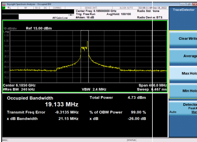
Plot 7-14. 26dB & 99% Bandwidth Plot Antenna WF5t (160MHz 802.11ax RU26 (UNII Band 5) - Ch. 47)
