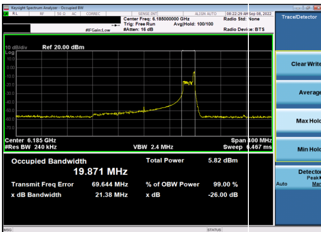
Plot 7-15. 26dB & 99% Bandwidth Plot Antenna WF5t (160MHz 802.11ax RU26 (UNII Band 5) - Ch. 47)
