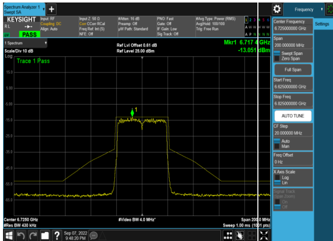
Plot 7-540. In-Band Emission Plot SDM Antenna WF5b (40MHz 802.11ax (UNII Band 7) – Ch. 155, MCS11)
