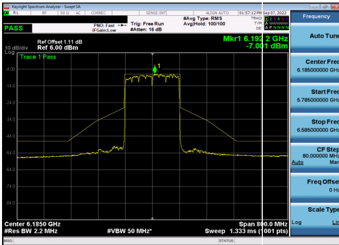
Plot 7-528. In-Band Emission Plot SDM Antenna WF5b (160MHz 802.11ax (UNII Band 5) – Ch. 47, MCS11)
